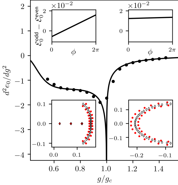
FIG. 2. Second derivative of the ground-state energy density e_0 with respect to coupling for a mean-field solution [20] with L = 2000 (solid line), and the exact solution at L = 128 , both at quarter filling ( \rho = 1/2 ). Lower insets: the variables e_\alpha (diamonds) and \omega_\beta (dots) are plotted with their imaginary parts on the y -axis and their real parts on the x -axis at g/g_c = 0.9 (left) and 1.1 (right). An animation of these spectral parameters as a function of g is included in the supplemental material [20]. Upper insets: energy difference between odd and even sectors is plotted as a function of boundary condition \phi for a quarter-filled system with 32 fermions at g/g_c = 0.7 (left) and 1.75 (right).
