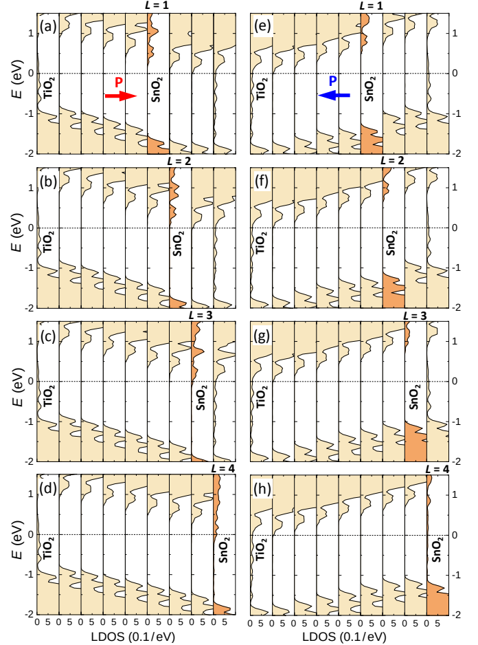
FIG. 2. Local densities of states (LDOS) as a function of energy E on each BO_2 (B = Ti, Sn) atomic layer within a composite BaTi(Sn)O_3 barrier for four FTJ structures with SnO_2 layer at L = 1 (a, e), L = 2 (b, f), L = 3 (c, g), and L = 4 (d, h) for polarization pointing right (a-d) and left (e-h). Horizontal dashed lines indicate the Fermi energy.
