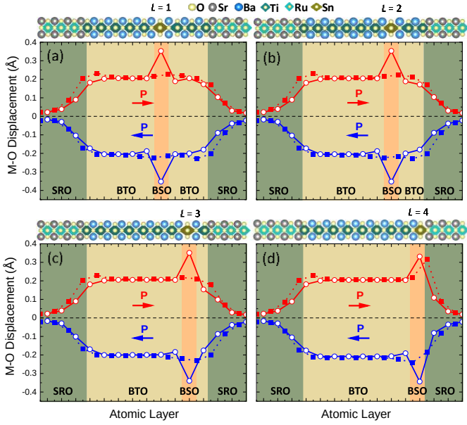
FIG. 1. Calculated relative polar displacement between cation (M) and anion (O) on each AO (squares, A = Ba or Sr) and BO_2 (circles, B = Ti, Sn, or Ru) layer across SrRuO_3/BaTi(Sn)O_3 supercells (top panels) with a SnO_2 monolayer placed at four different positions numbered by L = 1 (a), L = 2 (b), L = 3 (c), and L = 4 (d) as indicated by orange vertical bars. Positive (negative) values of the displacement shown in red (blue) correspond to polarization pointing to the right (left). Open (solid) symbols denote Ti-O, Sn-O, and Ru-O (Ba-O and Sr-O) displacements.
