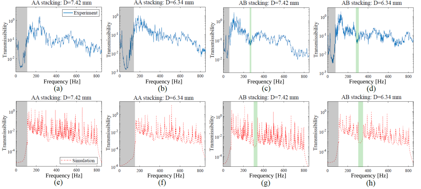
FIG. 5. Experimental results. (a-d) Transmissibility vs. frequency plots obtained from vibrometry data for AA stacking (a-b) and AB stacking (c-d), for different inter-layer distances. The plots reveal a foundation bandgap, whose width depends on the inter-layer distance and can be tuned by twist. For sufficiently strong inter-layer interactions, a second bandgap associated with symmetry breaking is switched on by twisting the layers from AA to AB stacking. (e-h) Transmissibility plots obtained from full-scale simulations for same stacking conditions and inter-layer distances, correlating well with the experimental results.
