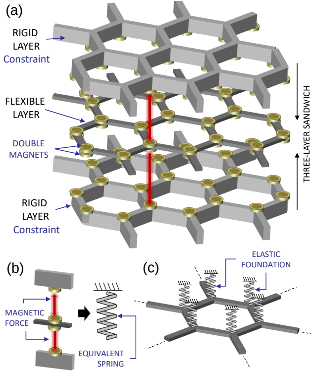
FIG. 1. Magneto-mechanical multi-layer analog of graphene bilayer. (a) Three-layer sandwich stacking. (b) Equivalent spring model for the magnetic interactions (c) Inner layer modeled as single layer on elastic foundation.
