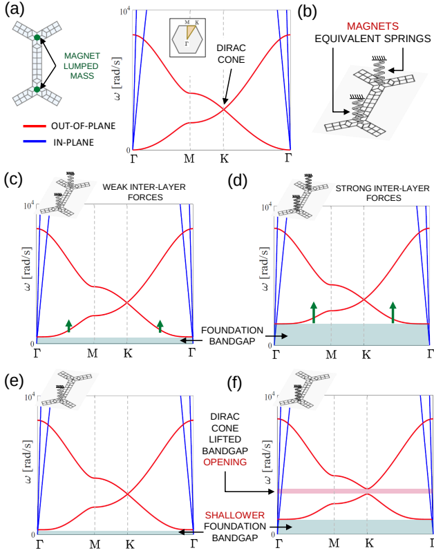
FIG. 3. (a) Evolution of band diagram upon changes in twist angle and inter-layer distance. (a) Baseline case of single layer: FEM model of unit cell; band diagram with in-plane (blue) and out-of-plane (red) modes, featuring Dirac cone at K point of the Brillouin zone. (b) Unit cell with elastic foundation (AA stacking case shown). (c) AA stacking with large inter-layer distance (weak magnetic forces), with up-shifting of the flexural mode and opening of a foundation bandgap. (d) AA stacking with smaller inter-layer distance (stronger magnetic forces), resulting in increase of the foundation bandgap width. (e) AB stacking with weak magnetic forces, resulting in reduction of the foundation bandgap width. (f) AB stacking with strong magnetic forces, resulting in increase in foundation bandgap width and opening of finite-frequency bandgap due to space inversion symmetry (SIS) breaking.
