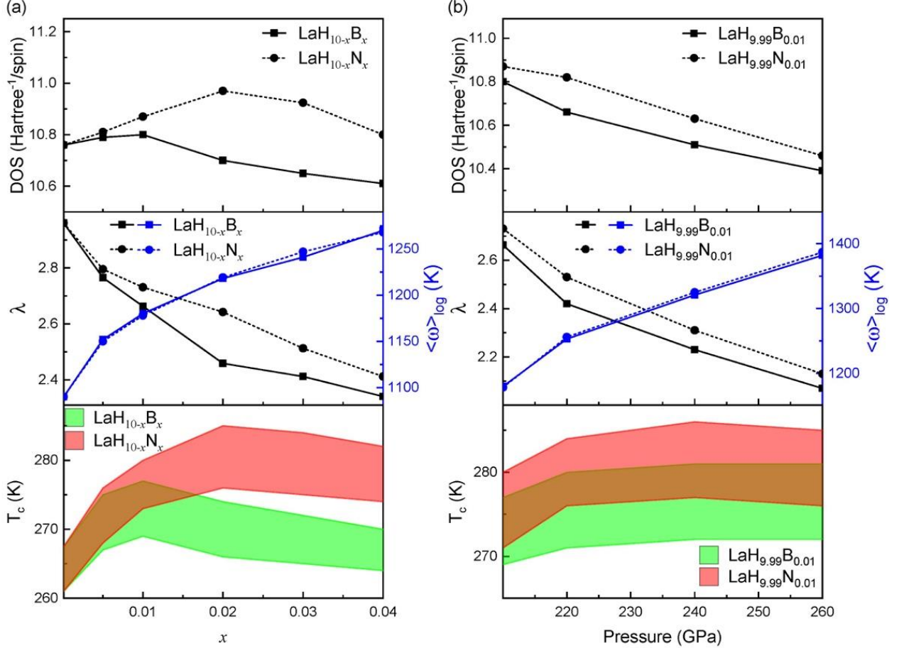
Fig. 3. (a) DOS, \lambda , \langle\omega\rangle_{\log} , and T_c of LaH 10-x B x and LaH 10-x N x with different doping levels at 210 GPa. (b) DOS, \lambda , \langle\omega\rangle_{\log} , and T_c of LaH 9.99 B 0.01 and LaH 9.99 N 0.01 at different pressures. For each T_c curve, the upper and lower bounds are obtained by choosing \mu^*=0.10 and 0.11 , respectively.
