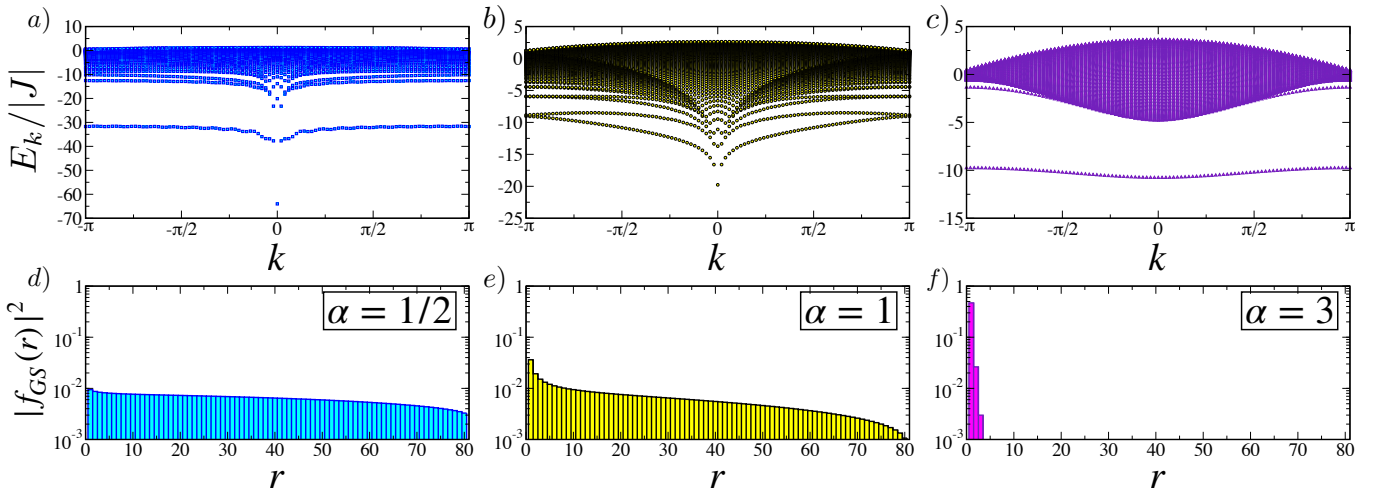
FIG. 1. Upper panels: Energy spectrum of the two-spin configuration \sum_{i=1}^L S_i^z = |L - 4|/2 , L = 100 , as a function of the momentum k \in [-\pi, \pi] for \alpha = 1/2 a), \alpha = 1 b) and \alpha = 3 c). Lower panels: density |f_{GS}(r)|^2 , i.e. the lowest energy eigenstate corresponding to k = 0 (see main text), for \alpha = 1/2 d), \alpha = 1 e), and \alpha = 3 f). Here we consider ferromagnetic couplings with \Delta/J = -5 and solve eq.(10) for p_{max} = 80 (half-maximum relative distance). For \alpha \leq 1 the relative wavefunction is non vanishing even at the edges. This feature persists even for larger values of \Delta .
