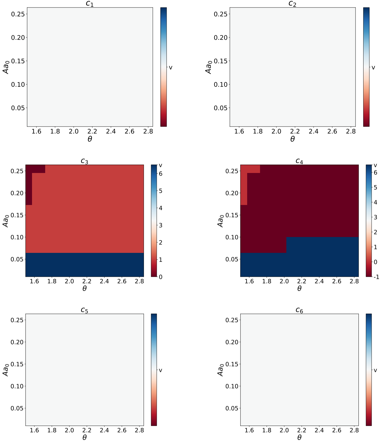
FIG. 15: (Color online) The Chern number maps for the central six bands in the TTG with AAA stacking and middle layer twisted. The letter "v" stands for the case when no gap opening has been observed.
