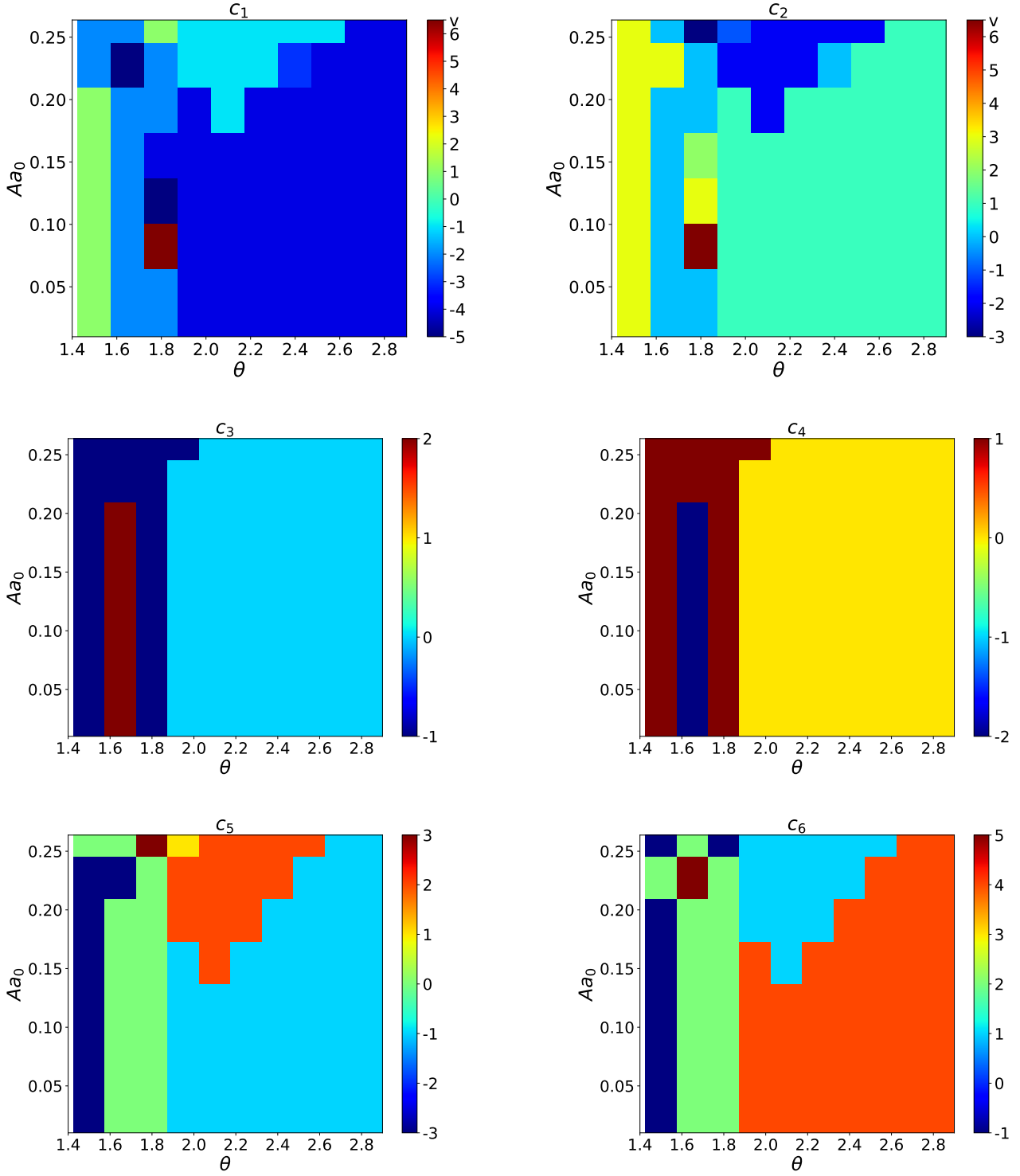
FIG. 14: (Color online) The Chern number variation for the six central bands in the TTG system with the AAA stacking and top layer. This is associated with Fig. 7 (a).
