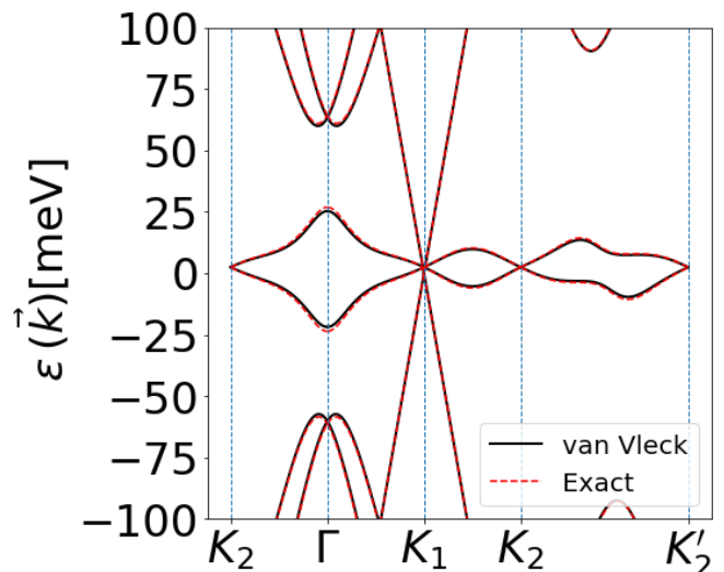
FIG. 13: Comparison of the band structure for TTG with ABA stacking and middle layer twisted driven by waveguide light with \theta = 1.3^\circ , Aa_0 = 0.8 , and \omega = 1.5\gamma . obtained via the quasi-energy operator Eq. 6 (dashed lines) versus the zeroth order van Vleck Hamiltonian H_0 (solid lines).
