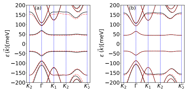
FIG. 5: (Color online) Comparison between the exact quasi-energies and the energies from the effective Hamiltonians for the band structure of the TTG with AAA stacking and middle layer twisted, driven by circularly polarized light \theta = 1.6^\circ , Aa_0 = 0.4 , and \omega = 3\gamma . (a) Van Vleck (solid lines) and exact quasi-energies compared (dashed lines) (b) Rotating frame (solid lines) versus the quasi-energies (dashed lines).
