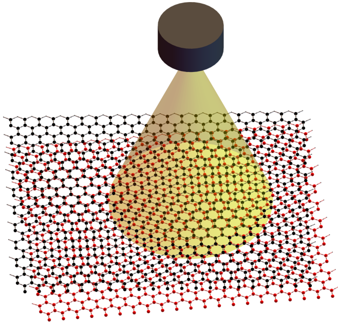
FIG. 3: Light source applied on TTG system with AAA middle layer twisted.
