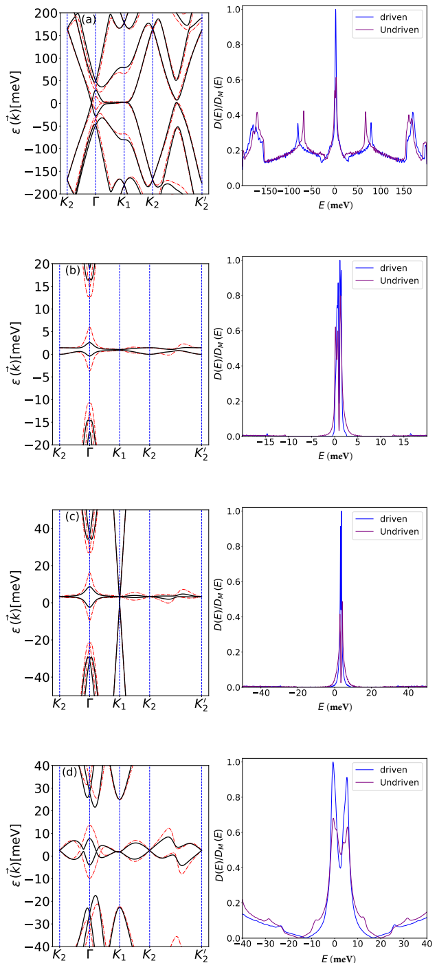
FIG. 11: (Color online) Left Column: Band structure of the TTG driven by waveguide light with Aa_0 = 0.3 . (a) The AAA stacking with TLT and (\theta, \omega) = (2.000^\circ, 2\gamma) , (b) the ABC configuration with TLT and (\theta, \omega) = (1.040^\circ, 2\gamma) , (c) AAA with MLT and parameters (\theta, \omega) = (1.450^\circ, 3\gamma) , and (d) the ABC stacking with MLT and (\theta, \omega) = (1.157^\circ, 2\gamma) . The solid lines are for the driven and the dash-dotted lines for the undriven case. Right Column: The density of states plots associated with the configurations on the left column rescaled by the maximum value D_M(E) of the driven case.
