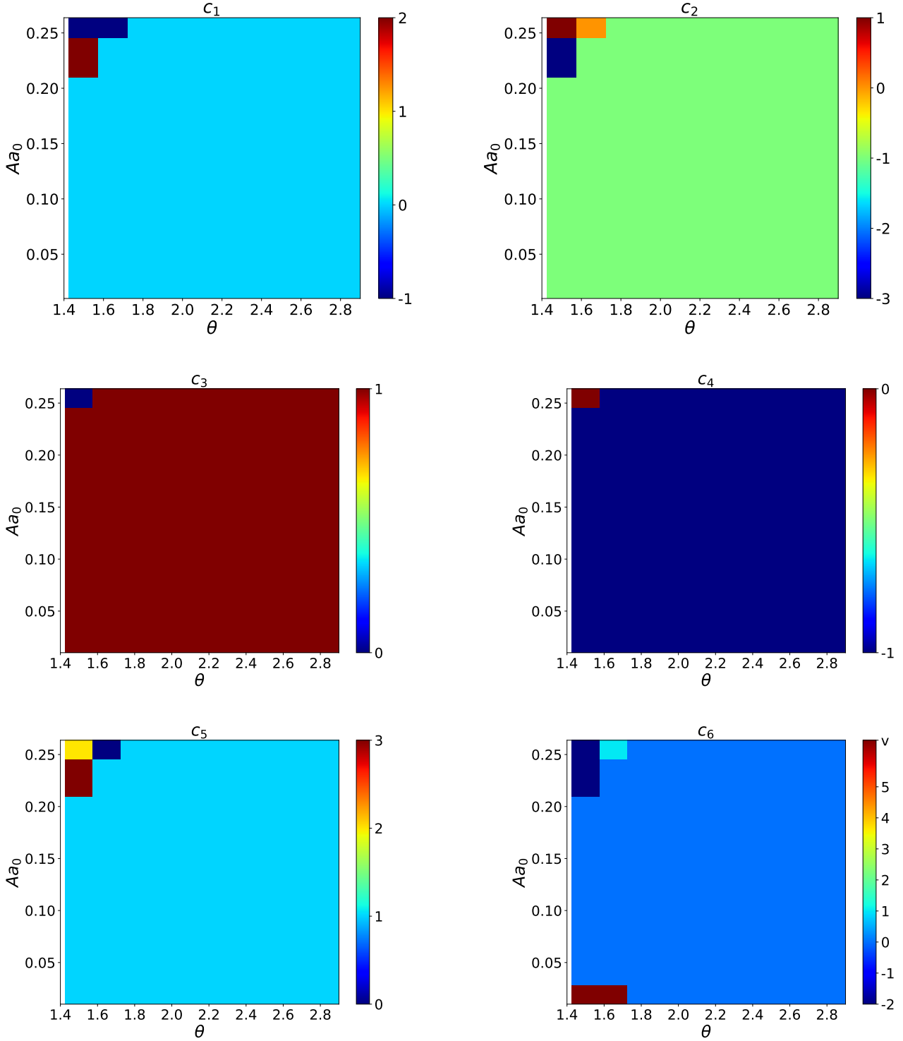
FIG. 16: (Color online) Variations of the Chern numbers for each of the six central bands c_1 \rightarrow c_6 for the case of ABC stacking and MLT. The letter v in the topological map of the sixth band ( c_6 ) corresponds to no gap opening??
