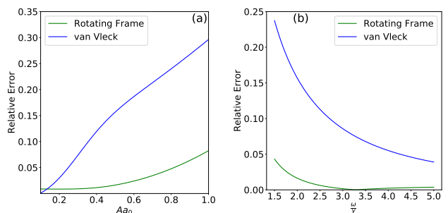
FIG. 6: (Color online) Plot of relative error for the gap at the K_1 symmetry point for the TTG system with AAA stacking and middle layer twisted driven by circularly polarized light (a) as function of Aa_0 , with \theta = 1.6^\circ , and \omega = 2\gamma , (b) and as a function of \omega/\gamma with Aa_0 = 0.5 .
