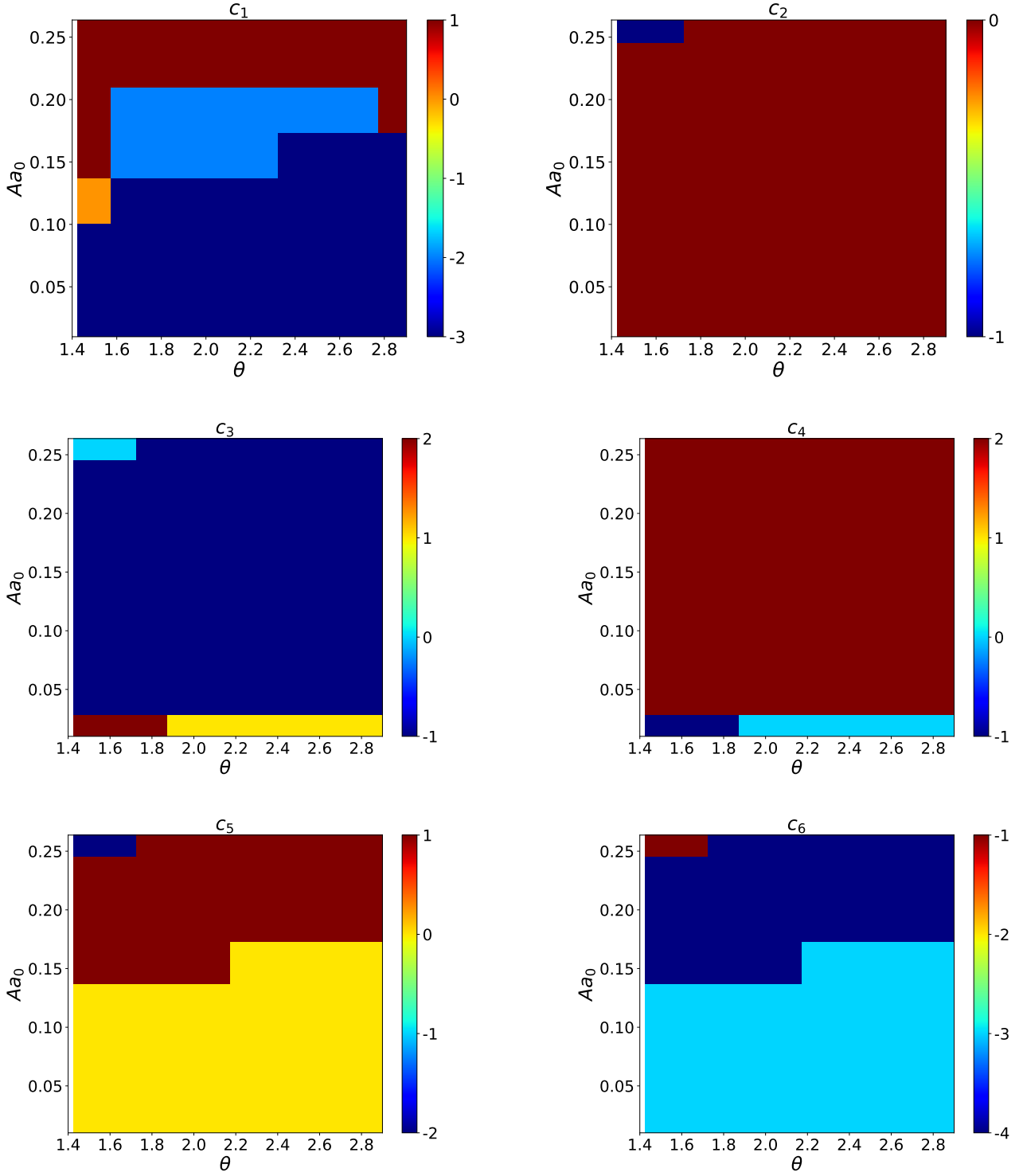
FIG. 17: (Color online) Topological maps for the six bands for the ABC stacking case with top layer twisting and right-handed circularly polarized light.
