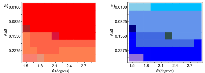
FIG. 9: (Color online) The topological phase diagrams for the TTG system with ABC stacking and top layer twisted where (a) for the left-handed circularly polarized light and (b) the right-handed circularly polarized light, where we took \omega = 2\gamma . For color codes, please refer to Table. I.
