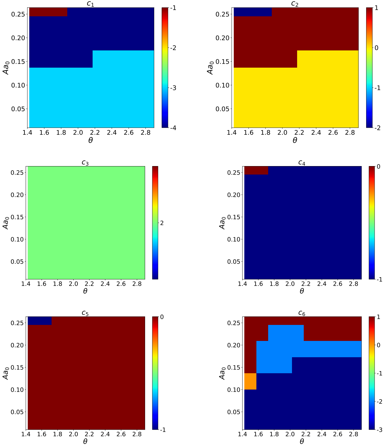
FIG. 18: (Color online) Reproduction of Fig. 17 but with incident light polarization being left-handed.
