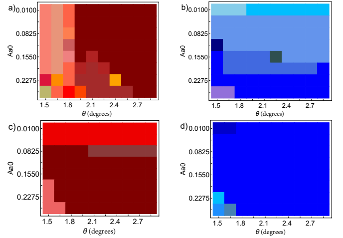
FIG. 7: (Color online) The topological phase diagrams for the TTG system for a range of values Aa_0 and the twist angle \theta with \omega = 2\gamma . (a) AAA stacking and top layer twist, (b) ABC stacking with top layer twisted, (c) AAA stacking with middle layer twisted, and (d) ABC stacking with middle layer twisted. Each color represents a set of values for the Chern numbers of the central six bands as indicated in Table I.
