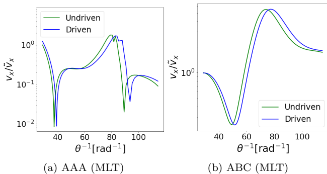
FIG. 12: Plot of velocity as function of 1/\theta for the center bands near K_1 in the twisted TTG system driven by waveguide light compared with the undriven case with Aa_0 = 0.3 , and \omega = 3\gamma . (a) Starting from AAA stacking middle layer twist (b) starting from ABC stacking middle layer twist. Here, \tilde{v}_x is the velocity at \theta = 2.0^\circ .
