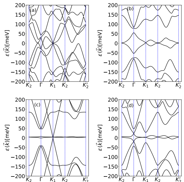
FIG. 2: (Color online) Band structure of the TTG with equilibrium Hamiltonian (Eq. 1) top layer twisted (top row) and middle layer twisted (bottom row) with twist angle \theta = 1.6^\circ . (a,c) Starting from AAA stacking and (b,d) starting from ABC stacking.
