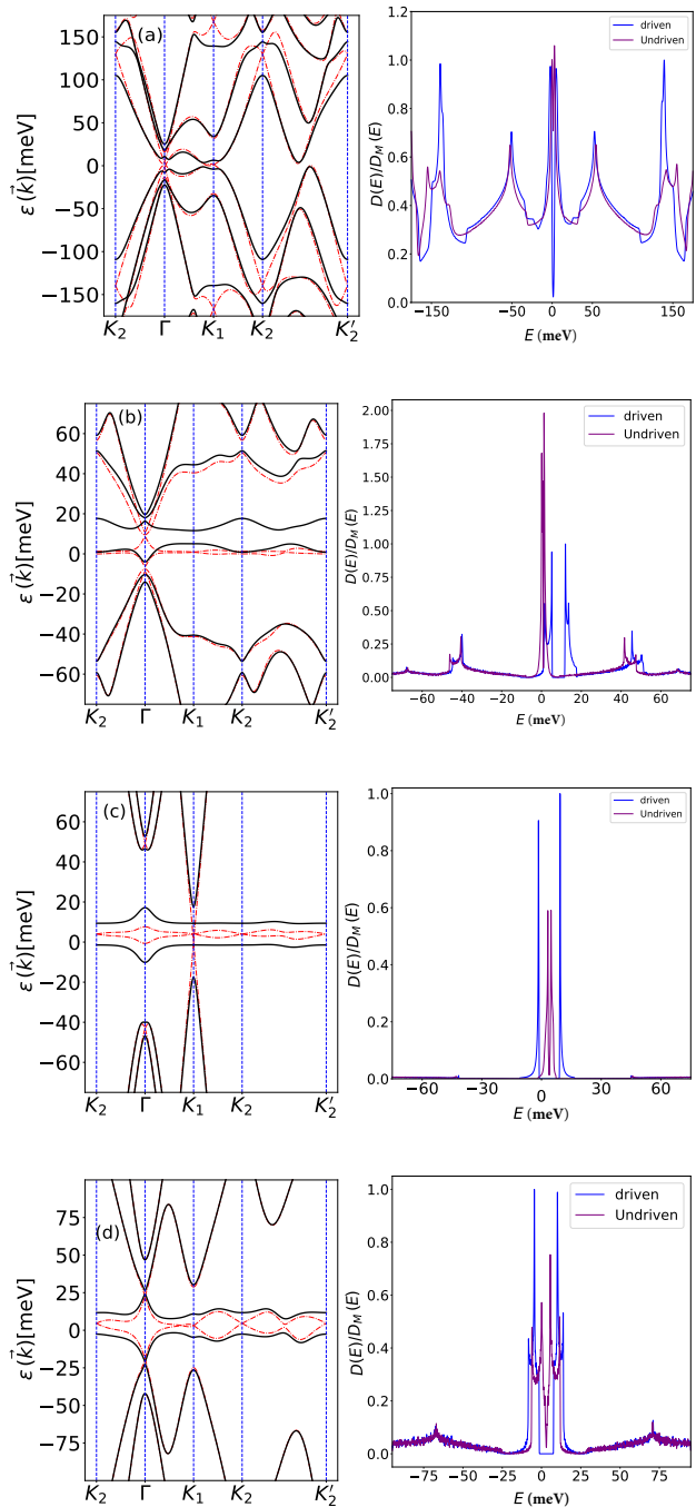
FIG. 4: (Color online) Band structure (left column) for TTG driven by circularly polarized light. (a) Starting with AAA stacking with TLT and parameters (\theta, Aa_0, \omega) = (1.8^\circ, 0.25, 2\gamma) , (b) the ABC with TLT and (\theta, Aa_0, \omega) = (1.0^\circ, 0.15, 3\gamma) , (c) AAA MLT and (\theta, Aa_0, \omega) = (1.6^\circ, 0.15, 3\gamma) , and (d) ABC MLT with (\theta, Aa_0, \omega) = (1.6^\circ, 0.15, 3\gamma) . In the above plots, the dash-dotted lines represent the undriven case and the solid lines represent the driven case. The corresponding density of states plots (DOS) are on the right column rescaled by D_M(E) which is the maximum value of the DOS of the driven case.
