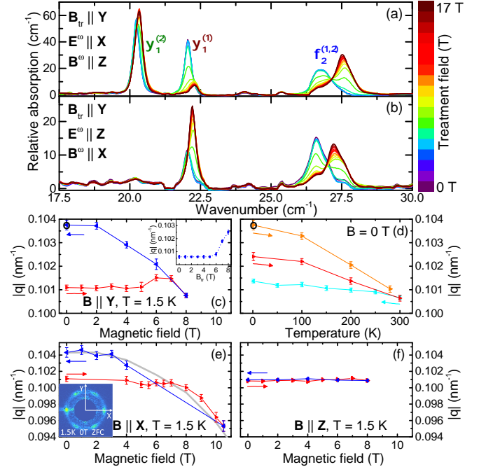
FIG. 4. (a)-(b): Zero-field THz absorption spectra measured at 3 K after the application of fields \mathbf{B}_{tr} \parallel \mathbf{Y} with magnitude continuously increasing to 17 T. The sample was heated above the Néel temperature and ZFC to 3 K before each sequence. The colour bar shows the highest treatment field, \mathbf{B}_{tr} preceding each zero-field measurement. The magnetic field dependence of the \mathbf{q} vector lengths, |q| measured with SANS at 2 K for \mathbf{B} \parallel \mathbf{Y} , \mathbf{B} \parallel \mathbf{X} and \mathbf{B} \parallel \mathbf{Z} are plotted in panel (c), (e) and (f), respectively. A typical SANS pattern is shown in the inset of panel (e). (d) Temperature dependence of the \mathbf{q} vector lengths for ZFC (light blue) and field treated (orange and red, in 8 T when \mathbf{B} \parallel \mathbf{Y} ) samples in zero field.
