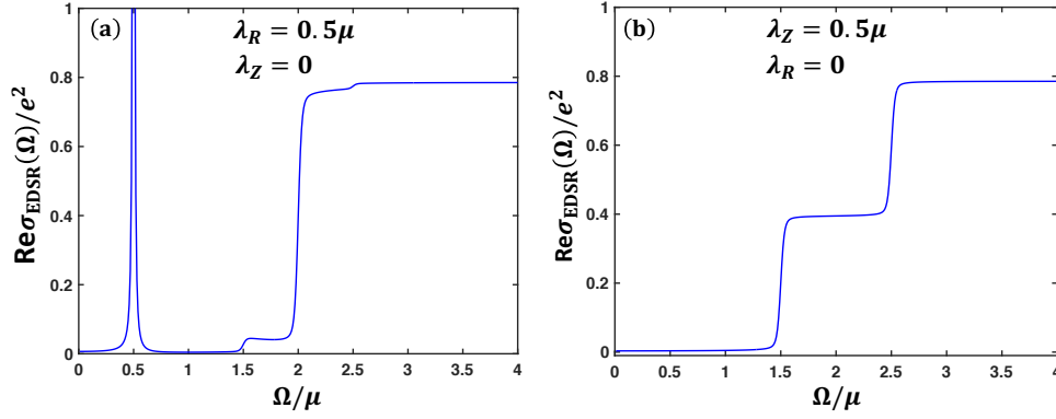
FIG. 3. Non-interacting electrons. (a) Real part of optical conductivity for Rashba SOC, showing the resonance at \lambda_R and continua starting at \Omega = 2\mu and \Omega = 2\mu \pm \lambda_R . The resonance is the zero-field EDSR effect. For the VZ case (b), there are continua starting at \Omega = 2\mu \pm \lambda_Z , but no resonance at \lambda_Z . VZ SOC does not lead to zero-field EDSR resonance. In both cases, the Drude part of the conductivity is not shown. Broadening is the same as in Fig. 2.
