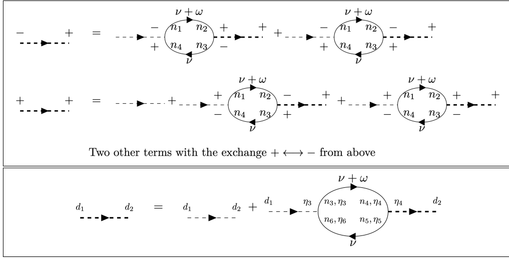
FIG. 5. The Dyson equations for the collective mode propagators. The bold dotted line denotes the recursively defined collective phonon. The bottom diagram generalizes the above diagrams [17, 18, 82, 83].
