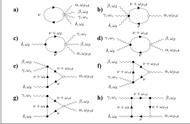
FIG. 11. Feynman diagrams for the non-collective contributions to the third-order conductivity[76]. Diagram h) is the only diagram that does not require regularization. Diagrams a), b), c), d), e), f), and g) exist to regulate diagram h) as \omega_{\delta} , \omega_{\gamma} , and \omega_{\beta} hit various singularities.
