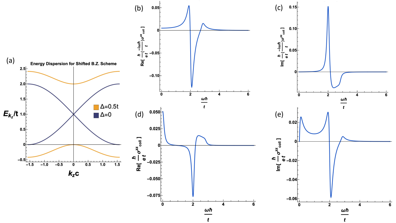
FIG. 17. Spectrum and conductivity for the tight-binding model of a 1D CDW. The spectrum is shown in (a), with both \Delta = 0 and \Delta = 0.5t . The plots of i\omega\sigma_{\text{coll}}^{zz} ((b) and (c)) and \sigma_{\text{coll}}^{zz} ((d) and (e)) are each shown in natural units. The real ((b) and (d)) and imaginary ((c) and (e)) parts are provided for the parameters \eta = 0.1t/\hbar and a gap \Delta = 0.5t , where the small self-energy \omega \rightarrow \omega + i\eta serves to numerically resolve the plot.
