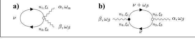
FIG. 6. Feynman diagrams for the non-collective contributions to the linear conductivity. a) is the diamagnetic term. b) is the single-particle term.
