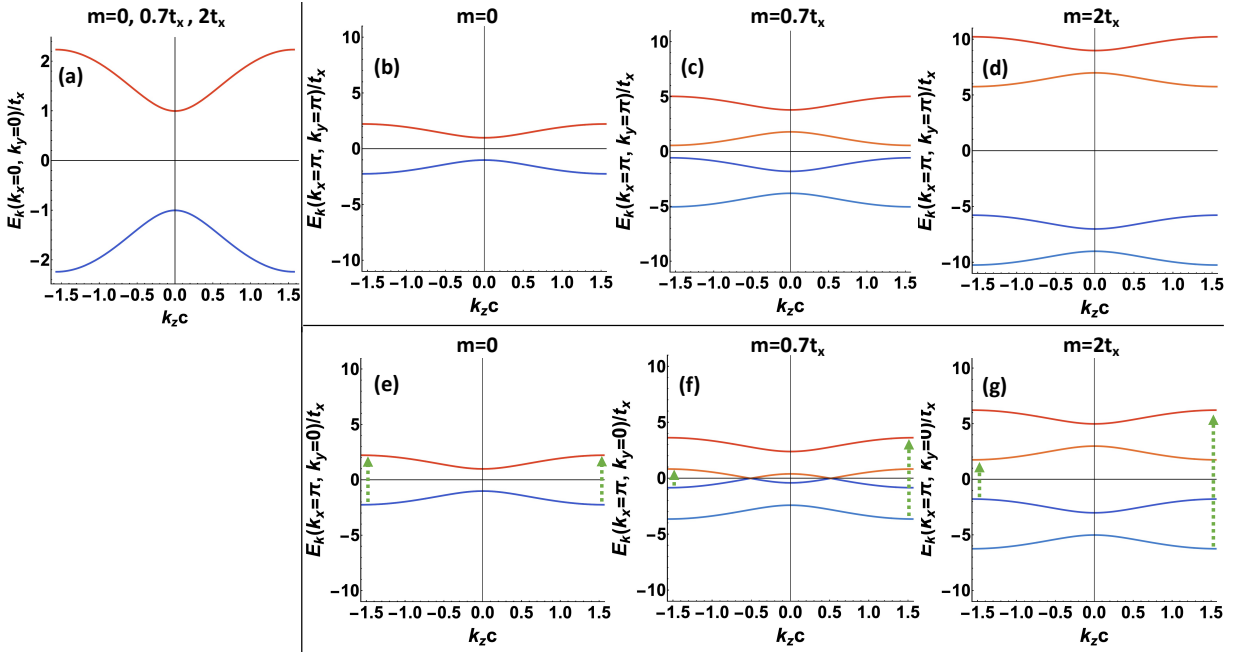
FIG. 1. The spectra for the lattice model with mean field electron-phonon interactions in the shifted Brillouin zone scheme, with t_x = t_y = t_z and \Delta = 0.5t_x . (a) is a cut through k_x = k_y = 0 , which shows the gapped Weyl nodes at k_z c = 0 . (b-d) are cuts through (k_x, k_y) = (\pi, \pi) , illustrating that the parameter m lifts the band degeneracy near the Brillouin zone edge. At m = 0 , three additional pairs of Weyl points exist at the Brillouin zone edge, which are gapped by the electron-phonon interaction as can be seen in (b) at k_z c = 0 . Plots (e-g) show a different slice of the spectra at (k_x, k_y) = (\pi, 0) , and the green arrows signify excitations described in Section IV C 2 b.
