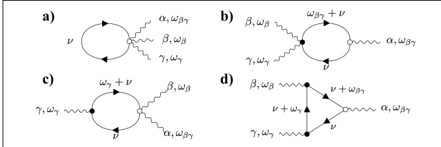
FIG. 9. Feynman diagrams for the non-collective second-order conductivity[76]. Diagram d) is the only diagram that does not require regularization, since all the vertices are linear in the electric field. Diagrams a), b), and c) exist to regulate diagram d) as \omega_{\gamma} and \omega_{\beta} hit various singularities.
