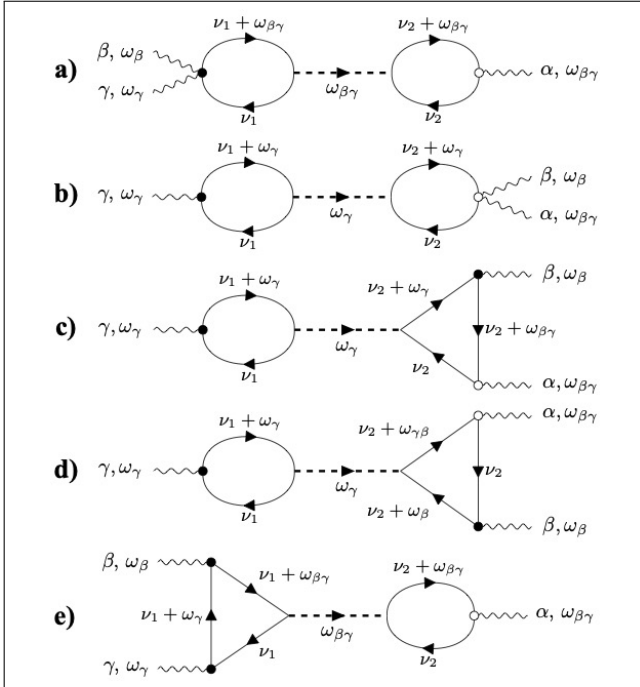
FIG. 10. Feynman diagrams for collective mode contributions to the second-order conductivity. Each diagram has a single-photon vertex loop contribution.
