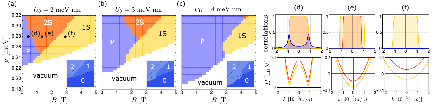
FIG. 4: Phase diagrams and zero-bias conductance with interactions and without SOC. (a-c), Phase diagrams of the waveguide near the crossing of the subbands \alpha = |0, 0, \downarrow\rangle and \beta = |0, 0, \uparrow\rangle as a function of magnetic field B and chemical potential \mu for different attractive interaction strength |U_0| = 2 meV nm (a), 3 meV nm (b), and 4 meV nm (c), and temperature T = 25 mK. The phase ‘P’ corresponds to a region where |\Delta| > 10^{-3} meV ( \sim k_B T ), i.e., when we have electron pairs. The phase ‘1S’ and ‘2S’ denote the phases where one and two single-particle bands are populated, respectively. The phase ‘vacuum’ denotes the phase where none of the single-particle bands is populated and no pairing is observed ( |\Delta| < 10^{-3} meV). The insets show the associated conductance (in units of e^2/h ), where the thin dashed lines correspond to the non-interacting case. Panels (d-f) show on the top the correlations \langle c_{\beta k}^\dagger c_{\beta k} \rangle (yellow), \langle c_{\alpha k}^\dagger c_{\alpha k} \rangle (red) and |\langle c_{\beta k} c_{\alpha - k} \rangle| (blue) appearing in the definitions of the mean-fields (19)-(21). The corresponding band structures appear at the bottom, showing e.g. in panel (d) (bottom) that a gap |\Delta| protects the band from single-particle excitations. Other parameters as in Fig. 3.
