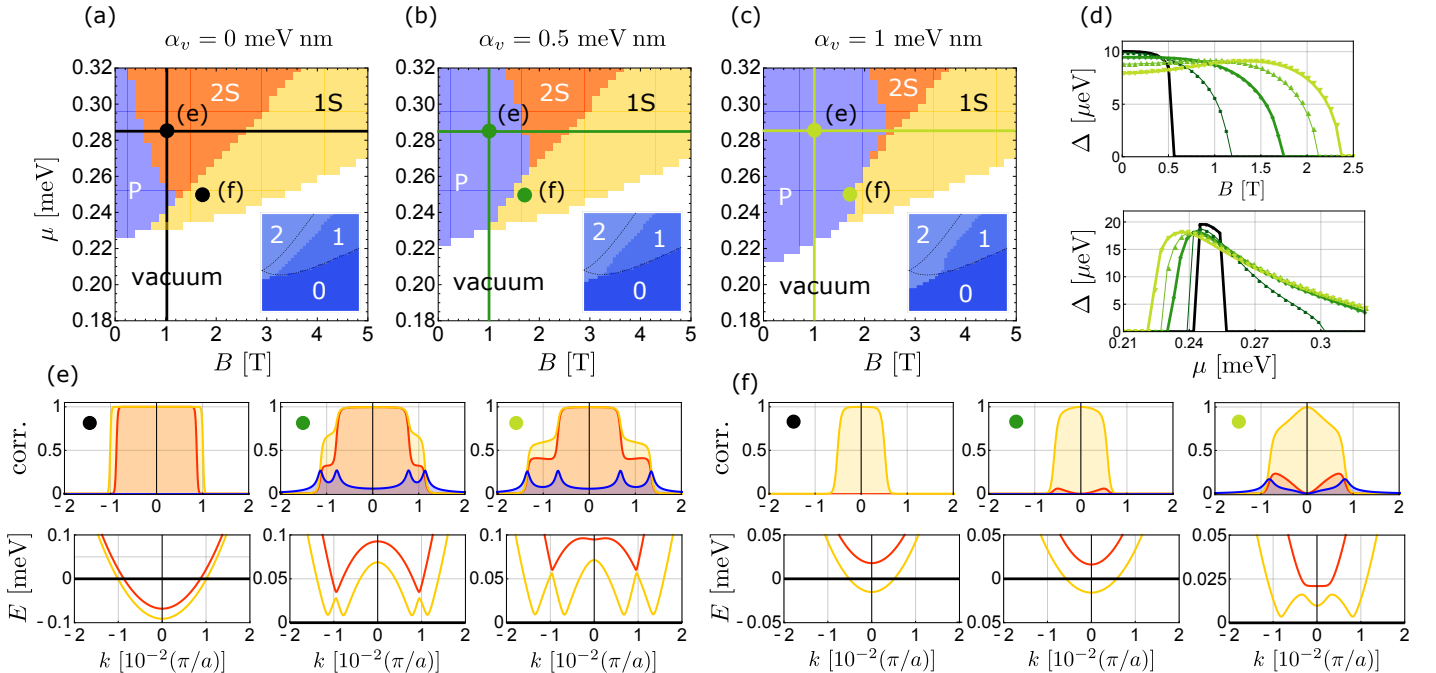
FIG. 5: Phase diagrams and zero-bias conductance with interactions and vertically-induced SOC ( \alpha_v \neq 0 ). (a-c) Phase diagrams of the waveguide near the crossing of the subbands \alpha = |0, 0, \downarrow\rangle and \beta = |0, 0, \uparrow\rangle as a function of magnetic field B and chemical potential \mu for different SOC strength \alpha_v = 0 meV nm (a), 0.5 meV nm (b), and 1 meV nm (c), for interaction strength |U_0| = 2 meV nm and temperature T = 25 mK. The phases are labelled as in Fig. 4, and the insets show the associated conductance. (d) Pairing \Delta across horizontal (top) and vertical (bottom) linecuts of the phase diagrams for SOC strength ( \alpha_v = 0, 0.25, 0.5, 0.75 and 1 meV nm). (e),(f) (top) Correlations \langle c_{\beta k}^\dagger c_{\beta k} \rangle (yellow), \langle c_{\alpha k}^\dagger c_{\alpha k} \rangle (red) and |\langle c_{\beta k} c_{\alpha - k} \rangle| (blue) appearing in the definitions of the mean-fields (19)-(21). (e),(f) (bottom) Corresponding band structures. Other parameters as in Fig. 3.
