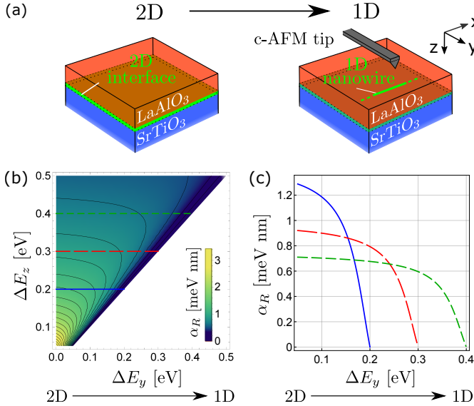
FIG. 2: Rashba SOC from 2D to 1D. (a) Sketch of the transition from a 2D conducting interface to a 1D nanowire as realized via c-AFM lithography. (b) Rashba SOC strength \alpha_R as a function of the lateral and vertical confinements \Delta E_y and \Delta E_z . The values of \alpha_R along the horizontal lines (corresponding to three specific values of \Delta E_z ) are shown more clearly on panel (c). (c) Rashba SOC strength \alpha_R as a function of the confinement \Delta E_y for \Delta E_z = 0.2 eV (solid blue line), 0.3 eV (red long-dashed line) and 0.4 eV (green short-dashed line). Increasing the confinement along \Delta E_y reduces the dimensionality of the system and the Rashba SOC.
