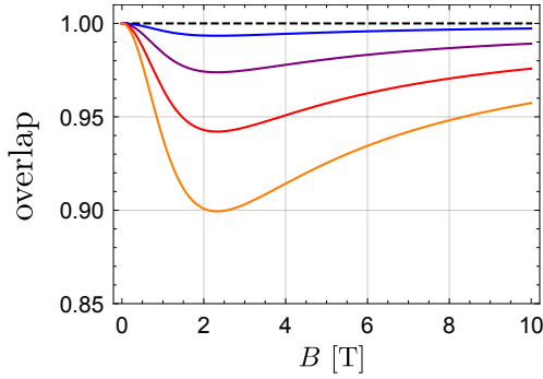
FIG. 7: Overlap [Eq. (34)] between the two spin-dependent eigenstates of along y as a function of magnetic field B for \alpha_l = 0 (dashed black), 0.25 (blue), 0.5 (purple), 0.75 (red) and 1 (orange) meV nm, for m_y = 2m_e , where m_e is the electron mass and l_y = \sqrt{\hbar/(m_y\omega_y)} = 20 nm.
