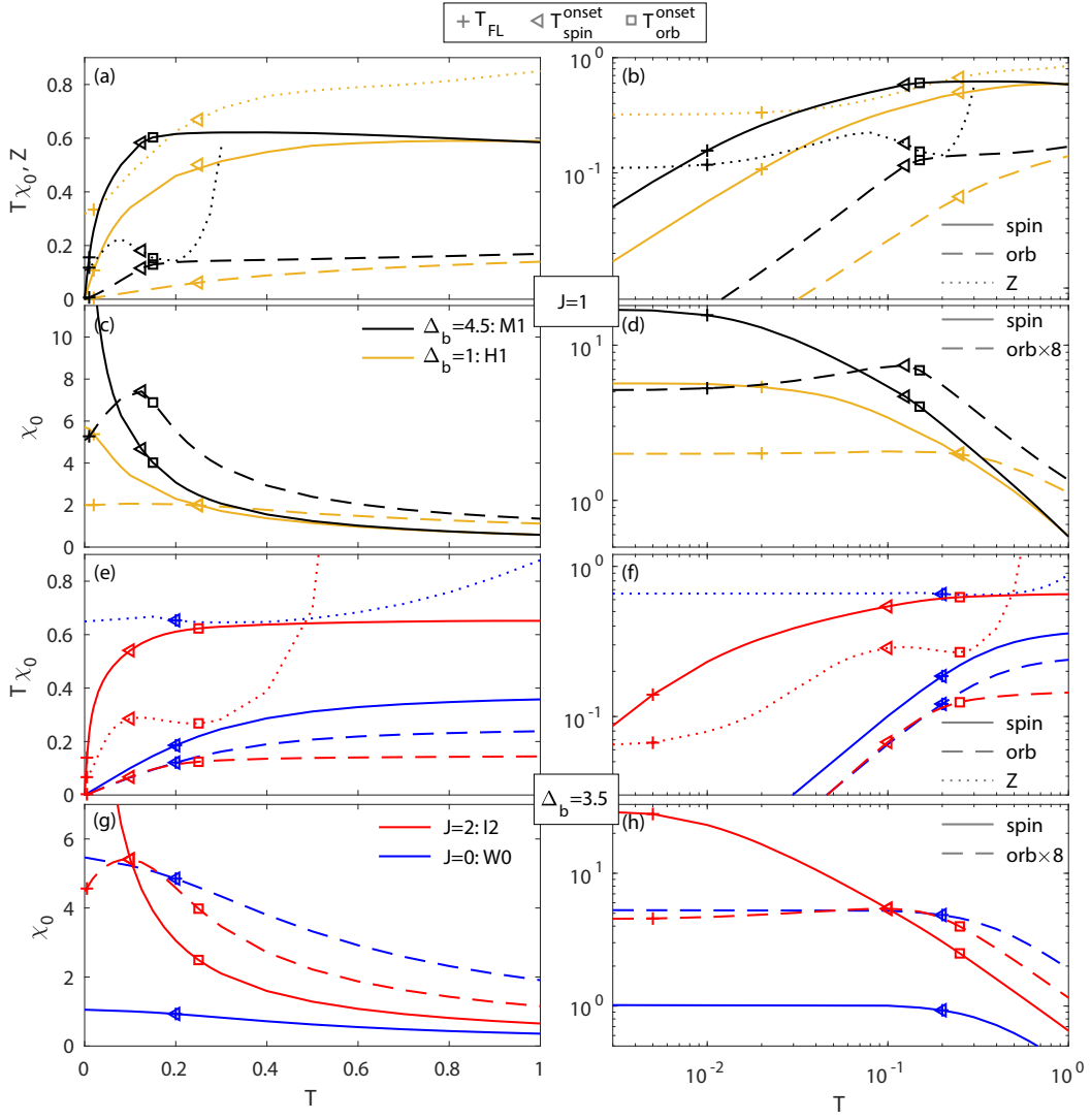
FIG. 7. The static local orbital (dashed) and spin (solid) susceptibilities, (a,b,e,f) T\chi_0^{orb,spin} and (c,d,g,h) \chi_0^{orb,spin} , all plotted as functions of temperature on a linear (left) and a logarithmic (right) scale, for M1 (black), H1 (yellow), I2 (red), and W0 (blue). In addition, the quasiparticle weight (dotted), Z(T) , is shown in (a,b,e,f). The squares mark the onset of orbital screening, T_{orb}^{onset} , below which T\chi_0^{orb} deviates from a constant value, i.e. from Curie-like behavior. Note that Z(T) diverges for T > T_{orb}^{onset} . The triangles mark the maxima of \chi_0^{orb} and also signal the onset of spin screening, T_{spin}^{onset} , below which T\chi_0^{spin} deviates from Curie-like behavior. The crosses denote the FL scale, T_{FL} , below which FL behavior is found. In M1, we observe that T_{spin}^{onset} \approx T_{orb}^{onset} = T_M . In H1, we find T_{orb}^{onset} \gg T_{spin}^{onset} , as discussed in Ref. [7]. The data for the static susceptibilities shown in panels (a-d) are adapted from Ref. [7]. A Curie-Weiss analysis of the data of panel (c) is presented in App. B.
