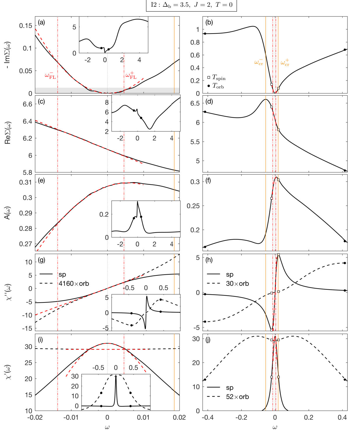
FIG. 13. (a,b) The imaginary part, \text{Im } \Sigma(\omega) , and (c,d) the real part, \text{Re } \Sigma(\omega) , of the self-energy; (e,f) the local spectral function, A(\omega) ; (g,h) the imaginary part, \chi''(\omega) , and (i,j) the real part, \chi'(\omega) , of the spin (solid) and orbital (dashed) susceptibility are plotted versus frequency for I2 ( \Delta_b = 3.5 , J = 2 ) at T = 0 . Left panels are zooms into the FL regime, whereas their insets show the quantities on a large frequency range. The SOS window is presented in the right panels. Dashed red fits reveal FL behavior for \text{Im } \Sigma(\omega) , \text{Re } \Sigma(\omega) , and A(\omega) in the asymmetric range, \omega_{\text{FL}}^- < \omega < \omega_{\text{FL}}^+ , with \omega_{\text{FL}}^+ \approx \frac{1}{3}\omega_{\text{FL}}^- (indicated by vertical dash-dotted red lines) and for the orbital and spin susceptibility in the symmetric range, |\omega| < \omega_{\text{FL}}^+ . The vertical solid yellow line at \omega < 0 denotes the energy scale, \omega_{\text{cr}}^- , of the maximum in \text{Re } \Sigma(\omega) at \omega < 0 . In (b), \omega_{\text{cr}}^+ = -\frac{1}{3}\omega_{\text{cr}}^- marks the kink in \text{Re } \Sigma(\omega) at \omega > 0 . Filled dots and open squares mark the orbital and spin Kondo scales, respectively. The grey area in (a) indicates a systematic error in \text{Im } \Sigma(\omega) (cf. Sec. 3.2 of Ref. [73] for details).
