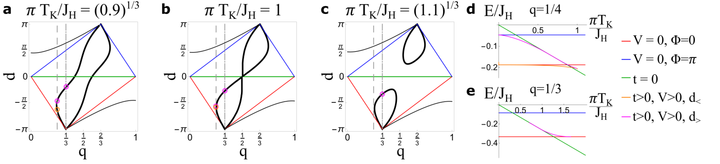
FIG. 4. Graphical illustration of mean field solutions. a - c Each point on the black curves corresponds to a solution of Eq. (8c) for a given value of the Doniach parameter \pi T_K/J_H . For q < 1/2 ( q > 1/2 ), we concentrate on d < 0 ( d > 0 ) (other solutions are “false vacua” indicated as thin lines). For comparison, we include analogous curves of solutions in the limit T_K = 0 [ t > 0, V = 0 (red) and t < 0, V = 0 (blue)] as well as J_H = 0 [ t = 0, V > 0 (green)]. The vertical gray dashed lines indicate the position of q = 1/4, 1/3 . For q = 1/4 there are up to two non-trivial solutions with -\pi < d < 0 (orange and pink circles, denoted d_< and d_> , respectively), while for q = 1/3 there is only one non-trivial solution (pink circle) in addition to the solution d = -\pi corresponding to complete Kondo breakdown ( V = 0 ). The corresponding mean field energy is plotted with the same color code in d, e , and compared to the solutions where either V = 0 or t = 0 .
