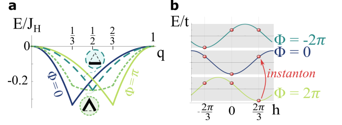
FIG. 3. a Ground state energies at T_K = 0 as a function of filling q , comparing rotationally symmetric solutions (labeled by their flux \Phi ) with symmetry broken states with one (two) non-zero t_m [graphically labeled by triangles with one (two) thick bonds]. b Single particle spectra of spinons at T_K = 0 with helicity quantum numbers h \in \{0, \pm 2\pi/3\} for different flux configurations \Phi = 0, \pm 2\pi . Instantons map \Phi \rightarrow \Phi \pm 2\pi and thereby reshuffle the wave functions but leave the spectrum unaltered.
