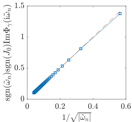
Figure 3. \text{sgn}(\tilde{\omega}_n) \text{sgn}(J_0) \text{Im } \Phi_\gamma(i\tilde{\omega}_n) as a function of 1/\sqrt{|\tilde{\omega}_n|} for 100 values of |\tilde{\omega}_n| . At large |n| , \Phi_\gamma(i\tilde{\omega}_n) approaches the zero-temperature form i \text{sgn}(J_0) \text{sgn}(\tilde{\omega}_n) \sqrt{2\pi} |\tilde{\omega}_n|^{-1/2} , indicated by the red dashed line.
