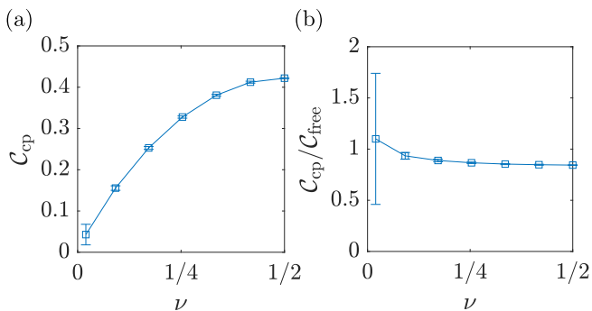
Figure 7. (a) C_{\text{cp}} for an antisymmetric tensor impurity as a function of \nu for \nu \leq 1/2 . Error bars are indicated. Note that \chi_{\text{imp}} for the filling \nu is the same as that for the filling 1 - \nu due to the particle-hole symmetry. (b) C_{\text{cp}}/C_{\text{free}} as a function of \nu .
