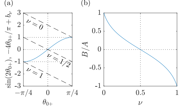
Figure 5. (a) Both sides of (81) as functions of \theta_{0+} . The blue solid line represents the left-hand side. The black dashed lines represent the right-hand side which is a linear function with intercept b_\nu = -4\nu + 2 , plotted for a few different values of \nu as indicated in the figure. (b) Solution for B/A as a function of \nu in the case \Delta = 1/4 .
