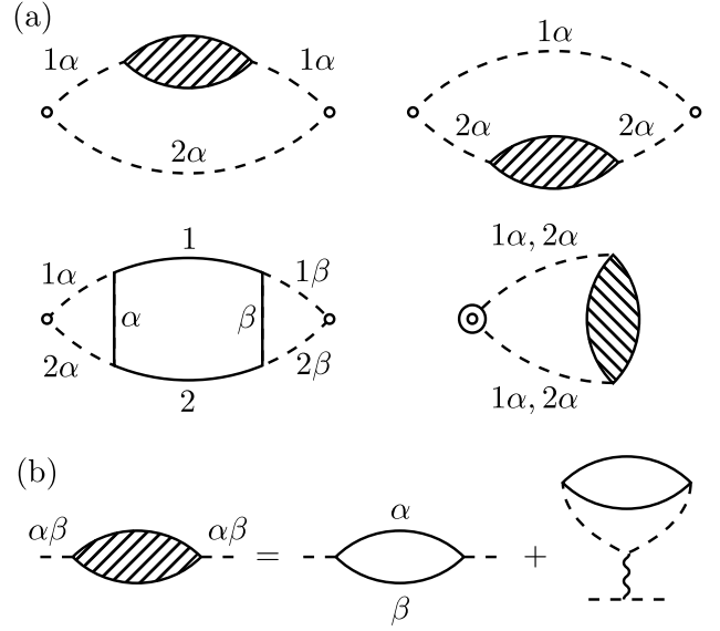
Figure 4. (a) Feynman diagrams relevant in the large- N limit for \chi_{b,b} , the bulk-bulk part of the impurity susceptibility to a uniform magnetic field. Single circles are source terms of the form (\partial_\tau \phi)\phi which couples linearly to h , and double circles are source terms of the form \phi^2 which couples to h^2 (cf. Eq. (50)). The solid lines are Majorana fermion propagators and the dashed lines are \phi boson propagators. (b) The shaded bubble which appears in the first panel. The wavy line represents the propagator of the Lagrange multiplier field \lambda and is of order 1/N^2 .
