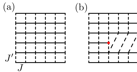
Figure 1. (a) A spin-1 antiferromagnetic Heisenberg model. The Heisenberg couplings on horizontal bonds are J , while the couplings on vertical bonds are J' . When J'/J is sufficiently small, the system is in a topological paramagnetic phase protected by the SO(3) spin rotation symmetry and translation symmetry. As we increase J'/J up to 1, there is a transition to the Néel ordered phase. (b) A dislocation defect with a (1, 1) Burgers vector, which supports a spin-1/2 topological mode in the paramagnetic phase.
