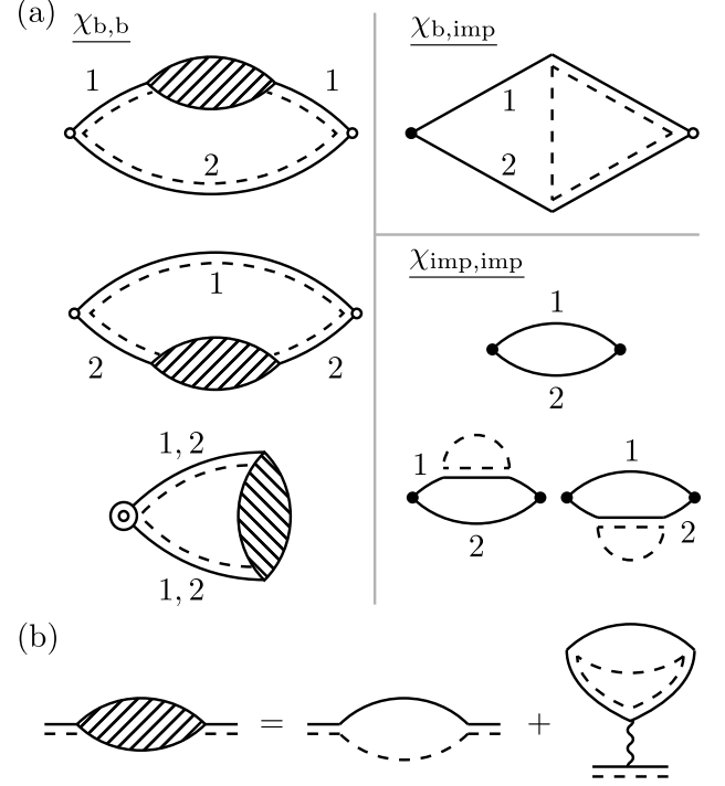
Figure 2. (a) Feynman diagrams at order 1 and 1/N for the impurity susceptibility \chi_{\text{imp}} . Single circles are bulk source terms of the form (\partial_\tau \phi)\phi , double circles are bulk source terms of the form \phi^2 which couples to h^2 and black solid dots are impurity source terms of the form \gamma\gamma (cf. Eq. (30)). The solid lines are propagators for \gamma_\alpha with \alpha \geq 1 and the dashed lines are \gamma_0 propagators. \phi boson propagators are represented by double lines (solid and dashed). (b) The shaded bubble which appears in the first panel. The wavy line represents the propagator of the Lagrange multiplier field \lambda and is of order 1/N .
