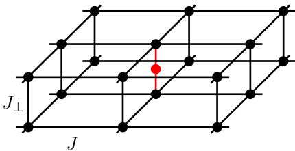
Figure 8. Bilayer antiferromagnet and an impurity (marked as a red dot) symmetric under the \mathbb{Z}_2 layer interchange symmetry.
