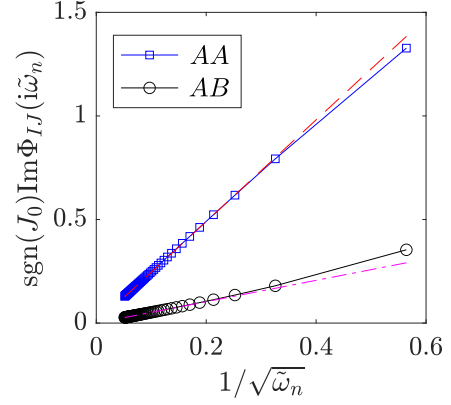
Figure 6. \text{sgn}(J_0) \text{Im } \Phi_{IJ}(i\tilde{\omega}_n) as a function of 1/\sqrt{i\tilde{\omega}_n} for 60 positive values of \tilde{\omega}_n . Blue squares and black circles represent IJ = AA and IJ = AB , respectively. The filling fraction is estimated to be \nu = 0.3354 \pm 0.0001 by a linear fitting of F_2(i\tilde{\omega}_n)/F_1(i\tilde{\omega}_n) with respect to 1/\tilde{\omega}_n using the 13 smallest positive frequency values. Red dashed lines and purple dotted-dashed lines indicate the asymptotic (zero-temperature) behavior for \nu = 1/3 .
