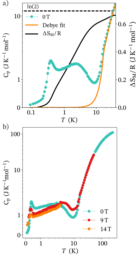
FIG. 3. a) Specific heat C_p(T) of KCeO 2 (cyan) measured in zero magnetic field and plotted with a Debye fit (orange) modeling lattice contributions. The magnetic specific heat peaks at 300 mK, suggesting KCeO 2 enters an ordered state. The integrated magnetic entropy is overplotted as a black line and approaches R\ln(2) at high temperature (indicated by the horizontal dashed black line). b) C_p(T) of KCeO 2 collected under fields of \mu_0 H = 0, 9 , and 14 T.
