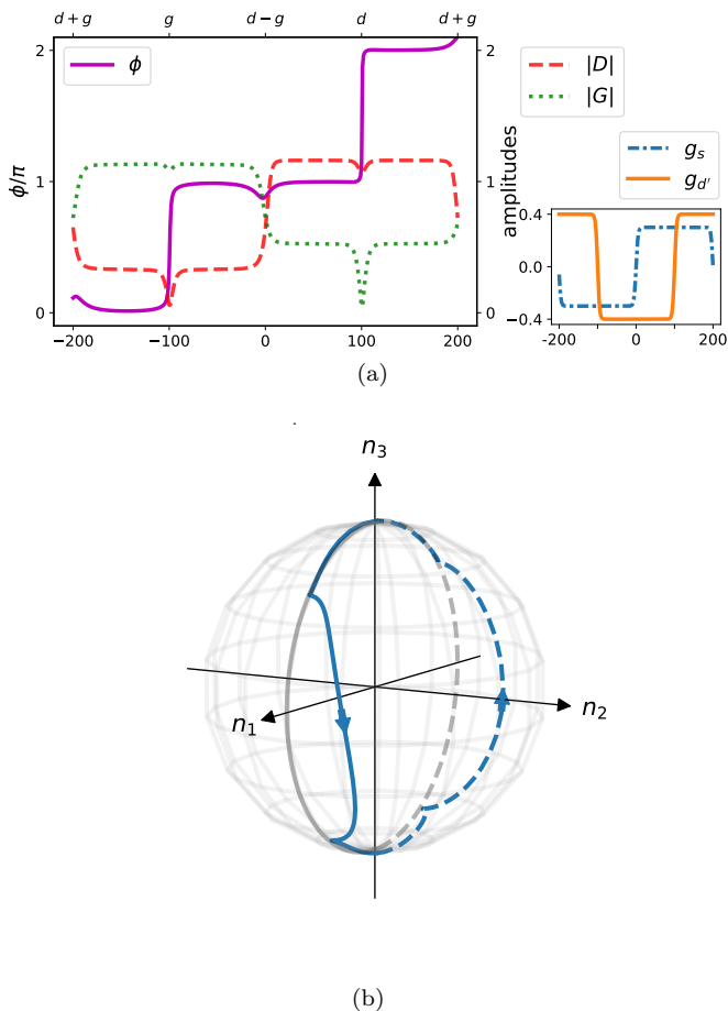
FIG. 7. Half quantum vortex pinned by strain texture a . (a) The behavior of the OP \Delta = (D, G) as a function of x . The two components of the strain, g_s(x) \propto \alpha_3 and g_{d'}(x) \propto \alpha_1 , are shown on the right. The domain walls are of the form \pm \tanh(x/l) with l = 5 , and the cylinder's circumference is 400 sites. The solid line represents the relative phase \phi given by the left vertical axis, while the dashed lines represent that amplitudes |D| and |G| (right vertical axis). The bottom horizontal axis represents the x position, while the top horizontal axis is labeled with the uniform state corresponding to the given strain texture at that position. (b). Trajectory of the OP \Delta = (D, G) projected onto the unit Bloch sphere. The arrow represent the direction of the contour. The gray circle line emphasizes the \hat{e}_1 - \hat{e}_3 plane.
