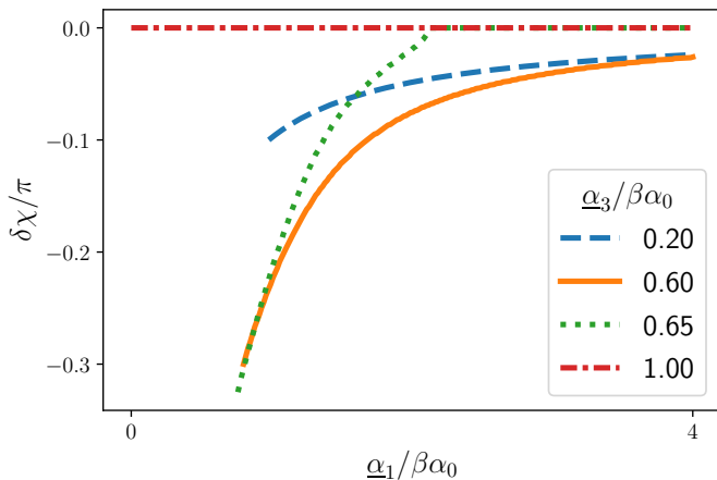
FIG. 3. Global phase a . The change \delta\chi in the global phase across a narrow domain wall where the xy component of the strain, \alpha_1 , is discontinuous. The domain wall is characterized by \alpha_1(y) = \underline{\alpha}_1 \text{sign}(y) , while \alpha_3(y) = \underline{\alpha}_3 is constant. \delta\chi is shown as a function of \underline{\alpha}_1/\beta\alpha_0 . The different curves correspond to different fixed values of the uniform component of the strain, \underline{\alpha}_3/\beta\alpha_0 .
