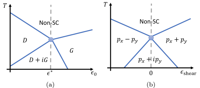
FIG. 1. (a) a . Schematic phase diagram as a function of two parameters - taken here to be isotropic strain ( \epsilon_0 ) and T , in the neighborhood of a tetra-critical point at which the transition temperatures to SC states with d -wave (i.e. B_{1g} ) and g -wave (i.e. A_{2g} ) coincide. (b). A similar schematic phase diagram - now where the x -axis signifies symmetry breaking shear strain, \epsilon_{\text{shear}} - for a system which at zero strain favors a SC order parameter the transforms according to a two dimensional irrep., p_x and p_y (i.e. E_u symmetry).
