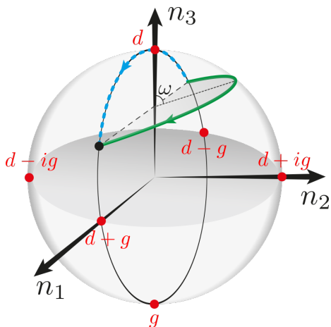
FIG. 2. Domain Walls a . The figure is the Bloch sphere representation of possible transitions across the domain wall where \alpha_1(y) \rightarrow \pm\alpha_1 as y \rightarrow \pm\infty , and \alpha_3(y) \equiv \alpha_3 > 0 is constant. The dashed blue arrow represents a TRS preserving transition through a pure d state. The solid green arrow represents a general TRSB transition restricted to a 2D plane intersecting the Bloch sphere, the angle of which relative to the \hat{e}_1 - \hat{e}_3 plane is denoted by \omega . In particular, if \omega = \pi/2 , then only the relative phase \phi changes from \phi = \pi \rightarrow 0 .
