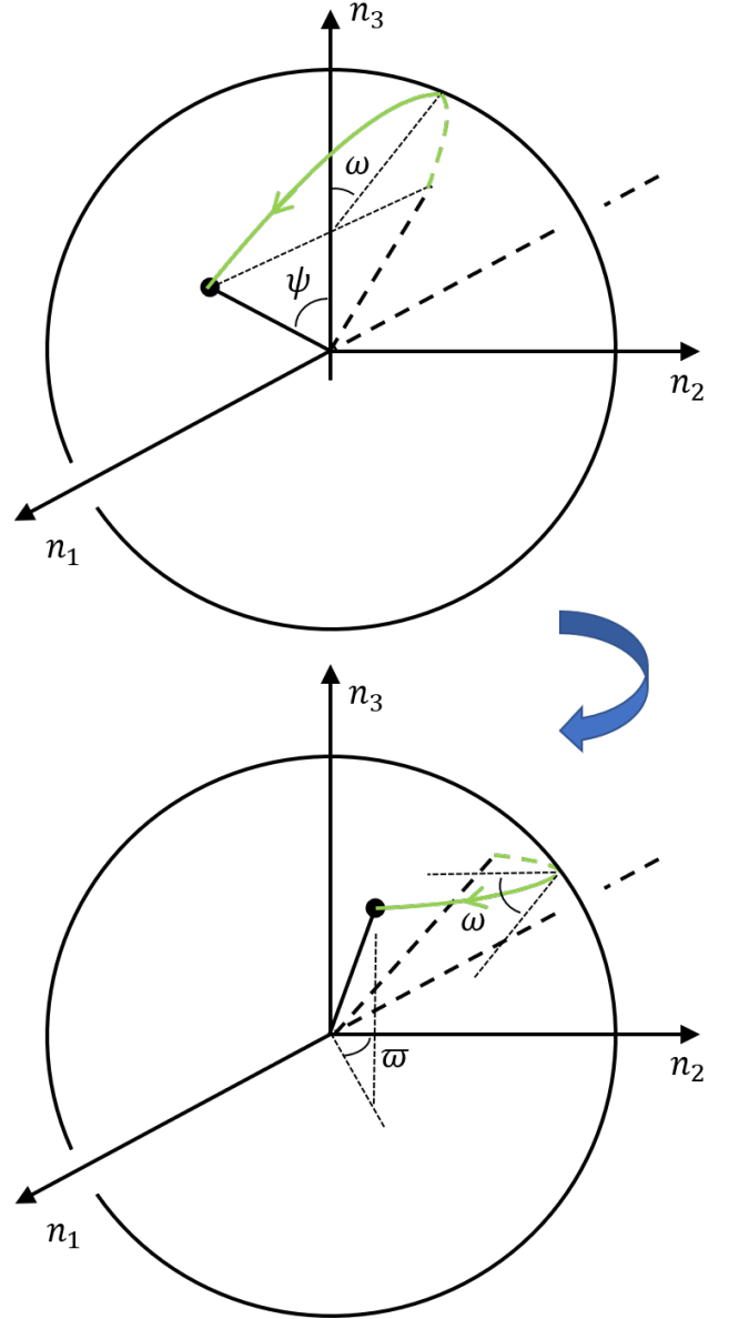
FIG. 8. General TRSB Domain Wall. The top figure is the Bloch sphere representation of a general TRSB transition through the domain wall \alpha_1(y) = \alpha_1 \text{sign}(y) . The arrow representing the transition path is assumed to be in a plane at angle \omega with respect to the \hat{e}_1 - \hat{e}_3 plane. The bottom figure is the transition rotated of angle \omega about the +x -axis in the clockwise direction.
