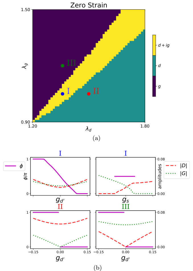
FIG. 5. (a) a Phase diagram of the microscopic Hamiltonian, Eq. (12,13), as a function of the interaction strengths \lambda_d, \lambda_g , calculated within self-consistent mean-field theory, in the absence of strain. Near degeneracy \lambda_d \sim \lambda_g , the middle portion denotes the TRSB d + ig state, while the bottom and top regions represent a pure d and pure g state, respectively. 3 representative point (I, II, III), one in each phase, are used in further calculations. (b) The top two panels depict the evolution of the uniform state at point (I) with shear g_{d'} and isotropic g_s strain. The solid line represents the relative phase \phi given by the left y -axis, while the dashed lines represent the amplitudes |D|, |G| , given by the right y -axis. Similarly, the bottom two panels represent the evolution of the uniform state for sample points (II) and (III) under shear g_{d'} strain.
