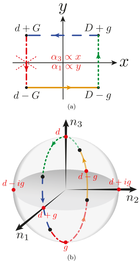
FIG. 4. A strain induced half quantum fluxoid a . (a) Real space contour around a topological point defect, along which the strain vector \alpha winds by 2\pi . The dashed cross shows the location of a \pi mismatch in the phase of the order parameter. D+g in the x > 0, y > 0 quadrant represents order parameter with a dominant D component and a smaller G component, and similarly in the other quadrants. (b) Corresponding trajectory of the order superconducting order parameter along the Bloch sphere. TRS is preserved along the path. Each segment of the contour is color/style-coded so that the same colors/line styles in the bottom and top figure correspond to each other.
