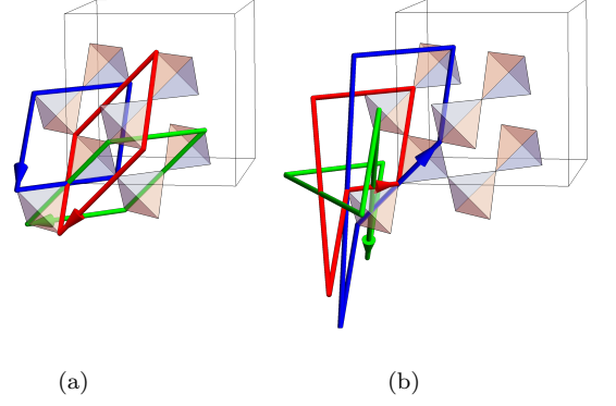
FIG. 1. Examples of loops for (a) T_i T_{i+1} T_i^{-1} T_{i+1}^{-1} = 1 and (b) ST_1 S^{-1} T_3^{-1} T_1 = 1 .
