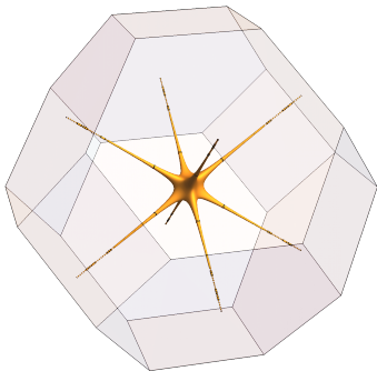
FIG. 2. Illustration of the nodal star Fermi surface; the contour corresponds to an energy infinitesimally above the Fermi level.
