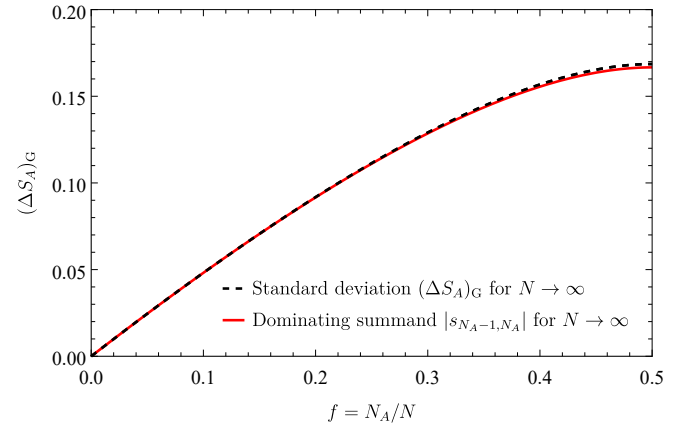
FIG. 3. We compare the standard deviation \lim_{N \rightarrow \infty} (\Delta S_A)_G from (25) with the leading summand |\bar{s}_{0,0}| = \lim_{N \rightarrow \infty} |s_{N_A-1, N_A}| = \frac{(3-4f)f}{6(1-f)} from (24).
