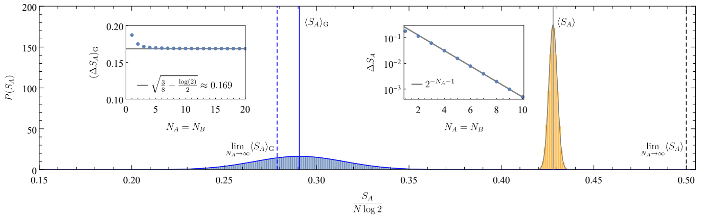
FIG. 2. We compare the probability distributions P(S_A) of the entanglement entropy S_A for Gaussian states and general states in a fermionic system with N_A = N_B = 5 . The expectation value \langle S_A \rangle and \langle S_A \rangle_G for N_A = N_B and their thermodynamic limits are indicated by vertical lines and vertical dashed lines, respectively. The insets depict the scaling of the standard deviation \Delta S_A and (\Delta S_A)_G for N_A = N_B \rightarrow \infty .
