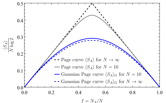
FIG. 1. We compare the Page curve for random states \langle S_A \rangle to the Page curve for random Gaussian states \langle S_A \rangle_G for a system with N fermionic degrees of freedom.
