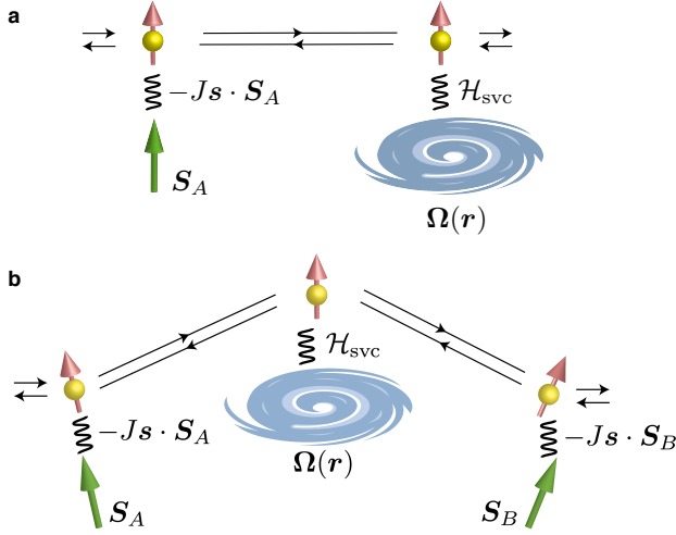
FIG. 2. Schematic descriptions of our theory. a , The Zeeman field acting on the localized spin due to vorticity. b , The DM interaction between the localized spins. The two green arrows represent the two localized spins S_A and S_B , and the red arrows with yellow spheres denote the conduction electron spins s , which interact through the exchange interaction J . The conduction electron spin also couples the vorticity \Omega(r) through SVC.
