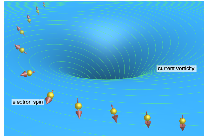
FIG. 1. Schematic figure of the spin-vorticity coupling. The red arrow with yellow sphere denotes the conduction electron spin, which is scattered by the current vorticity due to the spin-vorticity coupling.
