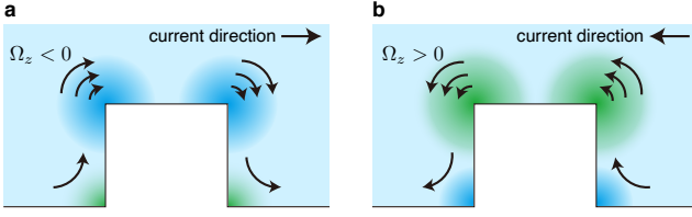
FIG. 3. Schematic description of the vorticity \Omega due to the electric current near the notch structure. a , When the current is applied along the left-to-right direction, the vorticity is nonzero at four corners of the notch; the blue-colored areas have the opposite vorticity direction to the green-colored areas. b , The current direction is reversed from a ; the vorticity direction is also reversed. Note that the absolute value of the vorticity does not change between the left-to-right and right-to-left currents. Since the vorticity-induced Zeeman field is proportional to the vorticity, the direction of the Zeeman field depends on that of vorticity and thus the current.
