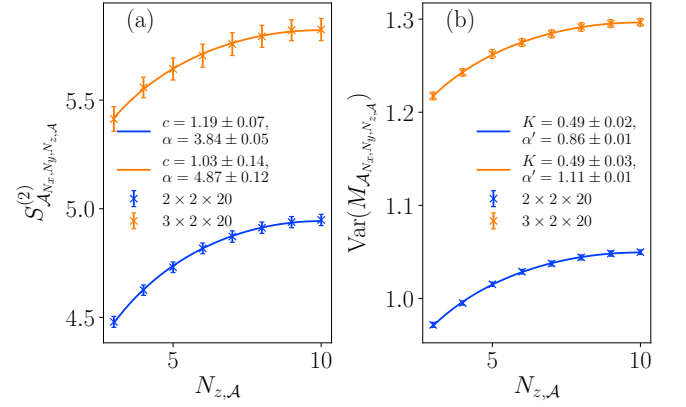
FIG. 2. Second Renyi entropy and spin fluctuations of the interacting model wave function |\Psi\rangle for a series of subsystems \mathcal{A}_{N_x, N_y, N_z, \mathcal{A}} 58 . We plot MC data obtained for two different systems sizes 2 \times 2 \times 20 (in blue) and 3 \times 2 \times 20 (in orange). (a) Scaling of the second Renyi entropy, fit to the prediction of Eq. (3). (b) Scaling of the spin fluctuations, fit to the prediction of Eq. (6).
