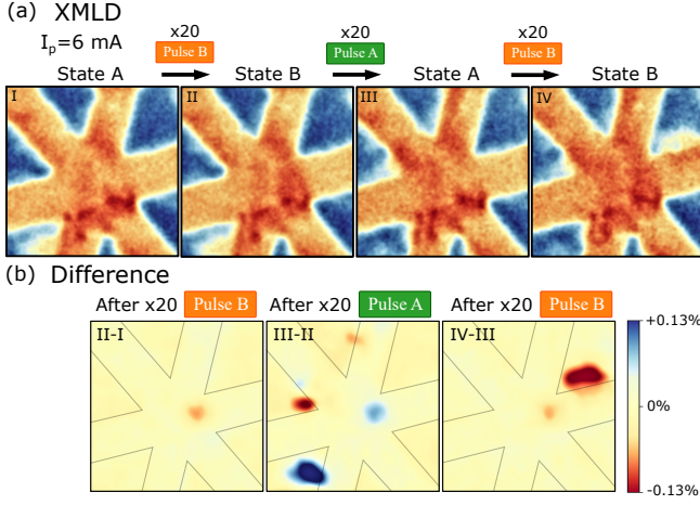
FIG. 4. AFM domain response to larger amplitude current pulses. (I) (a) I. State A, initial sample state. Followed by images after II. 20 \times B pulses, III; 20 \times A pulses, IV. 20 \times B pulses. In each case the current amplitude was 6 mA. (b) Differences of XMLD images in panel (a) highlight the pulse induced changes, with an expanded color scale, the same as the that of Fig. 2(b).
