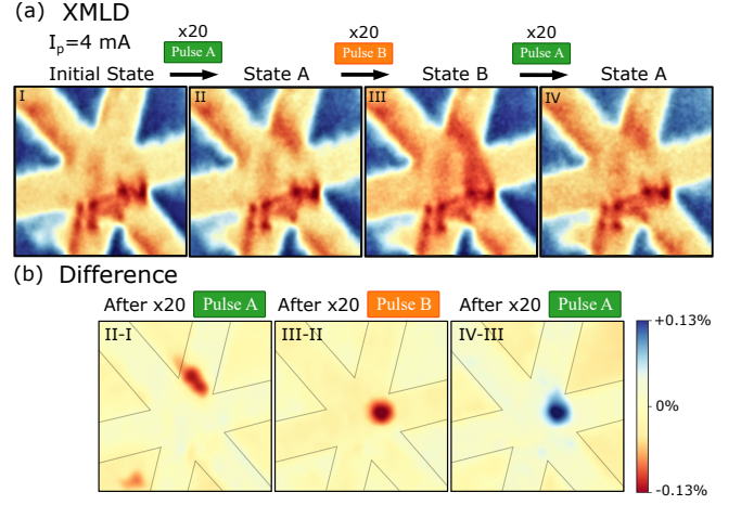
FIG. 2. AFM domain changes in response to current pulses. (a) XMLD images showing a 4 \times 4 \mu\text{m}^2 field of view. Image I shows the sample before current is applied; Images II, III and IV are images taken after the application of 20 current pulses of type A, type B and then type A, respectively. The pulse amplitude is 4 mA for all the images in the sequence. (b) Differences of XMLD images in panel (a) to highlight the pulse induced changes to AFM domain structure. The color scale in (b) is expanded to highlight changes.
