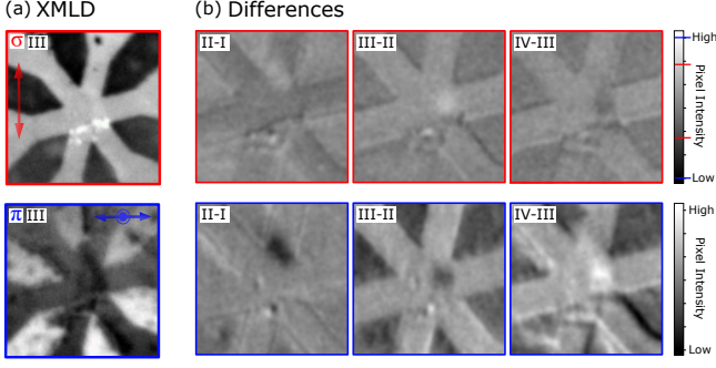
FIG. 3. (a) \sigma and \pi projections of Image III in Fig. 2a. Bright regions indicate that the AFM order is aligned perpendicular to the polarization direction whereas dark regions indicate that the AFM order aligns parallel to the polarization direction. (b) \sigma (top panel) and \pi (bottom panel) projections of the difference images in Fig. 2b. The same scale bar is used on both panels to highlight the larger contrast in the \pi polarization images. The marks on the \sigma color scale bar show the maximum and minimum values for \sigma (red marks) and \pi (blue marks) polarization difference images.
