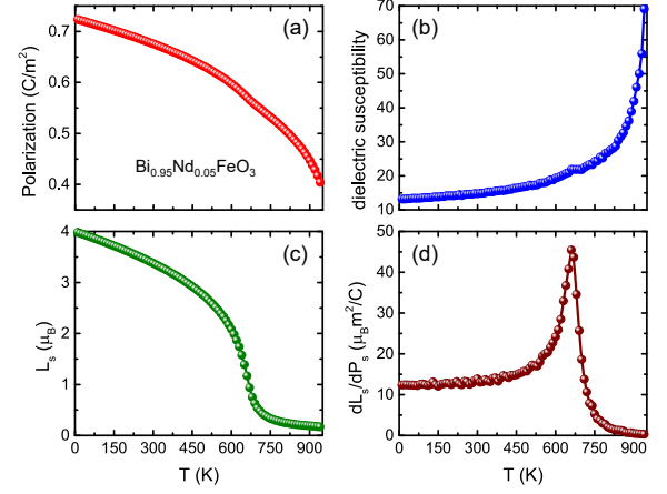
FIG. 2. Temperature dependence of some properties in disordered Bi 0.95 Nd 0.05 FeO 3 alloys, as obtained from our MC simulations: (a) the macroscopic polarization P_s ; (b) the average between the three diagonal elements of the dielectric susceptibility; (c) the AFM vector; and (d) the derivative dL_s/dP_s .
