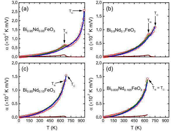
FIG. 1. Electrocaloric coefficient, \alpha , as a function of the temperature for different compositions in disordered \text{Bi}_{1-x}\text{Nd}_x\text{FeO}_3 alloys: (a) \text{Bi}_{0.95}\text{Nd}_{0.05}\text{FeO}_3 ; (b) \text{Bi}_{0.9}\text{Nd}_{0.1}\text{FeO}_3 ; (c) \text{Bi}_{0.85}\text{Nd}_{0.15}\text{FeO}_3 ; and (d) \text{Bi}_{0.835}\text{Nd}_{0.165}\text{FeO}_3 . The solid green lines represent the fit of the MC results by the second line of Eq. (11), i.e., \alpha = \frac{T_0 a'(T)}{C_{ph}} P_s \varepsilon_0 \chi + \frac{T_0 b'(T)}{C_{ph}} L_s \left. \frac{\partial L_s}{\partial P_s} \right|_T \varepsilon_0 \chi , where a'(T) = A_0 + A_1 T ( A_0 and A_1 being fitting constants), and C_{ph} and b'(T) are also fitting parameters. The solid blue lines display the fit of the MC results by its first contribution, \frac{T_0 a'(T)}{C_{ph}} P_s \varepsilon_0 \chi . The solid brown lines correspond to the fit of the MC results by its second contribution, \frac{T_0 b'(T)}{C_{ph}} L_s \left. \frac{\partial L_s}{\partial P_s} \right|_T \varepsilon_0 \chi (see text).
