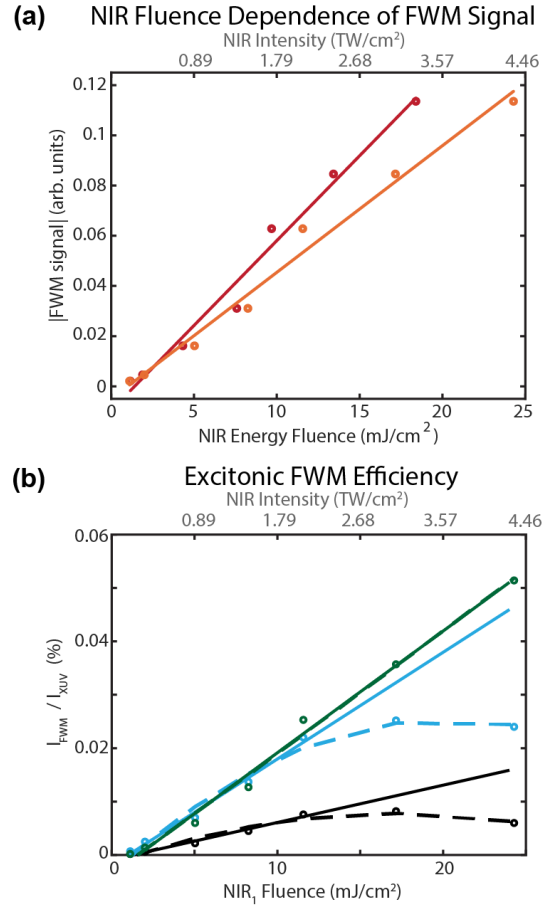
FIG. 4. NIR Fluence Dependence and Generation Efficiency of the FWM Signal. (a) The NIR fluence dependence of the strongest Na^+ core-excited at 33.61 eV for k_{NIR1} (orange) and k_{NIR2} (red); spectra are collected at temporal overlap. (b) The excitonic FWM efficiency calculated for the three main core-exciteds with increasing k_{NIR1} fluence observed at temporal overlap. Linear (solid) and quadratic (dashed) fits; 33.27 eV = black, 33.42 eV = light blue, 33.61 eV = green. Fluence dependence of FWM signal and excitonic efficiencies are all linear below 12 mJ/cm^2 (2.14 TW/cm^2 ), NIR fluences in the 8-10 mJ/cm^2 (1.43-1.79 TW/cm^2 ) were used in the FWM studies to stay in the linear regime.
