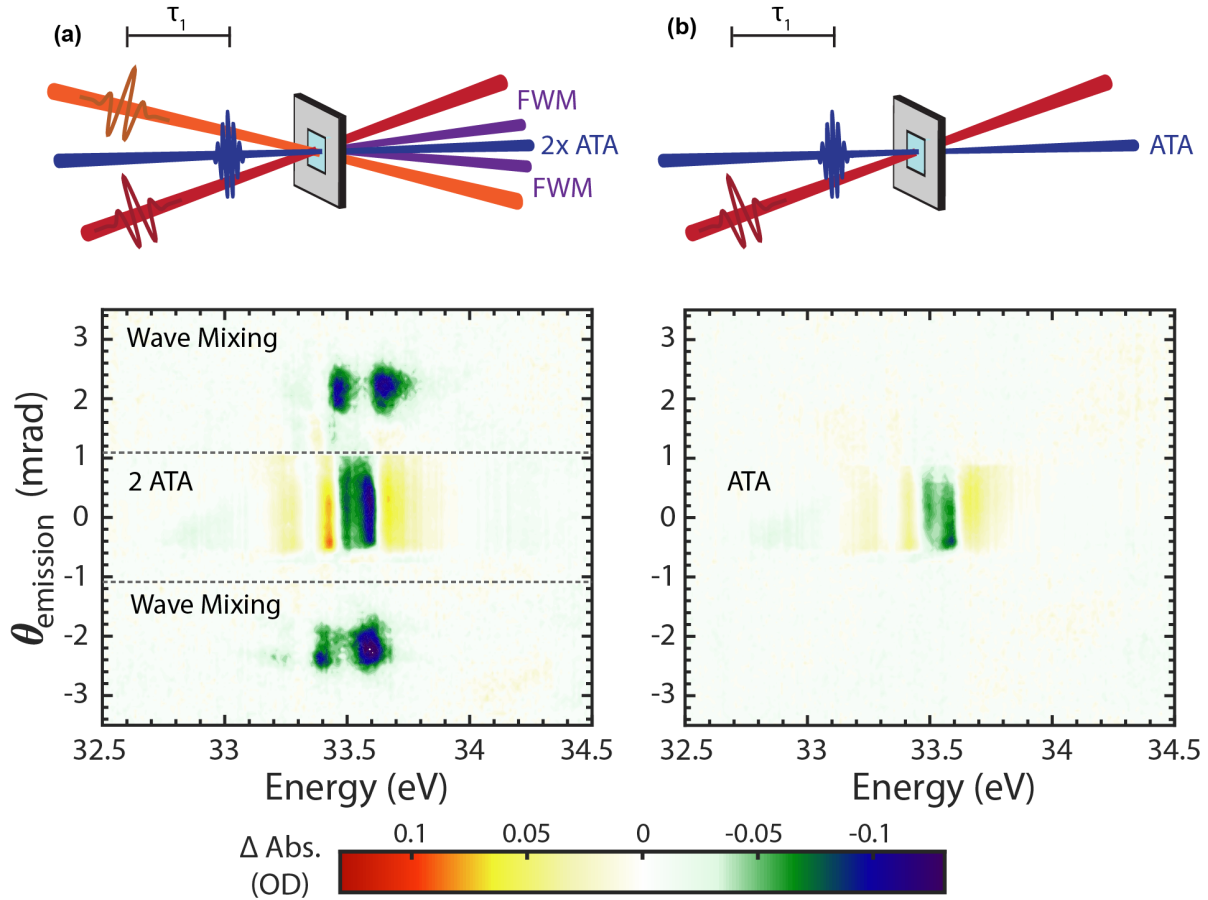
FIG. 3. XUV-NIR Nonlinear Wave Mixing Signal of \text{Na}^+ Core-Excitons in NaCl. (a) The \text{Na}^+ L_{2,3} core-exciton signal observed under the FWM experimental conditions (all beams unblocked, pulse sequence above) at temporal overlap ( \tau_1 = \tau_2 = 0 ). The background free FWM signals are observed at |\theta_{\text{emission}}| > 1 mrad while the ATA signals are found in the range -1 < \theta_{\text{emission}} < 1 mrad; negative \Delta\text{OD} indicates emission. (b) Confirmation of the nonlinear wave-mixing nature of the detected signals from blocking k_{\text{NIR}1} ; only the ATA signal from k_{\text{NIR}2} is observed as expected. To avoid detector saturation, the ATA signals are collected with 0.7 seconds integration while the FWM signals are collected with 2.0 seconds integration, resulting in the FWM signals shown in (A) effectively enhanced relative to the ATA signals by \sim 2.86 .
