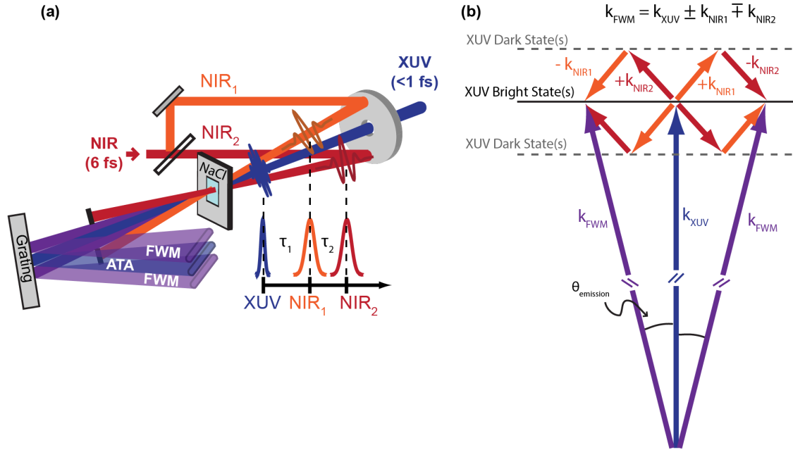
FIG. 2. Attosecond XUV-NIR Four-Wave Mixing Spectroscopy in a Noncollinear Beam Geometry. (a) Schematic of the beam geometry and pulse sequence. Two few-cycle NIR beams ( k_{NIR1}/NIR_1 , orange; k_{NIR2}/NIR_2 , red) are vertically stacked and crossed with an attosecond XUV pulse train ( k_{XUV}/XUV , blue) on the NaCl sample. The delays between each beam are independently tunable; the XUV-NIR delay is denoted \tau_1 and the delay between the two NIR pulses is \tau_2 . The wave-mixing signals ( k_{FWM} ) are emitted at an angle, \theta_{emission} , and the attosecond transient absorption signals are collinear with the XUV pulse. (b) The initially excited XUV-bright states are coupled through XUV-dark states and back to the bright state manifold through the two sequential NIR interactions. The phase-matching condition determines the emitted signal direction. Controlling the pulse timing determines whether the time-resolved XUV emission is determined by evolution of the XUV-bright states or the XUV-dark states.
