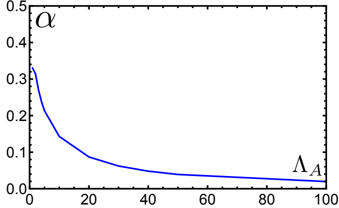
FIG. 17: Plot of the scaling dimension \alpha of the Amperean pairing vertex in the single patch critical theory with M/N = 1/2 , vs. the cutoff parameter \Lambda_A .
