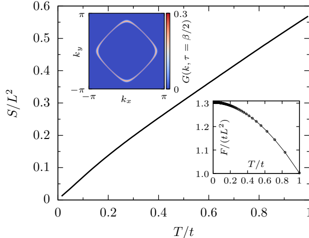
FIG. 4: Entropy density, S/L^2 , as a function of T at the QCP. We see it vanishes linearly as T \rightarrow 0 . The entropy is obtained by numerical differentiation of the free energy density, F/tL^2 , shown in the bottom inset. The top inset is G(k, \tau = \beta/2) , which is essentially the fermion spectral function averaged over an energy window of order T about the Fermi energy, for \beta t = 100 . We see the Fermi surface remains sharply defined at the QCP, in accord with Luttinger's theorem.
