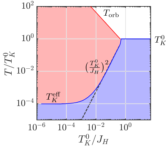
FIG. 9. Phase diagram obtained from a single iteration of the large- N equations, by solving Eq. (18), for q = 0.3 , D = 300 and T_K^0/D = 0.007 . The blue line is the solution T_K^{\text{eff}} , while the red line T_{\text{orb}} is obtained from the solution of Eq. (17) for a given s and J_H . The black dashed line corresponds to the scaling at intermediate T_K^0/J_H .
