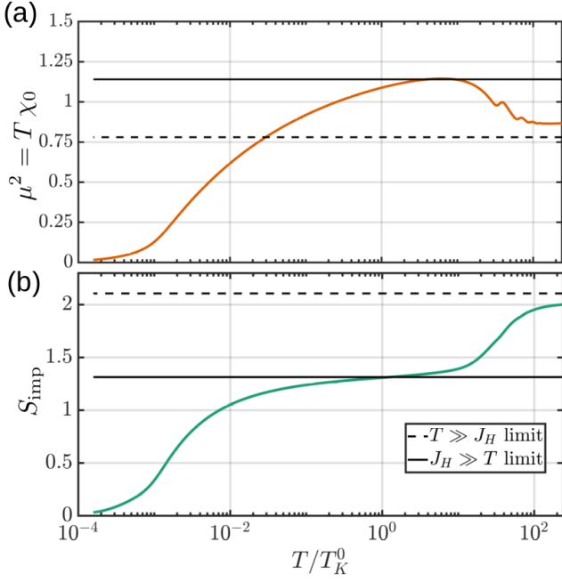
FIG. 4. (a) The impurity moment \mu^2 = T\chi_0 and (b) the entropy S_{\text{imp}} , respectively, as well as the two limits obtained analytically, as seen in Tab I. Parameters used were q = 0.3 and T_K^0/J_H = 0.07 .
