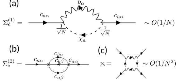
FIG. 10. (a) The electronic self-energy \Sigma_c^{(1)} = \frac{1}{N}G_\chi(-\tau)G_B(\tau) (we suppressed the orbital index m ) obtained from the Luttinger-Ward functional. (b) Next-order correction which includes inelastic scattering of the conduction electrons off the impurity, where vertices are represented in (c).
