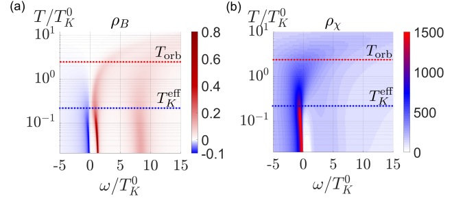
FIG. 6. (a) Temperature dependent Schwinger boson's spectral function and (b) holon's spectral function for the intermediate regime. In the locked moment phase, the low frequency peak moves downwards, finally settling into a constant value once T reaches T_K^{\text{eff}} \sim 0.22 T_K^0 . This leads to a clear gap in the bosonic and holon spectra at low frequency, while the high frequency spinon band remains. Parameters used were q = 0.3 and T_K^0/J_H = 0.08 , corresponding to a spinon gap of \Delta/T_K^0 = 3.3 .
