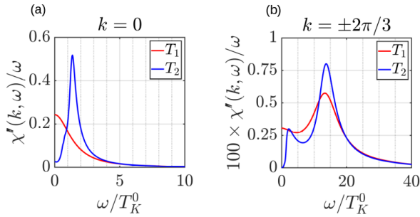
FIG. 7. Dynamical spin susceptibility \chi''(k, \omega)/\omega for temperature T_1 in the locked moment regime, and T_2 < T_K^{\text{eff}} in the Fermi-Liquid regime, for the uniform ( k = 0 ; a) and the staggered ( k = \pm 2\pi/3 ; b, enhanced by a factor of 100 for visibility) contributions. Parameters used were q = 0.3 and T_K^0/J_H = 0.08 , corresponding to a spinon gap of \Delta/T_K^0 = 3.3 .
