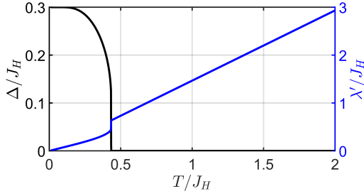
FIG. 8. Spinon gap \Delta (left) and modified spinon chemical potential \lambda' = \lambda - 2\Delta (right) obtained from equations (17), as a function of temperature. Parameters used were q = 0.3 .
