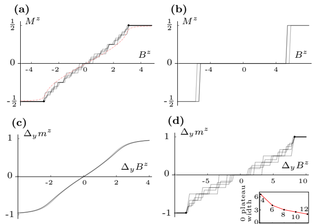
FIG. 1. Magnetization (a, b) and magnetization gradient (c, d) responses of a two-leg spin-1/2 ladder to an applied external magnetic field B^z and magnetic field gradient \Delta_y B^z respectively. In plots (a) and (c), the two-leg ladder is coupled via spin-anisotropic XY interactions that do not preserve subsystem symmetry, while the ladder in plots (b) and (d) is coupled via ring-exchange interactions that have subsystem symmetry. Additionally, for we include the magnetization response to a constant B^z of a chain that does not respect global U(1) S^z rotation symmetry, which is depicted as a dashed red line in (a). We superimposed numerical data for ladders with 4, 6, 8, 10, and 12 rungs. We clearly see that both magnetization and its gradient experience plateaus for the ring-exchange Hamiltonian, while there are no plateaus of magnetization gradient in the data for the XY-coupled ladder. In the magnetization gradient data for the ring-exchange model we see a small plateau at \Delta_y m^z = 0 that monotonically shrinks with increasing system size as shown by the inset plot. It is possible that this plateau will not survive the thermodynamic limit.
