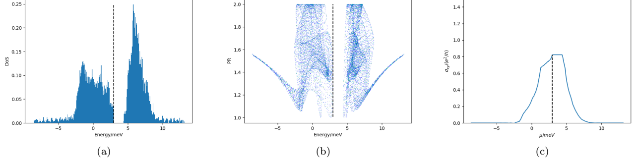
FIG. 13: Density of states, PR and \sigma_{xy} for \theta_G = 1.15^\circ and \theta_{BN} = -0.6^\circ
