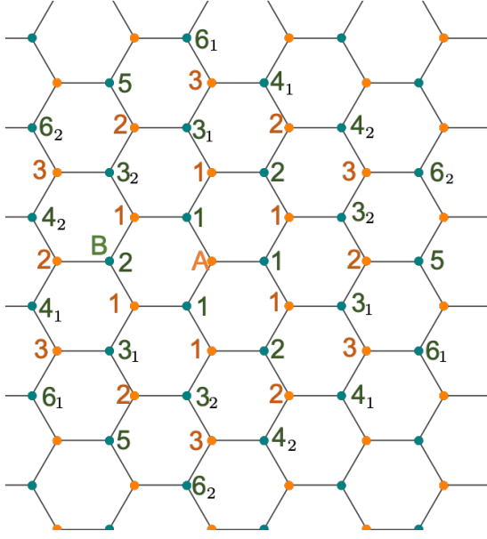
FIG. 5: Labels of the hopping terms from site A (orange circle) to other nearby sites. For example, hopping from A to an orange site labeled '2' corresponds to t_{2AA} and from A to a green site labeled 3_1 corresponds to t_{3AB1} .
