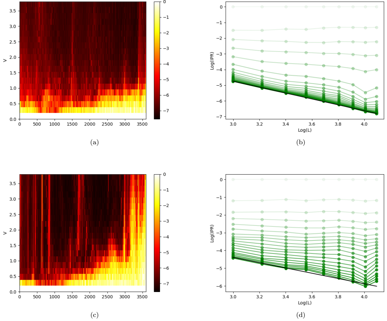
FIG. 14: IPR for single band model with dispersion. (a),(b): trivial case. (c),(d): non-trivial case. In (a)(b), \text{Log}(\text{IPR}) is plotted, x-axis labels different eigenstates in ascending order of their energies and y-axis labels different QP potential V from 0 to 4. The system size is 60 \times 60 . In (b)(d), green dots with different brightness connected by the same line label different QP potential V , from 0 to 4 (top to bottom), with 0.2 interval. The black line is the linear fitting for V = 4 . The linear system sizes are from 20 to 60.
