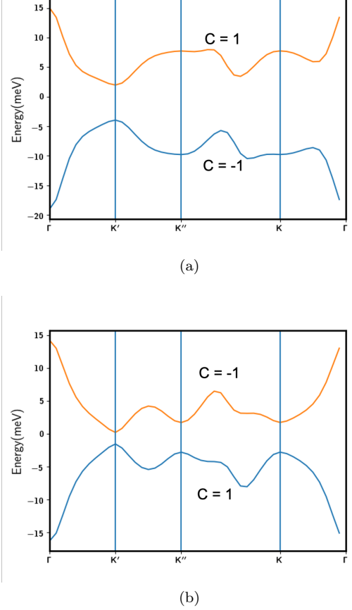
FIG. 3: Dispersion for (a)Case 1 and (b)Case 2. \theta_G = 1.2^\circ .
