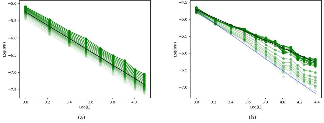
FIG. 15: IPR for single band model with non-uniform Berry curvature. (a): trivial( B_0 = 0 ) and (b): non-trivial( B_0 \approx 7.26 ). Green dots with different brightness connected by the same line label different B_1 , from 0 to 4 (top to bottom), with 0.2 interval. The black line in (a) is the linear fitting of the average IPR. The black line in (b) is the linear fitting of the average IPR for B_1 \geq 2 and the blue line in (b) is the linear fitting for B_1 = 0.2 .
