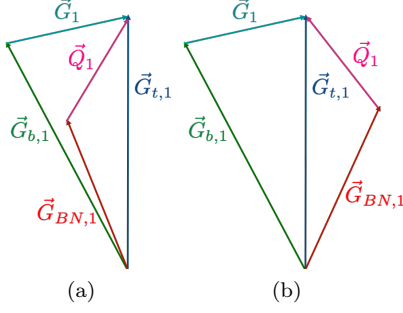
FIG. 1: (a) Case 1, \theta_{BN} > 0 and \theta_G > 0 . (b) Case 2, \theta_{BN} < 0 and \theta_G > 0 . The angles are exaggerated for illustration purpose.
