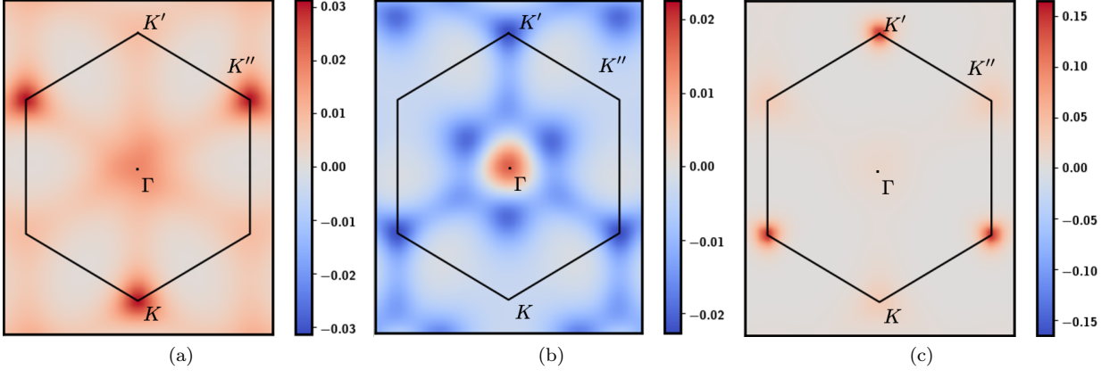
FIG. 4: Berry curvature distribution of valence band for (a) m_z only (b) Case 1 and (c) Case 2. \theta_G = 1.2^\circ . The black line is the boundary of the first BZ and the black dot is the \Gamma point.
