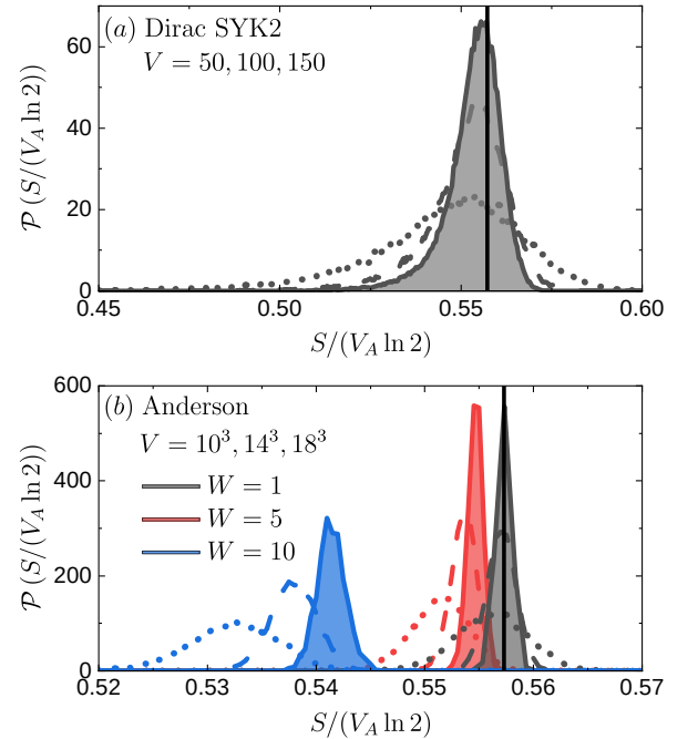
FIG. 3. Distributions of the von Neumann eigenstate entanglement entropies for (a) the Dirac SYK2 model (8), and (b) the 3D Anderson model (11) with W = 1, 5 , and 10 . The vertical lines mark the analytical prediction [Eq. (7)]. We show results for lattices with: (a) V = 50, 100 , and 150 , and (b) V = 10^3, 14^3 , and 18^3 , using dotted, dashed, and solid lines, respectively. The results in (a) were obtained using at least 10^5 randomly selected eigenstates, in each of the 500 Hamiltonian realizations over which we average. The results in (b) were obtained for 10^4, 10^3 , and 10^2 randomly selected eigenstates in each of the 100, 10, and 5 Hamiltonian realizations for V = 10^3, 14^3 , and 18^3 , respectively.
