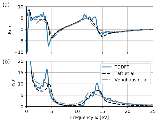
FIG. 2. Dielectric function of a crystalline graphite in the direction parallel to the layer : (a) real part \text{Re}\epsilon_{zz} and (b) imaginary part \text{Im}\epsilon_{zz} . The experimental spectra are also plotted as black [56] and gray [57] broken curves.
