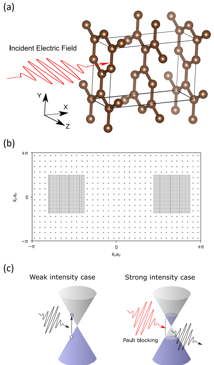
FIG. 1. Schematic illustration of a calculated system: (a) Linearly polarized electric field irradiates normally on an ABA-stacked graphite crystal for which we use a rectangular unit cell with 8 carbon atoms. (b) Non-uniform k -point distribution to sample the entire BZ that contains 1,656 coarse points and 6,272 dense points. (c) Band structure and electron occupation in the weak (left) and strong (right) field cases.
