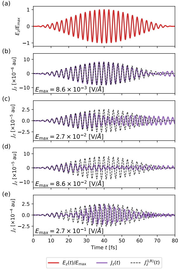
FIG. 3. Applied electric field (a) and induced current density (b-e) for four different maximal field amplitudes E_{\max} . The central frequency and the pulse duration are set to \omega_1 = 1.55 eV and T_P = 80 fs, respectively. In (b – e), purple lines show calculated current density using Eq. (5). Black broken-line shows the linear results with \sigma = 0.047 - 0.018i au.
