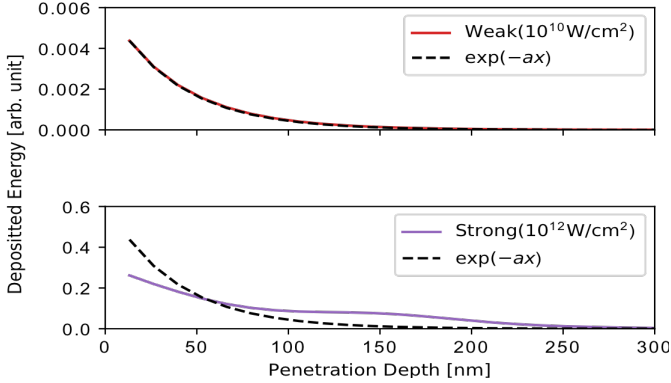
FIG. 11. Energy deposition as a function of distance from the surface. (a) for weak pulse and (b) for strong pulse cases.
