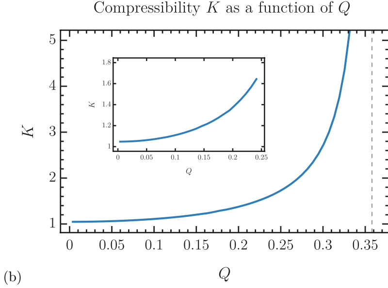
FIG. 11: (a) Charge as a function of the chemical potential for the fermionic SYK at zero temperature. The blue line is the numerical solution of the Schwinger-Dyson equations (E7) - (E13) for the fermionic SYK at zero temperature for different values of the asymmetry angle. There is a maximal value of the chemical potential at which the value of the charge Q_{\max} \simeq 0.358 . (b) Compressibility K as a function of charge for the fermionic spinon model at zero temperature (here we set J = 1 ). Compressibility diverges at Q_{\max} \simeq 0.358 ( \theta_f \simeq 0.153\pi ). Inset: compressibility growth as small Q .
