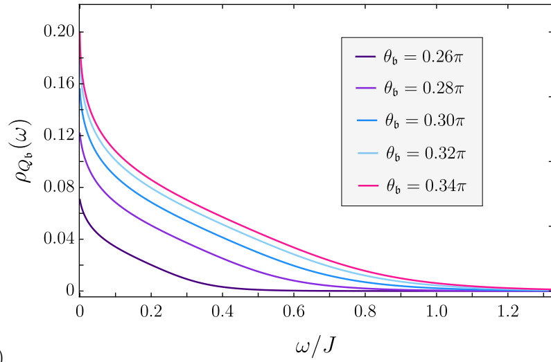
FIG. 15: Plots of the numerically computed spin spectral densities (7.12) for (a) fermionic and (b) bosonic spinon models at different values of asymmetry angles.
