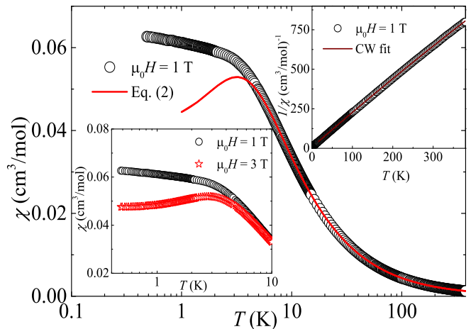
FIG. 3. \chi of polycrystalline \text{BaNa}_2\text{Cu}(\text{VO}_4)_2 sample as a function of temperature in an applied field \mu_0 H = 1 \text{ T} . The solid line is the fit using Bonner-Fisher model [Eq. (2)] for uniform Heisenberg spin-1/2 chain. Upper inset: inverse susceptibility 1/\chi vs T and the solid line represents the CW fit, as discussed in the text. Lower inset: the low-temperature \chi(T) measured in two different fields \mu_0 H = 1 \text{ T} and 3 T.
