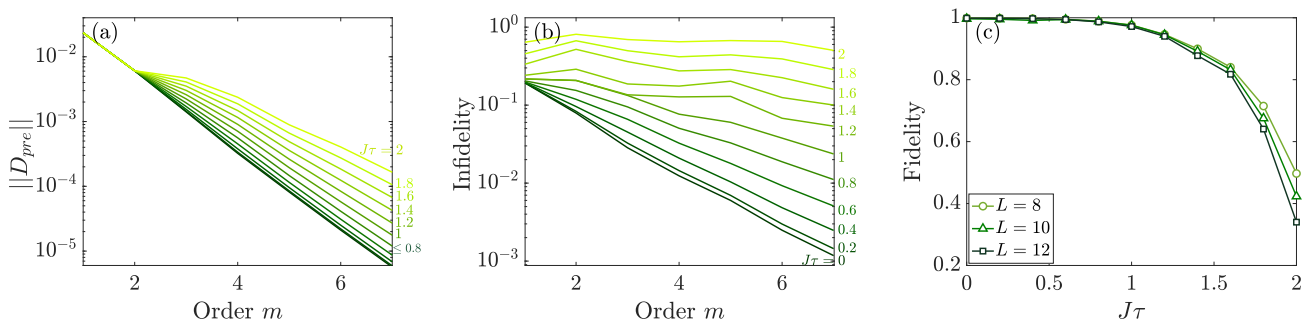
FIG. 4. D_{pre} expansion of KDM. (a) Norm of the m^{\text{th}} order term of the quasiconserved observable D_{pre} (normalized by L^2L ). Different curves stand for h\tau = J\tau from 0 to 2 in steps of 0.2. Darker color represents smaller J\tau . (b) Infidelity 1 - \langle D_{pre}(\infty)D_{pre} \rangle of infinite-time averaged D_{pre} evaluated up to m^{\text{th}} order. L = 12 is used. (c) Fidelity \langle D_{pre}(\infty)D_{pre} \rangle evaluated to 7^{\text{th}} order as a function of h\tau for different system sizes.
