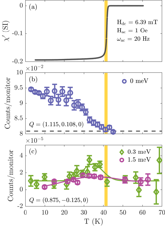
Figure 1. a) The real part of AC magnetic susceptibility, \chi' , showing the sharp transition to a diamagnetic state upon cooling below the superconducting critical temperature. T_c is indicated by the yellow stripe which spans a temperature range 41.3 \pm 0.8 \text{ K} . The steps followed in the conversion from emu to SI units are presented in Appendix A. b) Temperature dependence of magnetic order measured as 1-point scans on top of one of the IC peaks (1.115, 0.108, 0) . The incoherent background has not been subtracted. The dashed line indicates the background level extracted from an energy scan taken away from the incommensurate peak position, at (1.1, -0.24, 0) . c) Temperature dependence of magnetic fluctuations with energy 0.3 meV and 1.5 meV. Data were measured as 3-points scans with k_f = 1.2 \text{ \AA}^{-1} ( \Delta E = 0.070(1) \text{ meV} )
