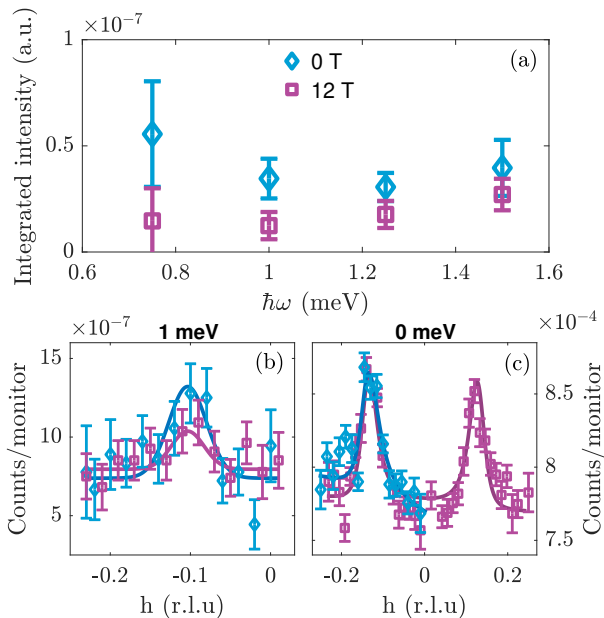
Figure 3. a) Magnetic field dependence of low-energy spin excitations measured at 2 K. Representative b) inelastic constant energy scan ( \hbar\omega = 1 meV) and c) elastic scans collected in the superconducting phase (2 K) with and without applied magnetic field. The solid lines are Gaussian fits to the raw data.
