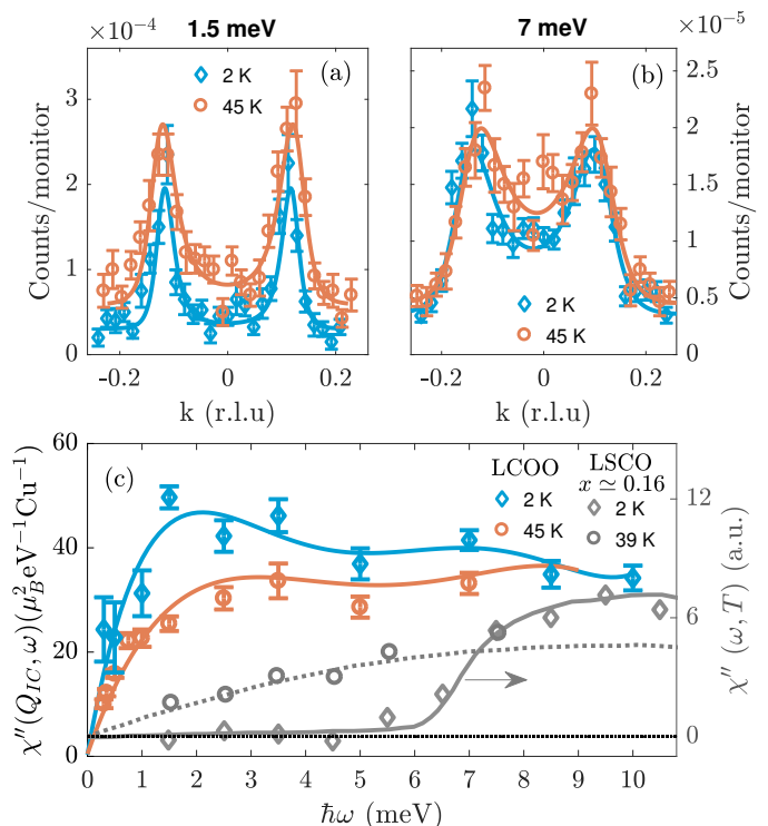
Figure 2. a) and b) Representative inelastic scans through the incommensurate positions (\pm\delta, 1 - \delta, 0) where \delta = 0.125 , collected at 1.5 meV and 7 meV with fixed outgoing wavevectors k_f = 1.55 \text{ \AA}^{-1} and k_f = 1.5 \text{ \AA}^{-1} , respectively. The data were collected at ThALES (a) and IN12 (b) at two temperatures: blue diamonds show data in the superconducting state (2 K) and orange circles show data within the normal state (45 K). The solid lines are Sato-Maki function fits to the raw data as described in the text. c) Dynamic susceptibility \chi''(\mathbf{Q}_{\text{IC}}, \omega) measured inside (2 K - in blue) and outside (45 K - in orange) the superconducting dome. Solid lines are guides to the eye. Each data point represents an average of values obtained at different k_f values and on different instruments (ThALES and IN12). In grey symbols, we show for comparison the magnetic susceptibility measured inside and outside the superconducting state by B. Lake et al. 33 on an optimally doped x = 0.163 LSCO sample.
