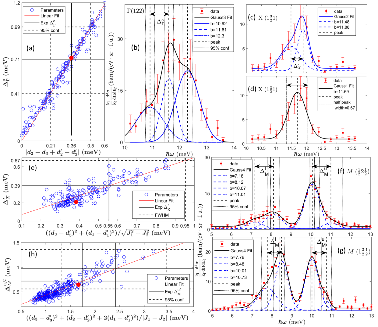
FIG. D4: (a) The linear dependence of the optical mode splitting at the \Gamma point \Delta_{\Gamma}^0 on |d_2 + d'_2 - d_3 - d'_3| . The linear fit is y = ax + b with a = 0.45(2) , b = -0.03(3) meV, with R^2 = 0.85 . (b) Excitation spectrum at the \Gamma point which provides experimental evidence for \Delta_{\Gamma}^0 with 95% confidence range shown. (c,d) 2-gaussian and 1-gaussian fits of the upper modes at the X point around 12 meV. The splitting \Delta_X' is defined in (c). (e) The linear correlation of \Delta_X' and the quantity D_X defined in Sec. D 2 c(2). The linear fit is y = ax + b with a = 0.70(6) , b = 0.00(3) meV, with R^2 = 0.71 . (f,g) 4-gaussian fit of two different M point spectra, from which we obtain \Delta_M^{u/l} = 0.97(39) meV and \Delta_M^{l/u} = 0.7(2) meV, respectively. (h) The linear correlation of \Delta_M^{u/l} and the quantity D_M defined in Sec. D 2 c(3). The linear fit is y = ax + b with a = 0.45(2) , b = -0.03(3) meV, with R^2 = 0.85 . In (a,e,h), we have marked the optimal set of parameters in Table I by the red solid symbol. Error bars in all figures represent one standard deviation. In (b-d,f,g), red symbols show neutron intensity data averaged over (0.1 \text{ \AA}^{-1})^3 \times (0.2 \text{ meV}) in the 4D \mathbf{Q} - \hbar\omega space.
