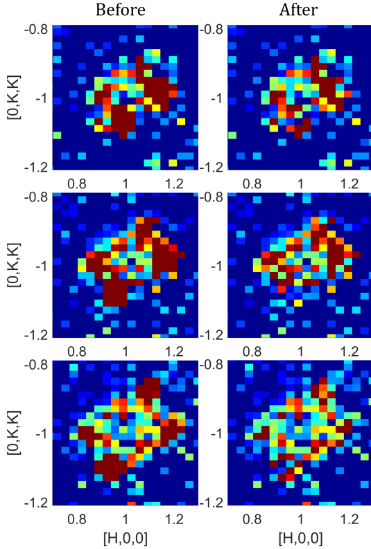
FIG. D6: (a-c) Constant energy slices of MACS data at energy transfers \hbar\omega = (a) 0.40(5), (b) 0.50(5), (c) 0.60(5) meV before the "spurious" subtraction, respectively. (d-f) Constant energy slices at energy transfers \hbar\omega = (d) 0.40(5), (e) 0.50(5), (f) 0.60(5) meV after removing the Bragg "spurious", respectively.
