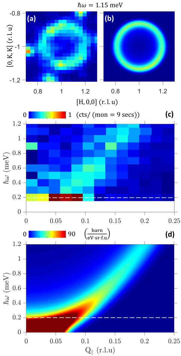
FIG. 3: (a) Constant \hbar\omega = 1.15(15) meV slice through MACS data near the \mathbf{Q}_0 = (\bar{1}\bar{1}\bar{1}) zone center. The spinwave signal forms a circle, which indicates isotropic dispersion. (b) Spinwave model calculation using the parameters in Table. I and numerically convoluting with the instrumental resolution described in Appendix E. (c) Q_{\parallel} - \omega intensity map of MACS data following azimuthal averaging around \mathbf{Q}_0 . Due to the azimuthal averaging, the errorbars of the pixels are inversely proportional to Q_{\parallel} ; The pixels near Q_{\parallel} = 0 (for example, bright pixels at \hbar\omega = 0.4, 0.6, 0.9 meV) have significantly larger errorbars compared to the pixels of finite Q_{\parallel} and are thus less reliable. (d) Calculated Q_{\parallel} - \omega intensity map using parameters in Table. I and the same azimuthal averaging as for the experimental data. Data in (a,c) shares the same color scal and was not independently normalized. Calculation results in (b,d) share the same normalized color scale. Dashed lines in (c,d) marks the lowest accessible energy transfer (0.2 meV) in the MACS experiment.
