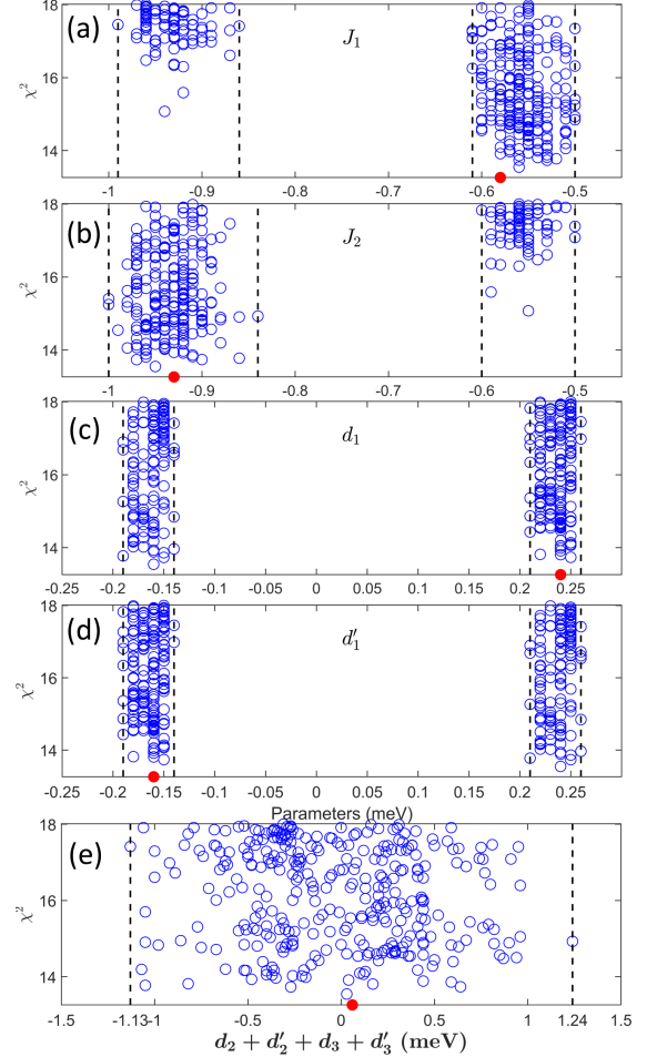
FIG. D3: The projections of the goodness of fit \chi^2 on the parameter axis for (a) J_1 , (b) J_2 , (c) d_1 , and (d) d'_1 . Each blue circle represents one set of parameters with low \chi^2 . The red circle shows the optimal set of parameters listed in Table I, the dashed lines show the bounds in these parameters inferred from the \chi^2 plots. (e) The projection of \chi^2 on the parameter axis d_2 + d_3 + d'_2 + d'_3 .
