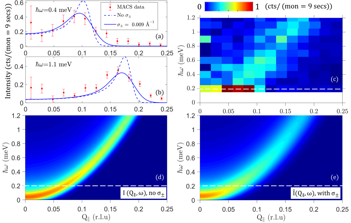
FIG. E7: (a,b) Constant energy cut of MACS data and the best fitted \tilde{I}(Q_{\parallel}, Q_{\perp} = 0, \omega) ( D = 67(8) \text{ meV \AA}^2 and \Delta_{\Gamma} = 0.0(1) \text{ meV} ) at \hbar\omega = 0.4, 1.1 \text{ meV} , respectively. \tilde{I}(\mathbf{Q}, \omega) has taken into account the average out-of-plane Q-resolution \sigma_{Q_{\perp}} = 0.07 \text{ \AA}^{-1} , the energy resolution \sigma_{\omega} = 0.05 \text{ meV} , the in-plane Q-resolution \sigma_{Q_{\parallel}} = 0.004 \text{ \AA}^{-1} . Both I(\mathbf{Q}, \omega) (Eqn. E1) and \tilde{I}(\mathbf{Q}, \omega) (Eqn. E2) with the extra broadening by \sigma_{\pm} (representing the presence of incommensurate modes) are plotted. The relatively better agreement of the \tilde{I}(\mathbf{Q}, \omega) (solid line) with the MACS data shows that we have observed the incommensurate nature of spinwave modes. (c) Q_{\parallel} - \omega intensity map of MACS data following azimuthal averaging around \mathbf{Q}_0 (the same as Fig. 3(c)). (d,e) Simulated I(Q_{\parallel}, \omega) and \tilde{I}(Q_{\parallel}, \omega) with the parameters and resolutions specified as in (a,b). Dashed lines in (c,d,e) marks the lowest accessible energy transfer (0.2 meV) in the MACS experiment. Error bars in (a,b) represent one standard deviation.
