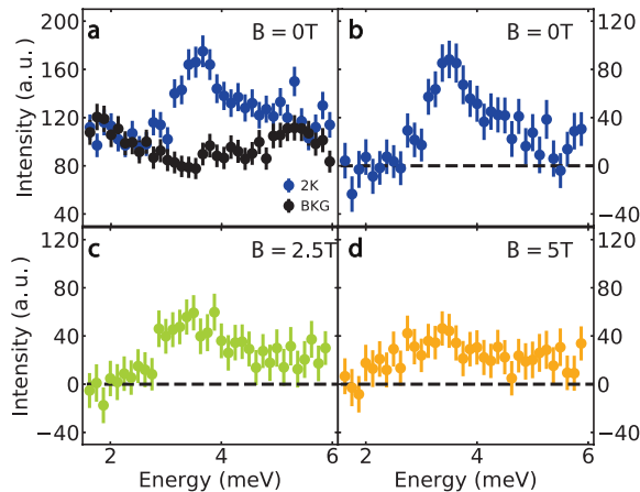
FIG. 4: (a) Constant- Q scans at Q_{AF} and the off-peak background positions at 2 K in zero field as shown in Fig. 1(d). (b)-(d) Constant- Q scans with background subtracted in 0, 2.5 and 5 T c -axis aligned fields. The error bars indicate statistical errors of 1 standard deviation.
