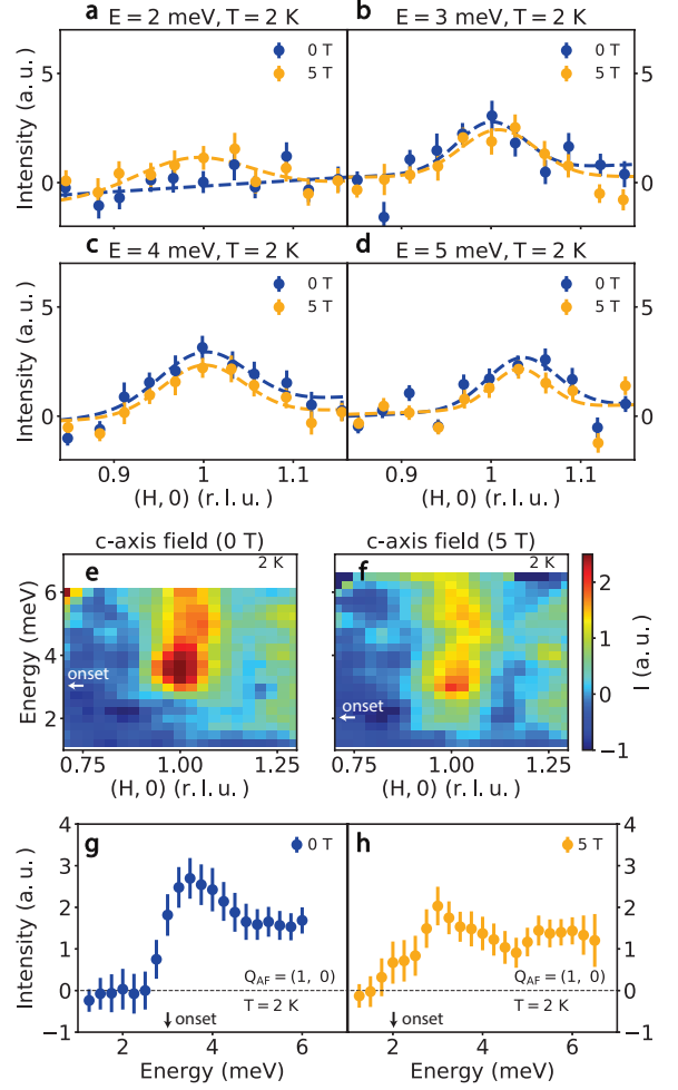
FIG. 3: (a)-(d) Constant-energy scans along the [1, 0] direction at E = 2, 3, 4 and 5 meV in zero and 5 T c -axis aligned magnetic fields at T = 2 K. (e) and (f) 2D images of wave-vector and energy dependence of the resonance in zero and 5 T magnetic fields at T = 2 K. The background subtraction process is similar to that of Fig. 2 59 . (g) and (h) are constant- \mathbf{Q} cuts at the \mathbf{Q}_{AF} position from (e) and (f), respectively. They have been smoothed two times by the 2D data processing method in David-Mslice program at NCCR. The arrows in (e), (f), (g), and (h) indicate the lowest energy where a Gaussian can be fit to the data. The error bars indicate statistical errors of 1 standard deviation.
