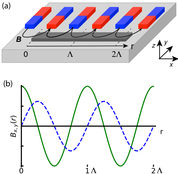
FIG. 1. (a) A schematic representation of the system geometry. Here, the nanowire (dark-grey rectangle) is in proximity with a superconductor (grey rectangle). Nanomagnets with alternating magnetization are arranged nearby (blue-red rectangles), in the same plane as the wire. Alternatively, the nanomagnets can be positioned higher than the nanowire, which could improve the shape of the magnetic field for our purposes 51 . (b) Components of the spiral magnetic field, B_x = B_{x0} \cos(2\pi r/\Lambda) (solid line) and B_y = B_{y0} \sin(2\pi r/\Lambda) (dashed line) in the nanowire, with period \Lambda , as a function of position along the wire, r . For an ideal helical field, we have B_{y0} = B_{x0} . Here, we show the case of an elliptic helical field, with B_{y0} = 0.62B_{x0} .
