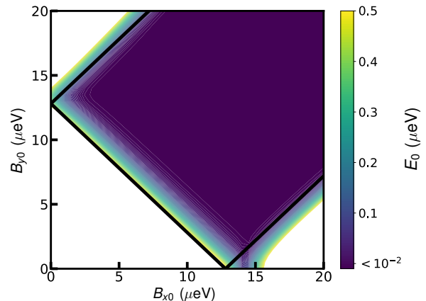
FIG. 6. Contour plot of the lowest positive energy E_0 of the system in the plane of magnetic field amplitudes B_{x0} and B_{y0} for the chemical potential \mu = \hbar^2 Q^2/8m + \delta\mu with \delta\mu = 4 \mu\text{eV} . Here, the superconducting pairing energy \Delta = 5 \mu\text{eV} , and the wire length L = 20 \mu\text{m} . The region with energy E_0 above 0.5 \mu\text{eV} corresponds to the gapped non-topological superconducting phase and is shown as unfilled parts of the B_{x0} - B_{y0} plane. The solid straight lines represent the analytical expressions (33) for the phase boundaries derived for linearized bands and an infinite length wire. In wires of finite length, the zero energy state develops over finite crossover region shown as transition colors in the color plot for the region of E_0 < 0.5 \mu\text{eV} , the dark purple color shows area where E_0 drops below 10^{-2} \mu\text{eV} .
