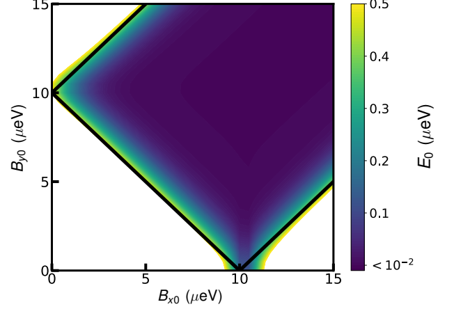
FIG. 3. Contour plot of E_0 , the energy of the state of lowest positive energy in the system, versus the magnetic field amplitudes B_{x0} and B_{y0} . Parameter values used are: superconducting order parameter \Delta = 5 \mu\text{eV} , magnetic field wavevector Q = 2\pi/\Lambda , \Lambda = 200 \text{ nm} , chemical potential \mu = \hbar^2 Q^2/8m = 49.6 \mu\text{eV} , and wire length L = 20 \mu . The uncolored region where E_0 > 0.5 \mu\text{eV} corresponds to the gapped non-topological superconducting phase, the dark purple color denotes the region in which E_0 < 10^{-2} \mu\text{eV} , and the crossover region over which the zero energy state develops in this wire with finite length is evident in the transitions between colors in the color plot for the region of E_0 < 0.5 \mu\text{eV} . The solid straight lines show the analytical predictions for the phase boundary given by Eq. (21).
