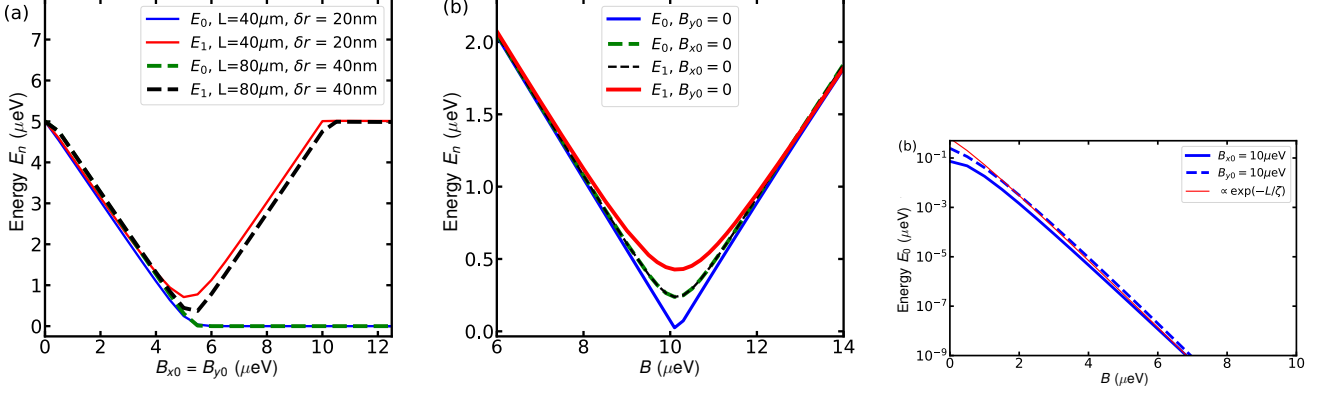
FIG. 4. Comparison of two lowest-energy excitation energies E_0 and E_1 in non-topological and topological phases as a function of magnetic field magnitude. (a): Energies E_0 and E_1 versus the magnetic field amplitude B_{x0} = B_{y0} in wires evaluated for different wire lengths, solid lines: L = 40 \mu\text{m} and \delta r = 20\text{nm} ; dashed lines: L = 80 \mu\text{m} and \delta r = 40\text{nm} . In the topologically nontrivial phase, E_0 approaches zero for when B_{x0} = B_{y0} is large. The second excitation energy E_1 reaches its minimum at the phase transition, where the gap in the density of states closes in the infinitely long wire, and then increases as the magnetic field is increased further. (b): Energies of the lowest two excitations as a function of one component of the field, B_{x0} = B (solid lines) or B_{y0} = B (dashed lines), while the other component is strictly zero, B_{y0} = 0 or B_{x0} = 0 , respectively. When one field component is zero, the magnetic field has no helicity and no topologically protected state can form. All the excitation energies show minima at B \simeq 2\Delta = 10 \mu\text{eV} and then all energies increase as B is increased further. When B_{x0} = 0 and the magnetic field is zero at the ends of the wire, E_0 = E_1 , but the energies E_0 and E_1 are split near B_{x0} = 2\Delta when the field at the ends is not zero ( B_{y0} = 0 case). (c): Energies of the lowest energy excitations as a function of one component of the magnetic field when the other component is fixed at twice the superconducting gap \Delta , either B_{x0} = B , B_{y0} = 2\Delta or B_{y0} = B , B_{x0} = 2\Delta . For both cases, the energy of the lowest energy state monotonically decreases towards zero as B increases, while all other excitation energies increase as the superconducting gap opens, consistent with a topologically nontrivial phase. For all these plots, the proximity-induced superconducting order parameter \Delta = 5 \mu\text{eV} , and the chemical potential \mu = \hbar^2 Q^2 / 8m = 49.6 \mu\text{eV} is matched to the middle of the magnetic superlattice gap. For panels (b) and (c), the wire length is L = 40 \mu\text{m} .
