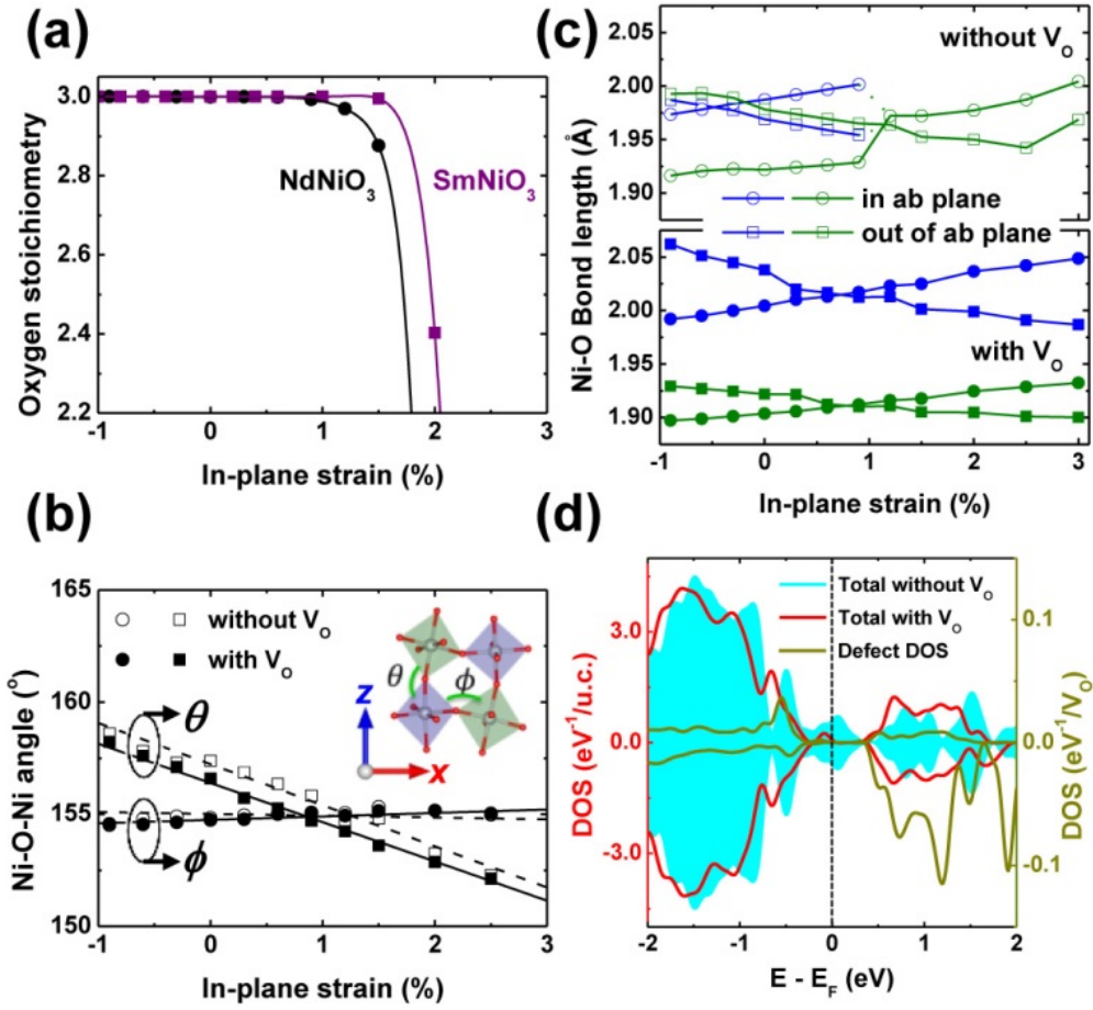
FIG. 1 (color online). (a) Strain-dependent oxygen stoichiometry in \text{NdNiO}_3 (solid circles) and \text{SmNiO}_3 (solid squares). The stoichiometry is calculated at room temperature and thermal equilibrium with \text{O}_2 molecule. The lines are guides to the eye for the data points. (b) Calculated octahedral tilt ( \theta ) and rotation ( \phi ) angles as a function of in-plane strain. The inset shows a Pbnm \text{NdNiO}_3 unit cell indicating the angles \theta and \phi . The tilt angle \theta and rotation angle \phi represent the Ni-O-Ni bonding angles with respect to the z axis and in the xy in-plane, respectively. In (b), open (filled) symbols represent the quantities in the absence (presence) of oxygen vacancies. (c) Calculated shorter (green) and longer (blue) Ni-O bond lengths in a-b plane (circle) and c plane (square) in absence (open symbol) and presence (filled symbol) of oxygen vacancy. Note that the difference between the shorter and longer Ni-O bondings increases in presence of oxygen vacancy. (d) Total and local density of states (DOS) in \text{NdNiO}_3 projected at the defect sites in the presence (lines) and absence (cyan background) of oxygen vacancies. Note a band gap for the oxygen-deficient \text{NdNiO}_3 .
