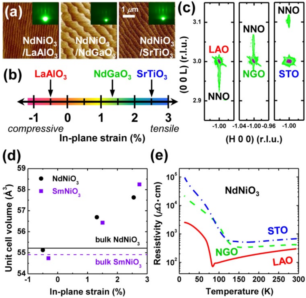
FIG. 2 (color online). (a) AFM topography images of the as-grown 14-nm-thick (left) NdNiO 3 /LaAlO 3 (LAO), (middle) NdNiO 3 /NdGaO 3 (NGO), and (right) NdNiO 3 /SrTiO 3 (STO) thin films, where the insets represent the corresponding RHEED patterns. (b) In-plane biaxial strain of NdNiO 3 with respect to pseudocubic LAO, NGO, and STO (001) substrates. (c) (-103) RSMs of pseudocubic NdNiO 3 (001) films. All of the RSMs are on the same scale in the H and L directions. All NdNiO 3 films are coherent with respect to the substrates. (d) The strain-dependent pseudocubic unit-cell volumes of epitaxial NdNiO 3 (solid circles) and SmNiO 3 (solid squares) films. The solid and dashed lines represent the unit-cell volume of bulk NdNiO 3 and SmNiO 3 in pseudocubic notation, respectively. (e) The temperature-dependent resistivity in the 14-nm-thick NdNiO 3 (001) films.
