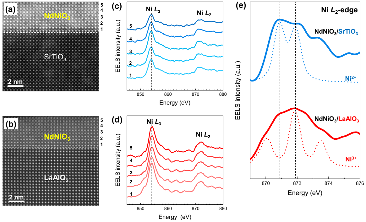
FIG. 3 (color online). STEM-high angle annular dark field (HAADF) images of the 10-unit-cell-thick NdNiO 3 (3.8 nm) films grown on (a) STO and (b) LAO substrates along the pseudocubic [100] zone axis. (c,d) EELS spectra of Ni L_{2,3} -edges obtained across the NdNiO 3 films shown in (a) and (b), respectively. Black dashed and gray dotted lines are guidelines for Ni L_3 . (e) The Ni L_2 -edges of the NdNiO 3 /STO (the blue solid line) and NdNiO 3 /LAO (the red solid line) films in (c) and (d), respectively. A comparison with the EELS calculation spectra of Ni 2+ (blue dashed line) and Ni 3+ (red dashed line) evidences that the oxidation states of Ni in 10-unit-cell-thick NdNiO 3 films grown on STO and LAO substrates are more towards Ni 2+ and Ni 3+ , respectively. For Ni 2+ , two distinct peaks (870.8 and 871.9 eV) was calculated with the estimated crystal field splitting parameter, 10 Dq , 1.1 eV, while three peaks (870.1, 871.9, and 873.8 eV) with higher 10 Dq , 1.8 eV was found in the Ni 3+ state.
