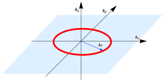
Figure 1. Ring of nodal points in the k_z = 0 plane resulting from the spectrum of the free Hamiltonian (2). The light blue shaded region represents the plane of the nodal line. Nodal loop of radius k_F is shown in red.
