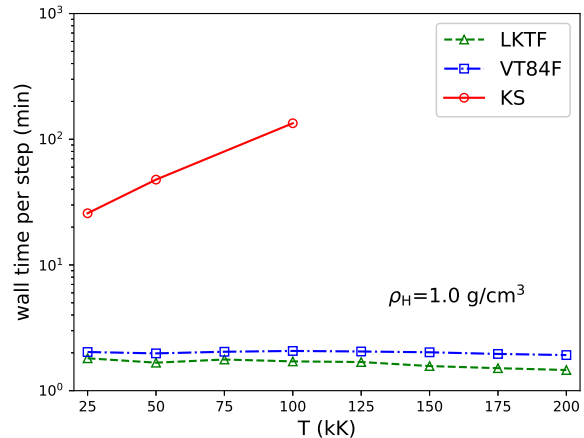
FIG. 1. Average WALL time per MD step as a function of T for ordinary KS-AIMD, and OF-AIMD with VT84F, and LKTF functionals. Hydrogen density is \rho_H = 1.0 \text{ g/cm}^3 . The KS cost grows while the LKTF and VT84F cost per step is T-independent. As noted before, at T = 0 K, LKT SCF convergence is faster than VT84F.
