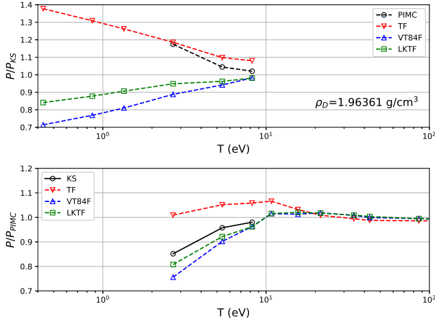
FIG. 7. Relative pressures versus temperature for D at \rho_D=1.96361 ( r_s = 1.4 bohr) from PIMC, KS, LKTF, VT84F, and TF. Upper panel is relative to KS pressures, lower is relative to PIMC pressures.
