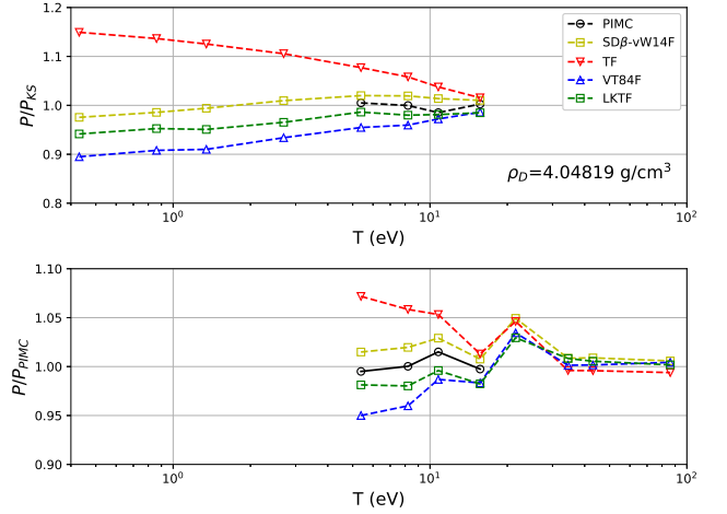
FIG. 8. As in Fig. 7 for D at \rho_D=4.04819 g/cm ^3 ( r_s=1.1 bohr) and with SD\beta -vW14F data as well.
