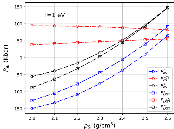
FIG. 4. Comparison of electronic pressure contributions from LKTF and conventional KS calculations for static cd Si at T = 1 eV. Superscript \mathcal{E} denotes internal energy contribution, TS, the entropic contribution, and \mathcal{P} the total.
