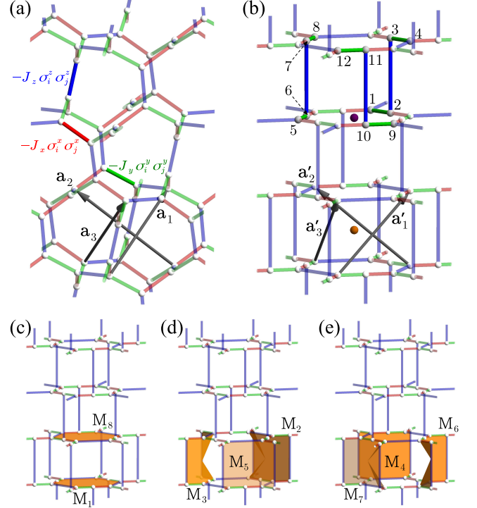
FIG. 1. Schematic pictures of the Kitaev model on the hypernonagon lattice. (a) The original hypernonagon lattice 28 and (b) the distorted one for better visibility 21 . \mathbf{a}_1 , \mathbf{a}_2 , and \mathbf{a}_3 ( \mathbf{a}'_1 , \mathbf{a}'_2 , and \mathbf{a}'_3 ) are the primitive translation vectors for the original (deformed) lattice. The white spheres represent the lattice sites on which the spin-1/2 degrees of freedom are defined. The red, green, and blue bonds denote the x , y , and z bonds of the Kitaev model in Eq. (1), respectively. A unit cell contains 12 sites, as indicated by the numbers 1–12 in (b). Two types of inversion centers are denoted by orange and purple spheres in (b). (c)–(e) The eight types of plaquettes M_p ( p = 1 –8) in a unit cell on which the \mathbb{Z}_2 fluxes W_p in Eq. (2) are defined. Each plaquette consists of 9 sites.
