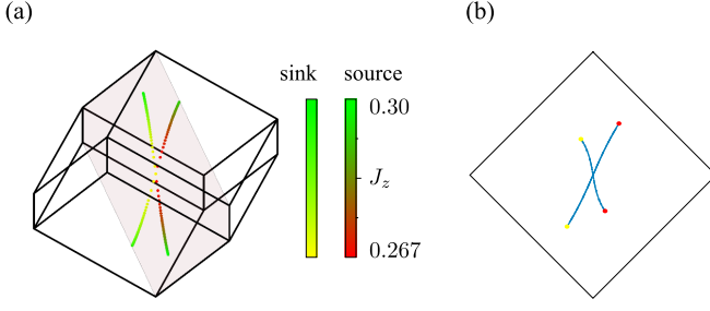
FIG. 7. Gapless SI phase. (a) Evolution of Weyl nodes for coupling constants 0.267 \leq J_z \leq 0.30 with J_x = J_y = (1 - J_z)/2 . The sink and source indicate the negatively- and positively-charged Weyl nodes, respectively. The shaded region indicates the remaining mirror plane in the SI phase with J_x = J_y . (b) Corresponding Fermi arcs on the 001-surface Brillouin zone for (J_x, J_y, J_z) = (0.36, 0.36, 0.28) .
