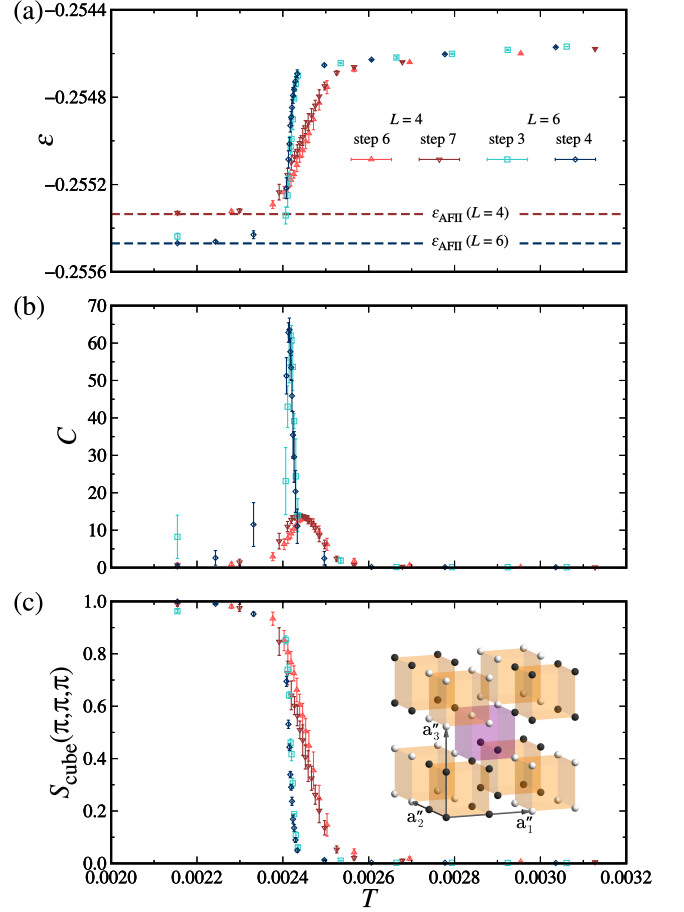
FIG. 4. Low- T phase transition. Shown are the T dependence of (a) the internal energy \varepsilon and (b) the specific heat C as given in Figs. 3(a) and 3(b), respectively, but plotted on a linear T scale, zooming in the low- T regime (the gray areas in Fig. 3). (c) The order parameter for the \mathbb{Z}_2 flux ordering, S_{\text{cube}}(\mathbf{Q}) at \mathbf{Q} = (\pi, \pi, \pi) at the last two optimization steps. The inset of (c) indicates the flux configuration in the low- T CSL phase, where black and white spheres represent fluxes with W_p = +i and -i , respectively. \varepsilon_{\text{AFII}} in (a) indicates the ground state energy for each system size. See the main text for details.
