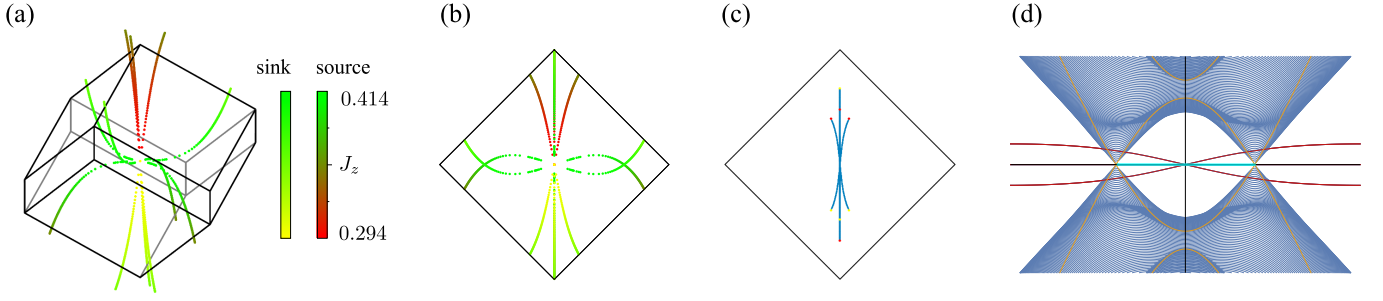
FIG. 10. Evolution of Weyl nodes for coupling constants 0.294 \leq J_z \leq 0.414 with J_x = J_y = (1 - J_z)/2 in (a) the bulk Brillouin zone and (b) projected down to the 001-surface Brillouin zone, respectively. The two Weyl nodes on the C_3 -invariant axis are not shown for clarity. (c) Corresponding Fermi arcs in the 001-surface Brillouin zone for (J_x, J_y, J_z) = (0.345, 0.345, 0.31) . This includes the Weyl nodes which lie on the C_3 -invariant axis along with their corresponding Fermi arc. (d) Band structures for J_z = 0.46 . The bulk band structure along the C_3 -invariant axis is plotted in yellow showing the two Weyl nodes. The band structure for the slab geometry along the projection of the C_3 axis to the surface Brillouin zone is plotted in blue and red. The projection of the two Weyl nodes as well as the Fermi arc which connects them are colored blue. The bands responsible for the remaining surface states left over from the other Weyl nodes, which are gapped out for J_z \approx 0.414 , are colored red.
