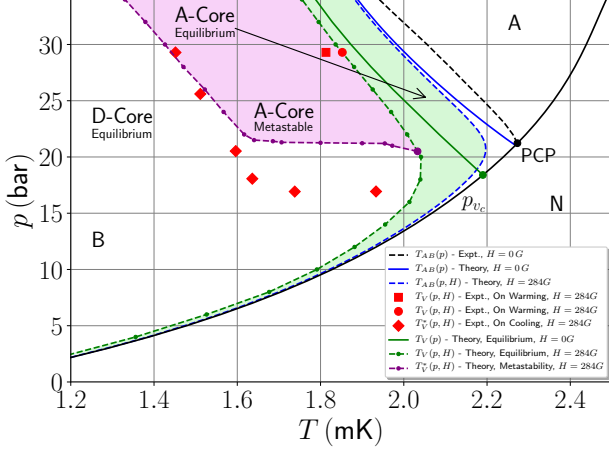
FIG. 1. The vortex core transition line, T_V(p, H) , for H = 0 G (solid green) separating the A-core and D-core vortex phases of ^3\text{He-B} terminates at a triple point (p_v, T_v) = (18.40 \text{ bar}, 2.19 \text{ mK}) . In a magnetic field the vortex core transition line extends to low temperatures down to p = 0 bar in a magnetic field, as shown for H = 284 G (dashed green). For comparison the Bulk AB transition lines for are shown in blue for H = 0 G (solid) and H = 284 G (dashed). The A-core phase supercools down to the metastability limit, T_V^*(p, H) , shown as the purple dashed line for H = 284 G. Experimental data for the transition on cooling (red diamonds) agrees well with the supercooling transition, while the data point at p = 29.3 bar taken on warming (red square/circle) agrees well with the calculated equilibrium vortex phase transition. The experimental data is from Ref. 12.
