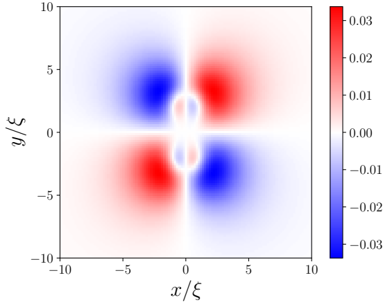
FIG. 7. Axial mass current of the D-core vortex at p = 20 bar and T = 0.55 T_c . The current density is scaled in units of j_c .
