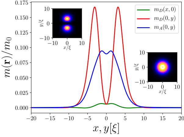
FIG. 8. Magnetization profiles, m_A and m_D , for the A- and D-core vortices, respectively. Insets: density plots of the same. For the A-core phase: p = 34 bar T = 0.75 T_c = 1.86 mK. For the D-core phase: p = 20 bar T = 0.55 T_c = 1.23 mK.
