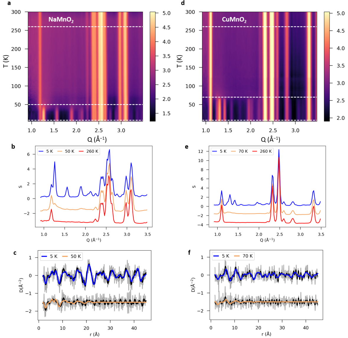
FIG. 3. Magnetic scattering and magnetic PDF analysis of CuMnO 2 and NaMnO 2 . (a) Color map of the scattered intensity S(Q) of NaMnO 2 with temperature on the vertical axis and Q on the horizontal axis. (b) S(Q) for NaMnO 2 at 5 K (blue curve), 50 K (orange curve), and 260 K (red curve), indicated by horizontal dashed lines in panel (a). (c) Corresponding mPDF data for NaMnO 2 at 5 K and 50 K. The 50 K data is offset along the y-axis by -1.5 \text{ \AA}^{-2} for clarity. The black curves and thin gray curves represent the Fourier filtered and unfiltered data, respectively. The blue and orange curves represent the mPDF fits for 5 and 50 K, respectively. (d-f) Equivalent results for CuMnO 2 . The intensity scale for (d) was chosen such that the strongest magnetic Bragg peaks for CMO and NMO have equal contrast. The magnetic model in Ref. 11 was used for the fits in (f).
