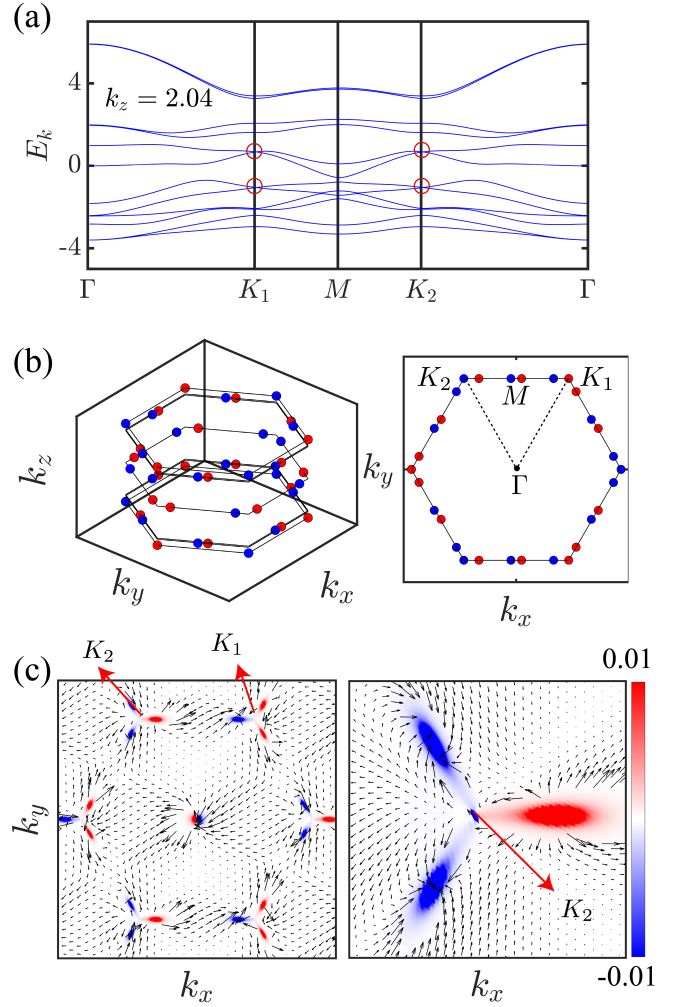
FIG. 8. (a): Band structure along symmetric paths of the BZ. Red circles indicate Weyl points. (b) Weyl points in the first BZ. Red circles correspond to Q > 0 , while blue circles correspond to Q < 0 . (c) Left: vector field \mathcal{B}^{(5)} associated with the fifth band on the q_z = 0^+ plane (taken as q_z = 10^{-4} in numerical calculation). Right: enlarged plot around the K_2 point. The model parameters are: t' = t , J = 2t , \alpha = 0.2\pi , \alpha' = 0.2\pi , and \theta' = \pi/4 \approx 0.785 .
