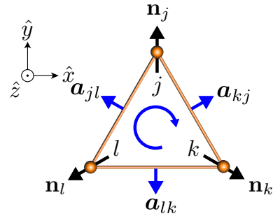
FIG. 2. Coplanar configuration with Berry phase different from 0 or \pi . The clockwise circulation indicates the bond orientations required to define the directions of the spin-orbit vectors \mathbf{a}_{kj} , \mathbf{a}_{lk} , and \mathbf{a}_{jl} , indicated with blue arrows.
