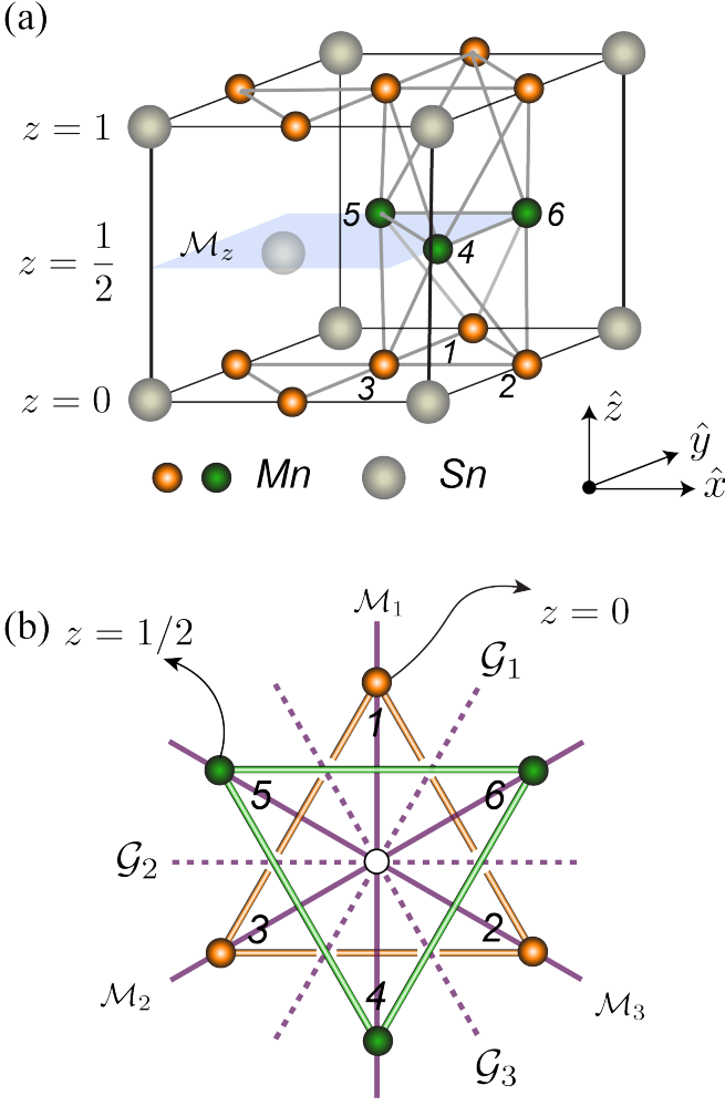
FIG. 6. (a) Crystallographic unit cell of Mn 3 Sn containing six Mn atoms (3 in the z = 0 plane and 3 in the 1/2 plane). \mathcal{M}_z with z = 1/2 is a mirror symmetry plane. (b) Vertical mirror planes \mathcal{M}_i and glide planes \mathcal{G}_i ( i = 1, 2, 3 ). The white circle at z = 1/4 indicates an inversion center.
