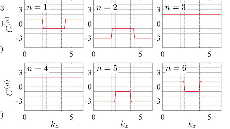
FIG. 5. Chern number C(k_z) for each (k_x, k_y) plane in momentum space. The in-plane parameters are the same as in Fig. 4, while the inter-layer hopping amplitudes are t_z^1 = 0.1t and t_z^2 = 0.3t .
