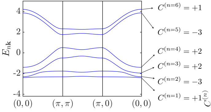
FIG. 4. Band structure of the tight-binding model of Eq. (77) for Hamiltonian parameters J = 0.5t , \alpha = 0.2\pi , \theta = 0 .
