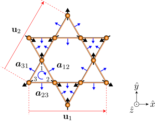
FIG. 3. Uniform 120^\circ magnetic ordering (black arrows) on the Kagome lattice. This is a straightforward extension of the single triangle state shown in Figure 2. The clockwise circulation indicates the bond orientation. The in-plane components of the SOC vectors \mathbf{a}_{12}^\perp , \mathbf{a}_{23}^\perp , \mathbf{a}_{31}^\perp are indicated with blue arrows. \mathbf{u}_{1,2} are the primitive lattice vectors of the Bravais lattice.
