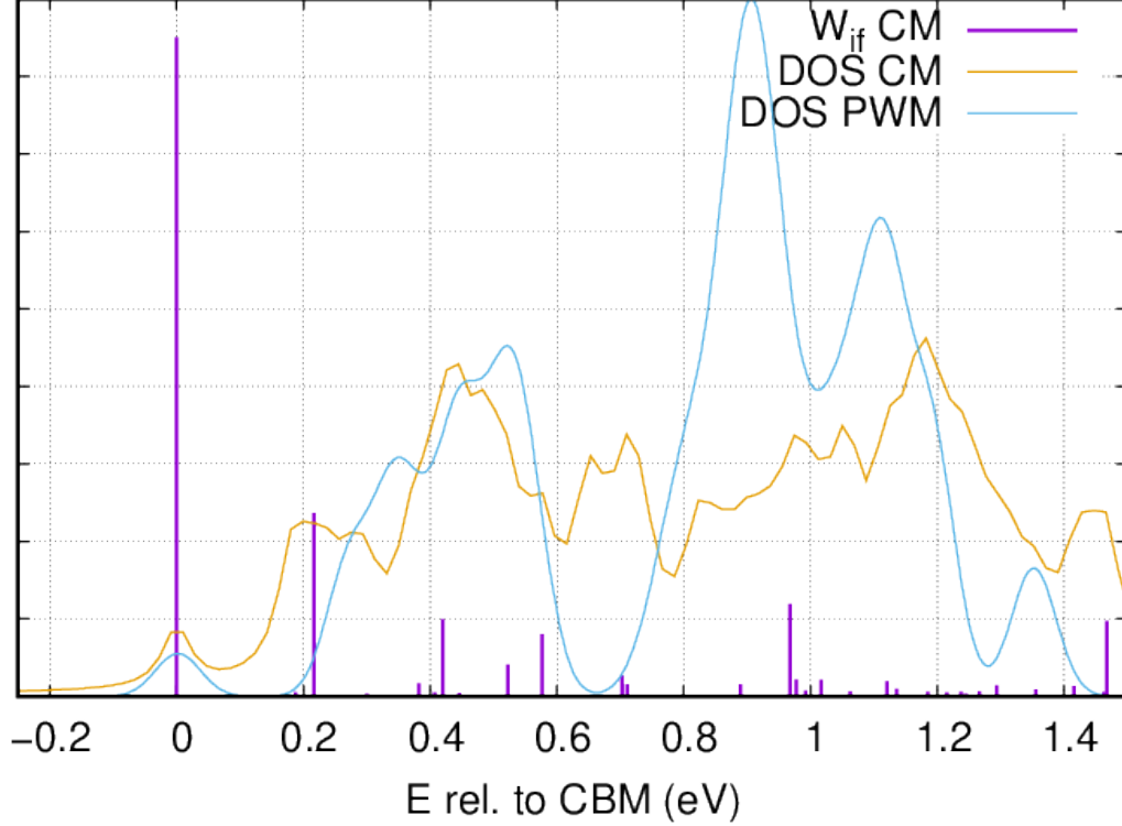
Figure 5. Electron-phonon matrix elements and density of states from CM calculations and density of states from PWM calculations near the conduction band minimum.
