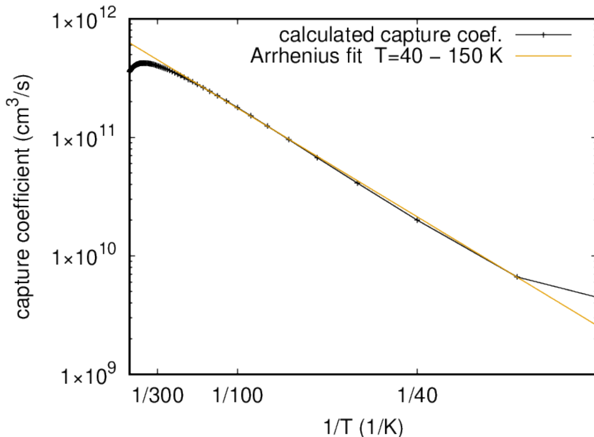
Figure 7. Arrhenius fit (yellow line) to calculated capture coefficient (decorated black curve – same data as the solid purple curve in Figure 6).
