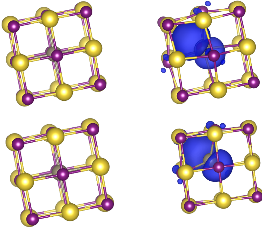
Figure 2. Calculated local environment of a Tl dopant in NaI using the PBE0 1/3 exchange-correlation approximation in plane-wave (top row) and cluster (bottom row) models without (left column) and with (right column) a trapped electron. The spin density isosurfaces (at 0.001 electrons per cubic angstrom) associated with the trapped electron is plotted in blue. Na atoms are shown in gold, I atoms in purple, and the Tl dopant is grey.
