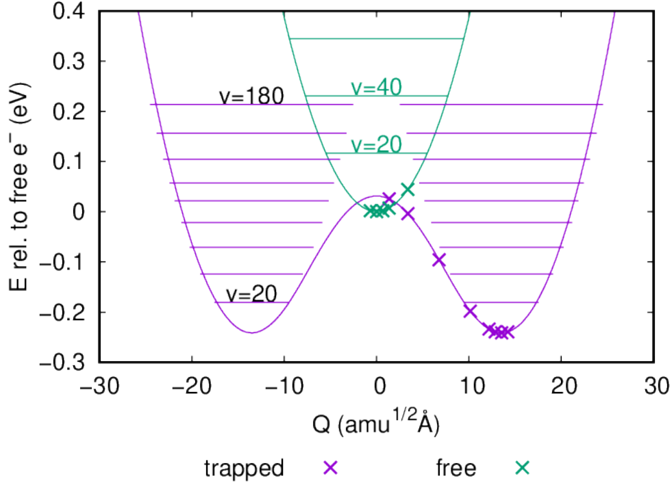
Figure 4. Final configuration-coordinate diagram used for calculation of the vibrational structure. The x's mark explicitly calculated points (and agree with the green x's in Figure 3), the curved solid lines are the interpolated/extrapolated adiabatic potential energy surfaces, and the horizontal solid lines mark every 20 th vibrational level (excluding the v = 0 levels for clarity), drawn between the classical turning points in the harmonic approximation.
