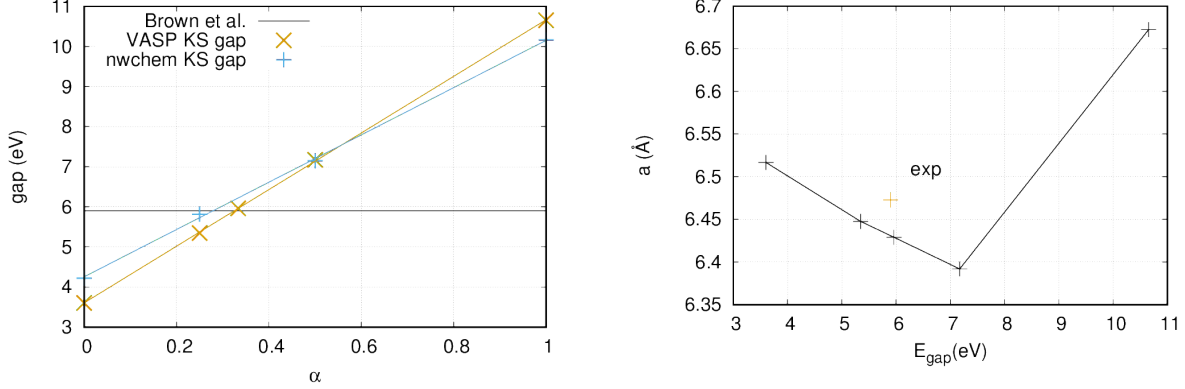
Figure 1. Left: Band gap vs. the fraction of explicit exchange included in the xc functional in our CM (blue) and PWM (yellow) calculations. Right: computed lattice constant a vs. band gap for the PWM calculations. The experimental band gap is taken from Ref. [79] while the lattice constant is from Ref. [79,80]. The functionals are otherwise standard PBE for the remainder of the exchange functional and the correlation functional, except for the case \alpha = 1 , which is Hartree-Fock (HF) theory (i.e. no correlation).
