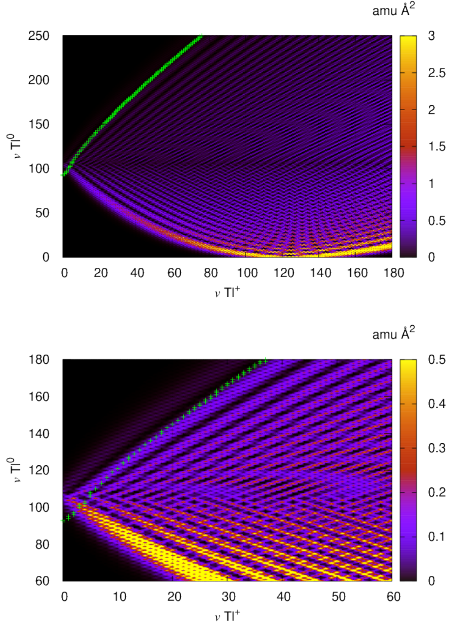
Figure 8. Heat map of the squared matrix elements |\langle I|Q|F\rangle|^2 between different vibrational states of the upper (horizontal axis) and lower (vertical axis) PES's. The green '+'s mark transitions that are allowed by energy conservation. Since none of the plotted quantities involve the thermal occupation factors, this figure describes both trapping and detrapping probabilities.
