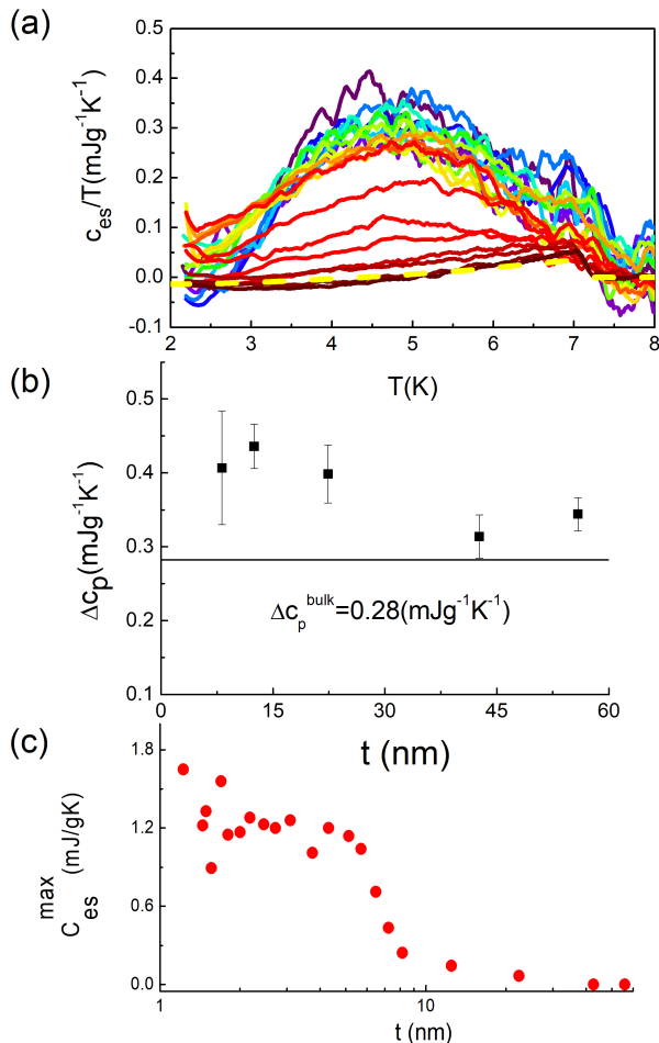
FIG. 4: (a) Specific heat of electrons in the superconducting state c_{es} normalized to temperature versus T . The squares mark the T_{Cres} of each layer extracted from the RT curves of Fig. 2(a). The yellow dashed line is a fit to BCS expectation. (b) The amplitude of the specific heat jump at T_C , \Delta c_p , as a function of thickness. (c) The maximum value of the specific heat, normalized to the specific heat of layer 22, as a function of thickness.
