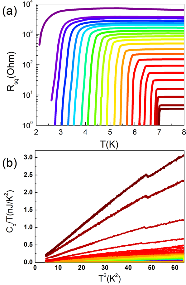
FIG. 2: (a) Resistance per square R_{sq} versus temperature for the 22 sequential quench condensed lead films. Purple is for thin films and red-brown for thick films. This color code is maintained throughout the paper. (b) Heat capacity of the films (same color code) in form of C_p/T versus T^2 highlighting the cubic behavior above 7.2 K.
