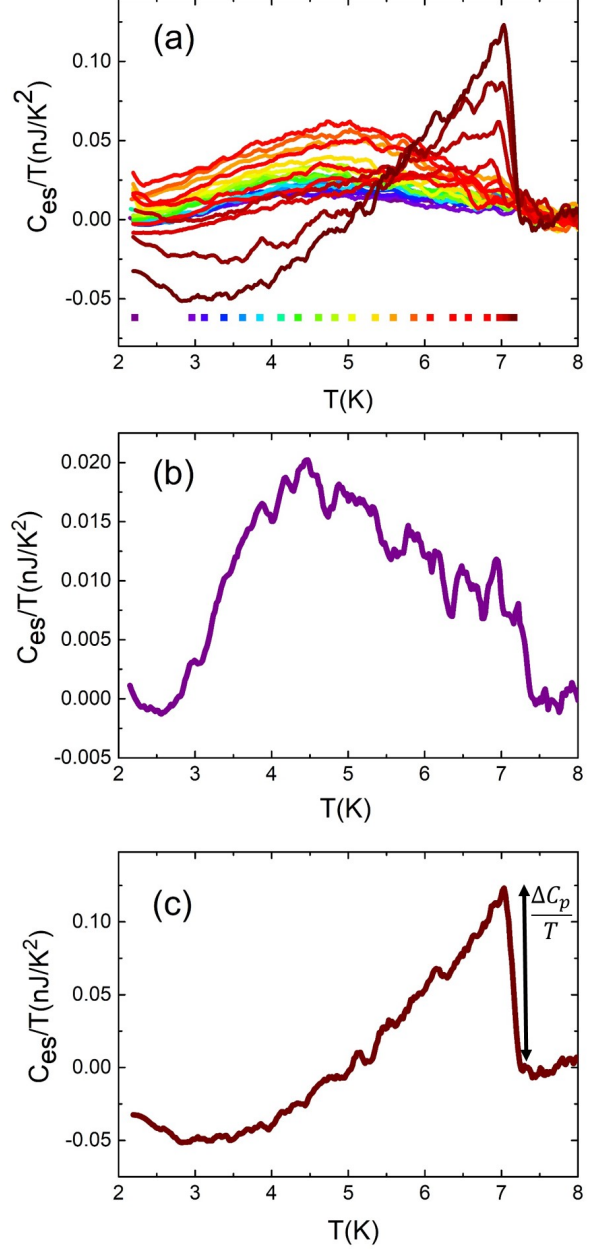
FIG. 3: (a) Superconducting electronic heat capacity C_{es} of the films normalized to temperature as extracted from the data presented in Fig. 2 along with an identical color code. The squares mark the T_{C_{res}} of each layer extracted from the RT curves of Fig. 2(a). The curves for the 1.2 nm and 55 nm thick films are shown in (b) and (c) respectively. In (c), the arrow represents the heat capacity jump normalized to temperature.
