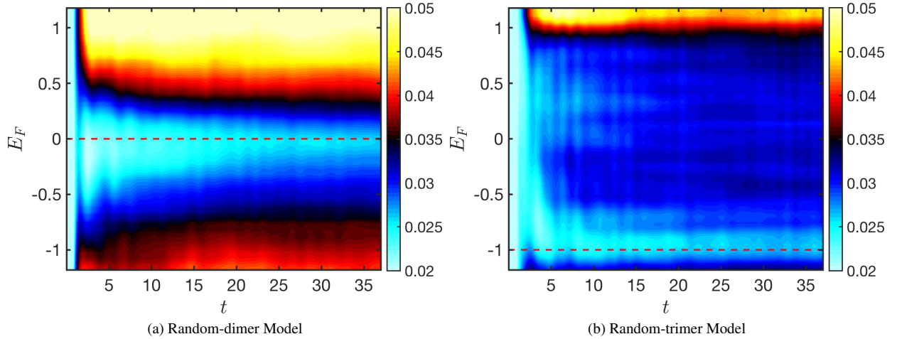
FIG. 1. (color online) EE between left- and right-movers (divided by N ) for a single disorder configuration of the random-dimer model (a) and the random-trimer model (b) as a function of t and doping level of initial state. There is a clear suppression of entanglement for initial states with E_F near the resonant energies of these models (dashed red lines). Parameters: N = 702 and \epsilon_b = -3/4 .
