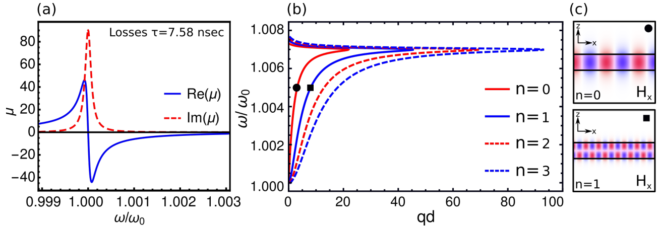
FIG. 2: Surface magnon polariton (SMP) modes on MnF 2 . (a) Frequency dependent permeability function for MnF 2 calculated using Equation 1 and using the parameters given in Table I. For MnF 2 , the resonance frequency is \omega_0 = 1.68 \times 10^{12} rad/s. For \omega_0 < \omega < \omega_{\max} , \text{Re}(\mu) < 0 , allowing for surface modes. (b) Dispersion relation for MnF 2 of thickness d , calculated in the quasi-magnetostatic limit which is valid in the range of thicknesses d we consider. The first four modes are shown. (c) Visualization of fundamental and first harmonic mode SMP through the field component H_x shown for a d = 200 nm film of MnF 2 at \omega/\omega_0 = 1.005 . The locations of these two modes are indicated on the dispersion curve.
