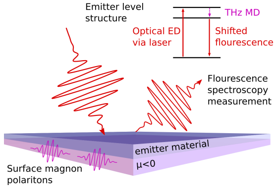
FIG. 8: Schematic for a potential fluorescence spectroscopy experiment to observe enhancement of magnetic dipole (MD) transitions through surface magnon polaritons. We consider a layered sample which contains a thin negative permeability film which supports SMPs, and a material containing an appropriately chosen emitter material. An external laser prepares the emitters into an excited state via an IR/optical transition. This excited state then decays via a THz transition into SMPs in the thin film, and then relaxes via a photon transition into the far field. The far field signal can be measured with a spectrometer to detect the Raman-shift in the fluorescence frequency compared to the incident laser frequency.
