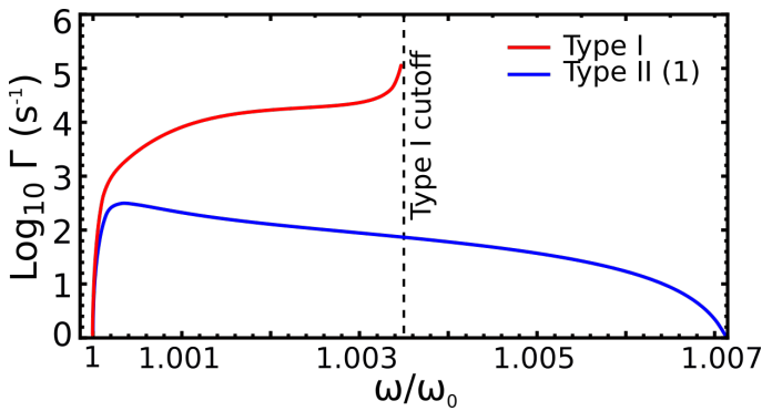
FIG. 7: Magnetic dipole transition rate for in-plane anisotropic \text{MnF}_2 . Magnetic dipole transition rate for a z -oriented dipole transition a distance z_0 = 5 nm from the surface into two different SMP modes in a d = 200 nm thick anisotropic slab of \text{MnF}_2 . The type I mode emits most strongly but over a narrower range of frequencies. The cutoff frequency is the frequency at which the first type I mode no longer satisfies the boundary conditions. The first order type II mode is emitted more weakly but is supported over the entire range of frequencies for which \mu(\omega) < 0 .
