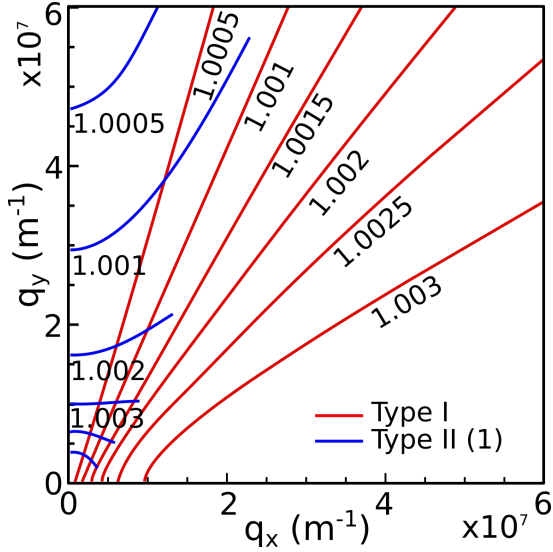
FIG. 5: Dispersion for anisotropic modes. Isofrequency contours for MnF 2 of thickness d = 200 nm. The frequency labels are given as \omega/\omega_0 , where \omega_0 is the resonance frequency of the material. The first type I modes are shown in red, while the type II modes with n = 1 are shown in blue.
