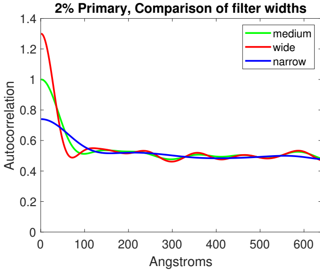
FIG. A3. Effect of varying the Fourier filter width around the CDW point when computing autocorrelation. “Medium” filter width is used in the main body of the paper.
