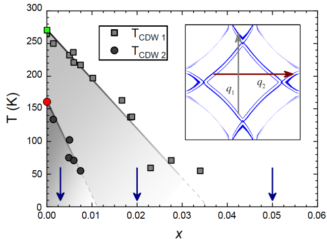
FIG. 1. Phase diagram taken from [13]. Colored points at x = 0 mark the phase transitions of the pristine sample. Grey points at finite x mark the crossover temperatures identified as features in the electrical resistivity. Vertical arrows mark the three Pd concentrations discussed in this manuscript. Inset: Calculated Fermi surface of the parent compound \text{ErTe}_3 (from [15]) with q_1 and q_2 as nesting vectors.
