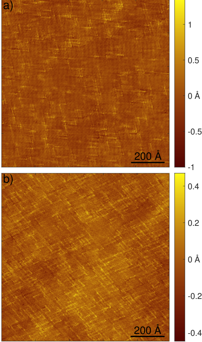
FIG. A1. 1000 Å topographic images for a) 0.3% Pd-intercalation sample and b) 2%.
