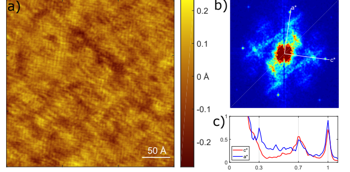
FIG. 4. a) 300Å Topography of 5% Pd-intercalation sample. b) FFT of (a) and c) the respective line cuts.
