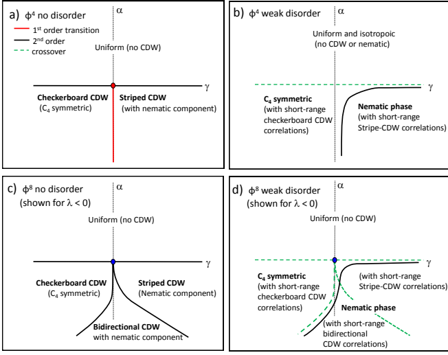
FIG. A4. Steps in constructing the phase diagram which is the result of the minimization of the different parts of the effective potential - see text.
