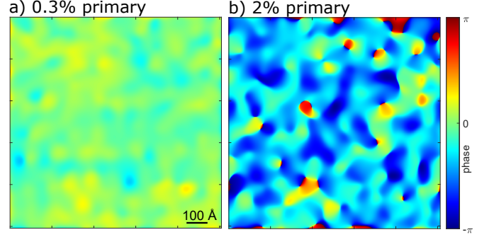
FIG. A2. 1000 Å phase plots for a) 0.3% Pd-intercalation sample and b) 2%.
