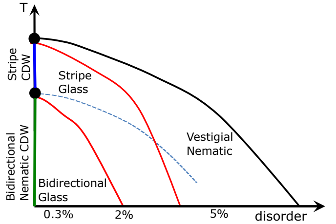
FIG. 5. A proposed phase diagram as derived in the Appendix.
