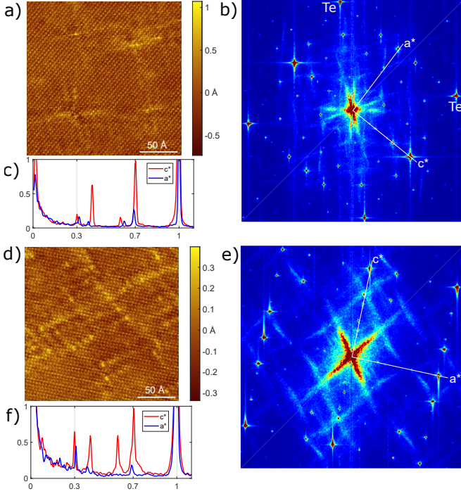
FIG. 2. a) Topography (cropped) of 0.3% Pd-intercalation sample. (Full size 100 nm image available in Appendix) b) FFT of (a) with reciprocal lattice points from the Te plane labeled and white lines indicating the line cut directions. c) The respective line cuts. Here the stronger CDW peaks (red) are along c^* . d) Topography (cropped) of 2% sample. e) FFT of (d) and f) the respective line cuts.
