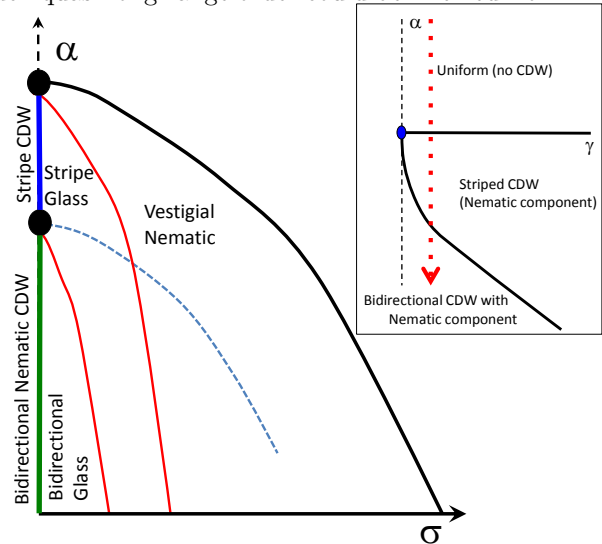
FIG. A5. A conjectured phase diagram as a function of temperature T and disorder strength \sigma . Here, the inset shows a portion of the clean limit phase diagram (plotted in the \alpha - \gamma plane, where \alpha should be considered a proxy for T ) - see text
