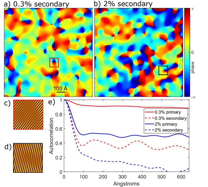
FIG. 3. CDW defect analysis of 0.3% and 2% Pd-intercalation samples. a) 1000 Å phase plot for the 0.3% secondary CDW showing dislocations. b) 2% sample c,d) Zoom in of the highlighted areas showing real-space filtered topography. e) Autocorrelation plots for the CDW signals.
