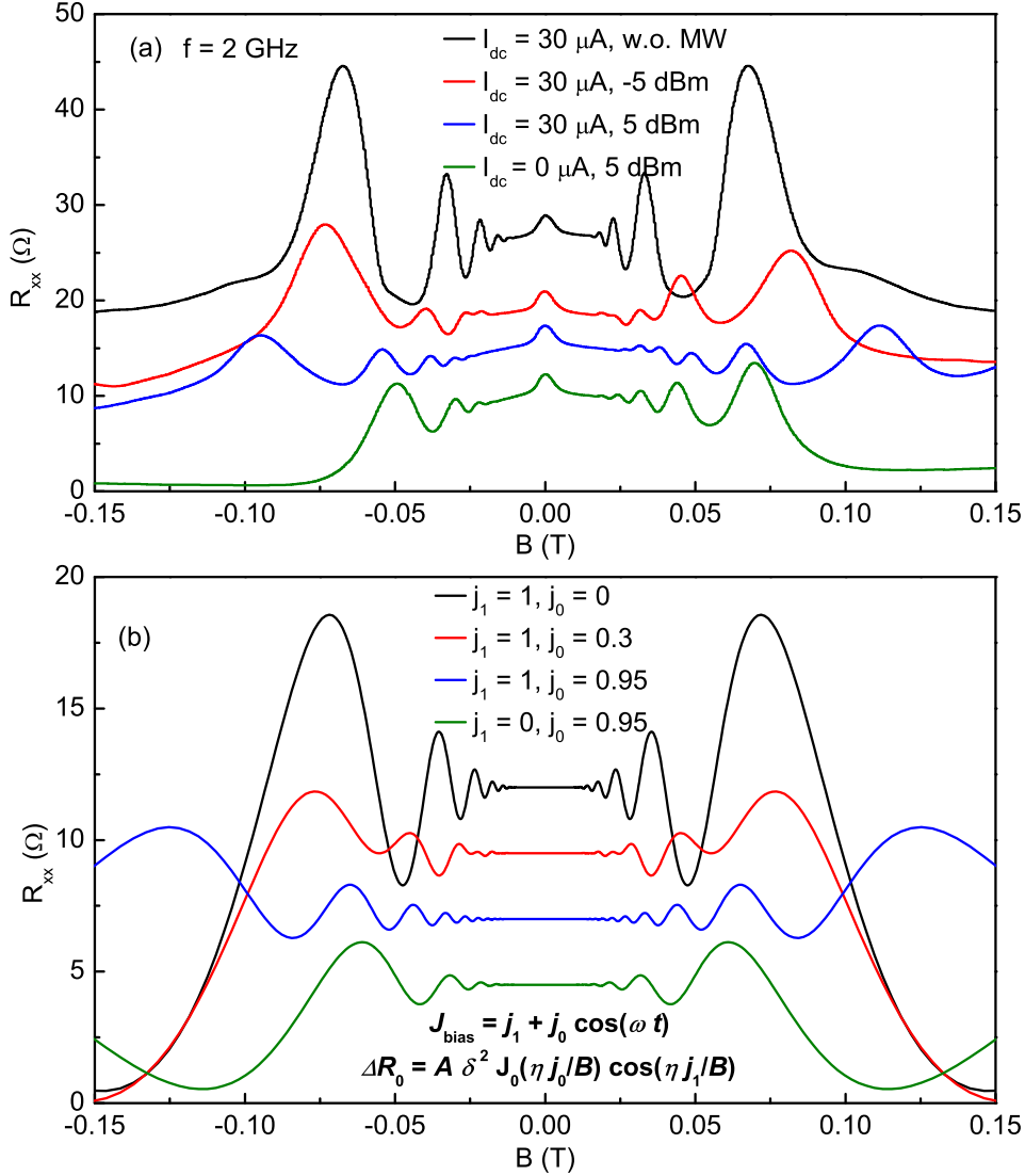
FIG. 4: (Color online). Panel (a): Magnetoresistance under MW irradiation for f = 2 GHz, with a dc-bias current passing through the Hall bar sample. The two kinds of oscillations merge into a new type of oscillation. (b): The traces of the formula \Delta R_0 = A \delta^2 J_0(\eta \frac{j_0}{B}) \cos(\eta \frac{j_1}{B}) are illustrated, where j_0 and j_1 are the relative amplitudes of the dc-bias and ac-bias current respectively. All the traces with vertical offset are shown for clarity.
