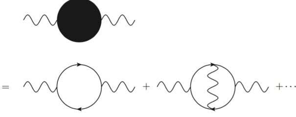
FIG. 1. In the present work, transport coefficients are defined as the IPI diagram in the first line. In the second line, the leading diagram on the left is given by RPA approximation, which can be isotropic. As higher order diagrams such as the right one in the second line are included, \langle aa \rangle would contribute to parity violating off diagonal terms at general e^2 , and invalidate the assumption of Drude values.
