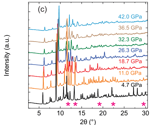
FIG. 1. (a) The \text{Ce}_3\text{Bi}_4\text{Pt}_3 unit cell, along with the fundamental Ce units (tetrahedrally coordinated to both Bi and Pt) that compose the larger structure. (b) Volume change with pressure of \text{Ce}_3\text{Bi}_4\text{Pt}_3 . The red line is a fit to the third-order Birch-Murnaghan equation of state [Eq. 1]. The 0 GPa volume was determined outside of a DAC. (c) Diffraction patterns (offset) for various pressures taken at room temperature. Cu peaks are marked with pink asterisks.
